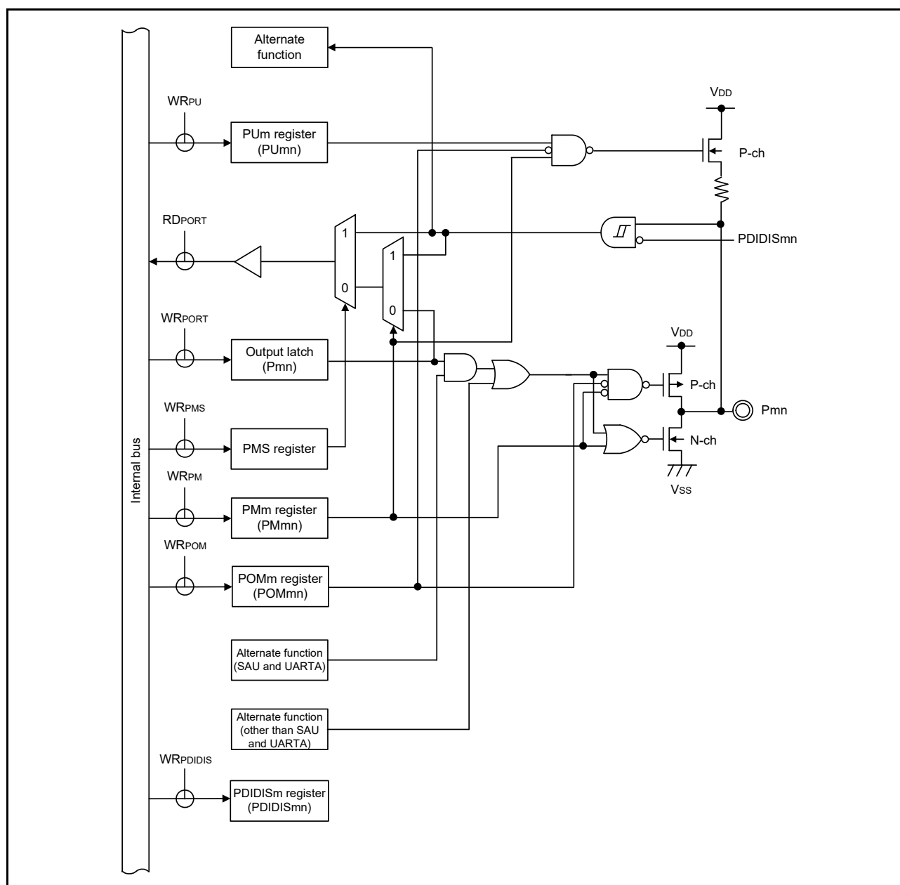
Figure 2 - 12 Pin Block Diagram for Pin Type 7-1-12
