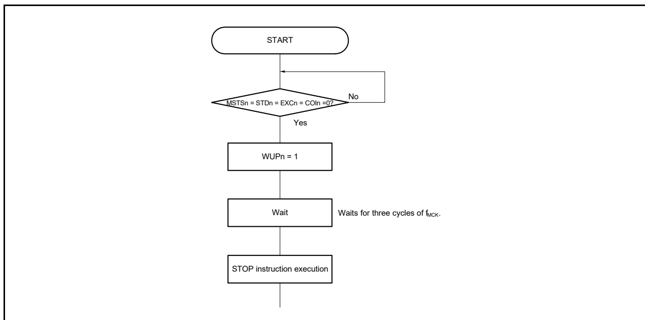
Figure 14 - 22 Flow When Setting WUPn = 1
