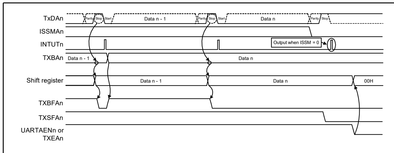
Figure 15 - 19 Timing Chart When Continuous Transmission Is Completed
