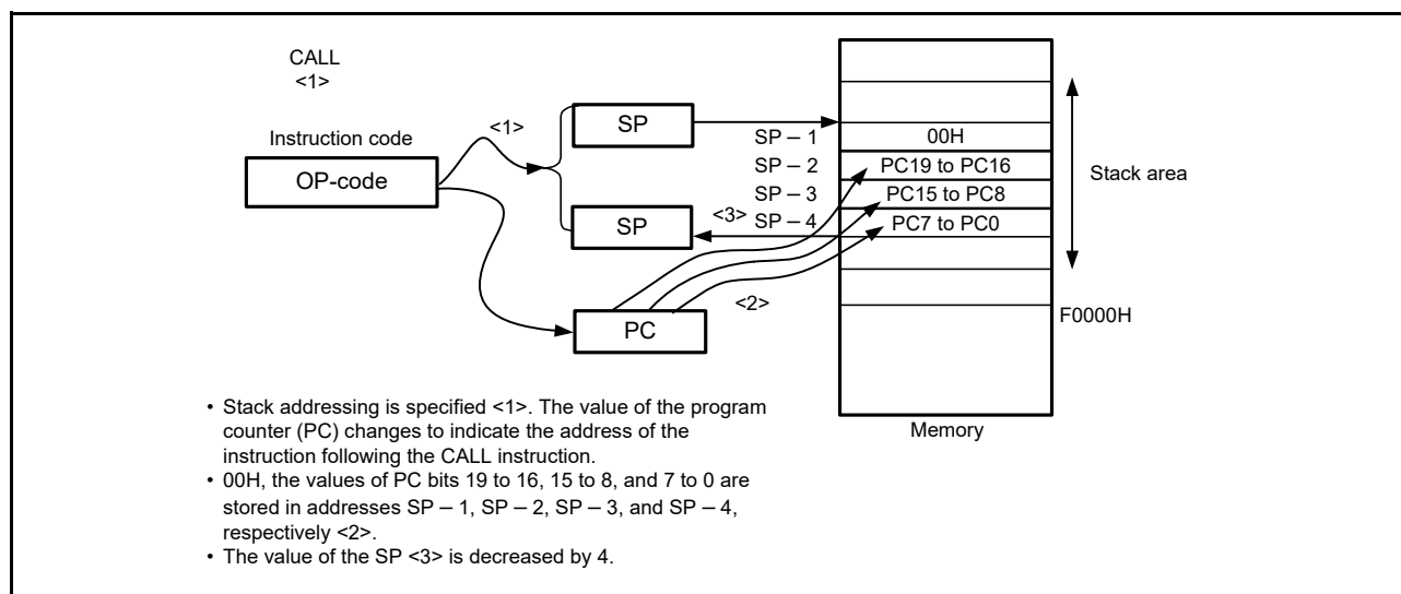
Figure 3 - 36 Example of CALL, CALLT
