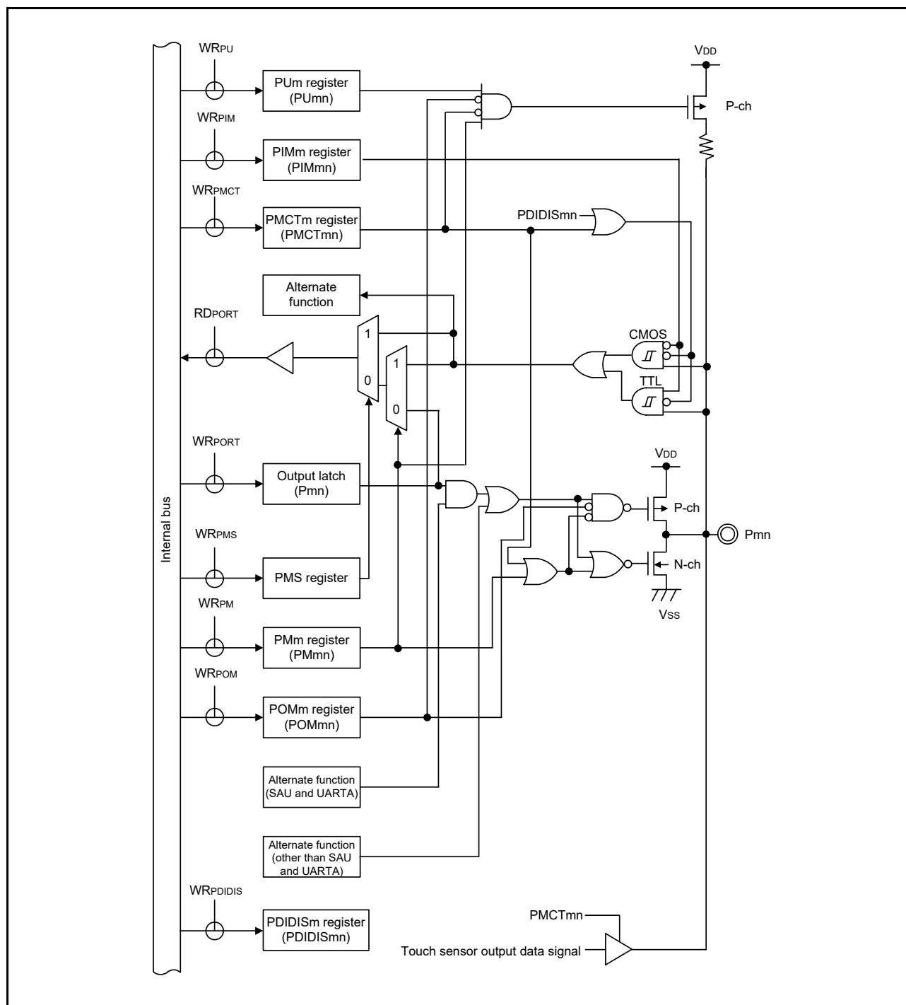
Figure 2 - 24 Pin Block Diagram for Pin Type 8-31-2
