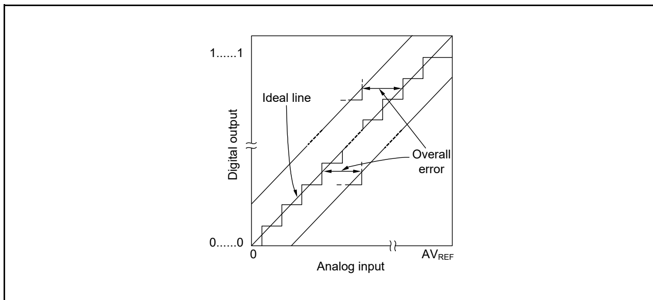
Figure 12 - 39 Overall Error
