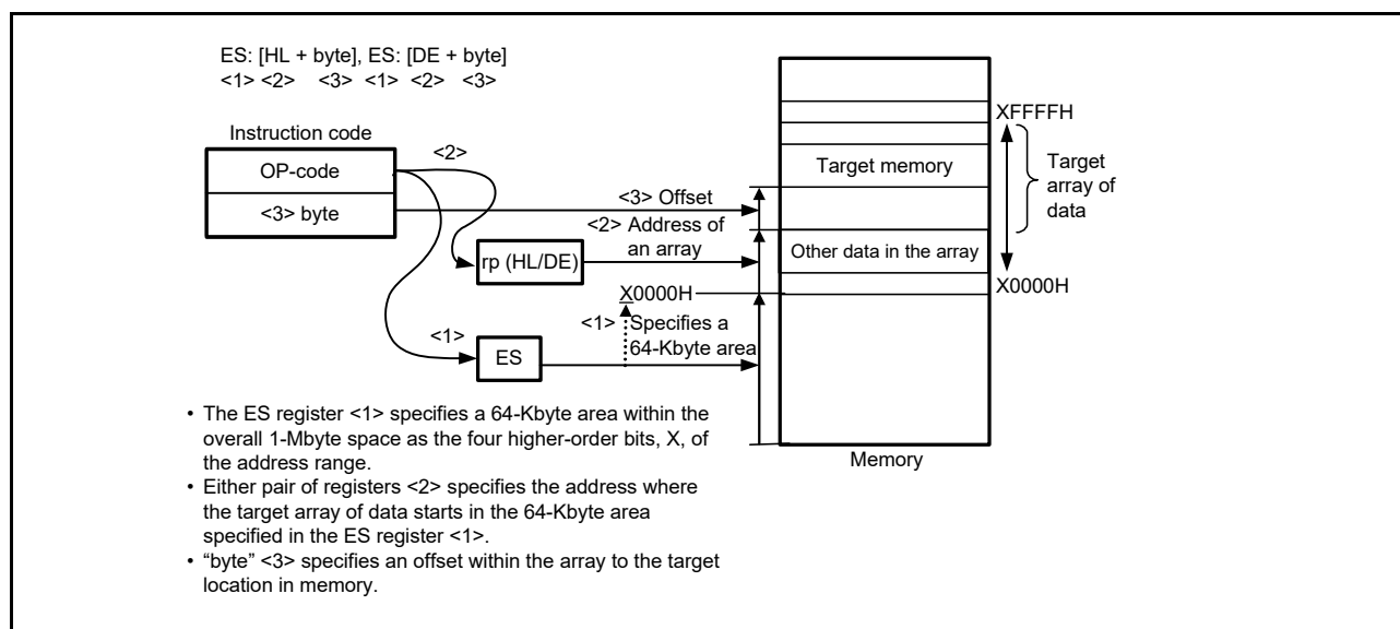
Figure 3 - 29 Example of ES:[HL + byte], ES:[DE + byte]
