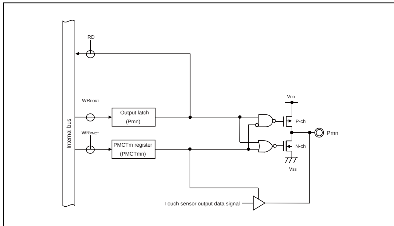
Figure 2 - 4 Pin Block Diagram for Pin Type 2-1-1
