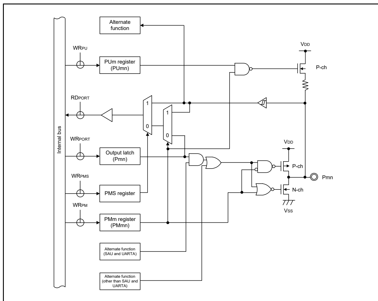
Figure 2 - 11 Pin Block Diagram for Pin Type 7-1-3
