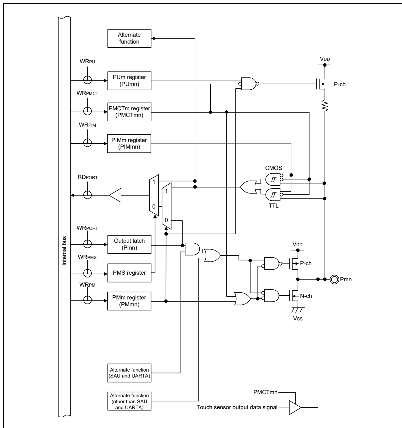
Figure 2 - 23 Pin Block Diagram for Pin Type 8-31-1
