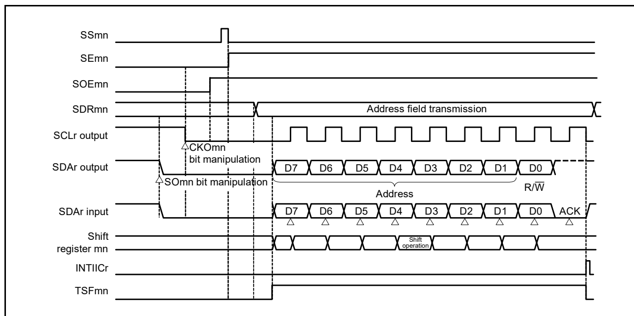
Figure 13 - 105 Timing Chart of Address Field Transmission
