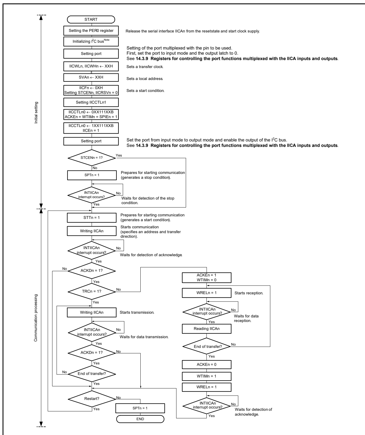
Figure 14 - 28 Master Operation in Single-Master System
