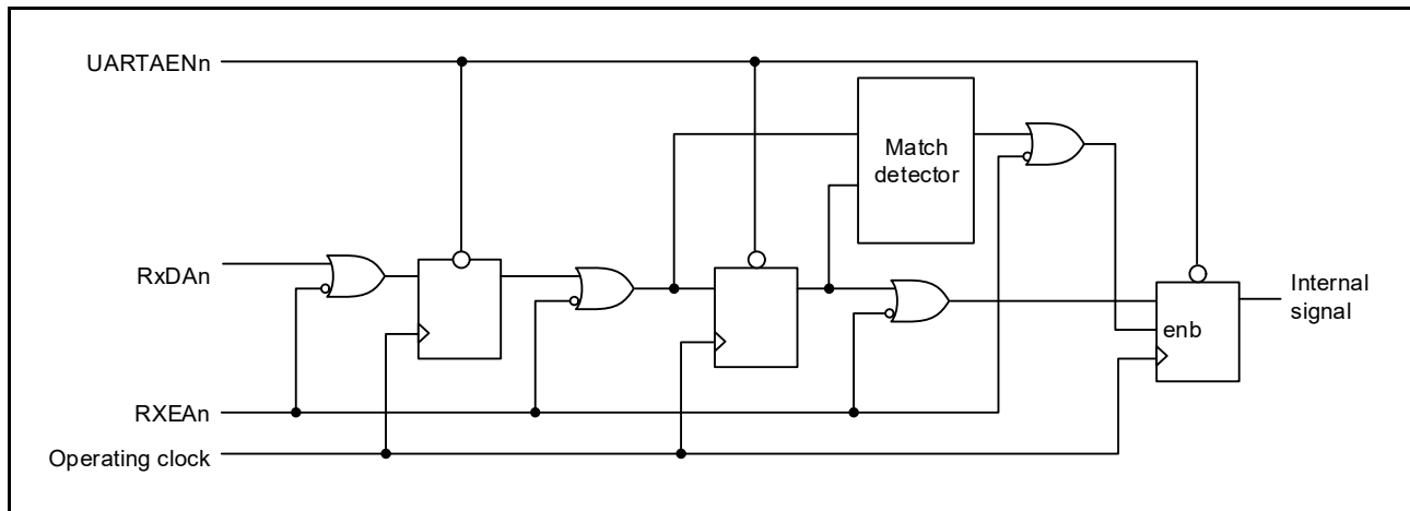
Figure 15 - 22 Noise Filter
