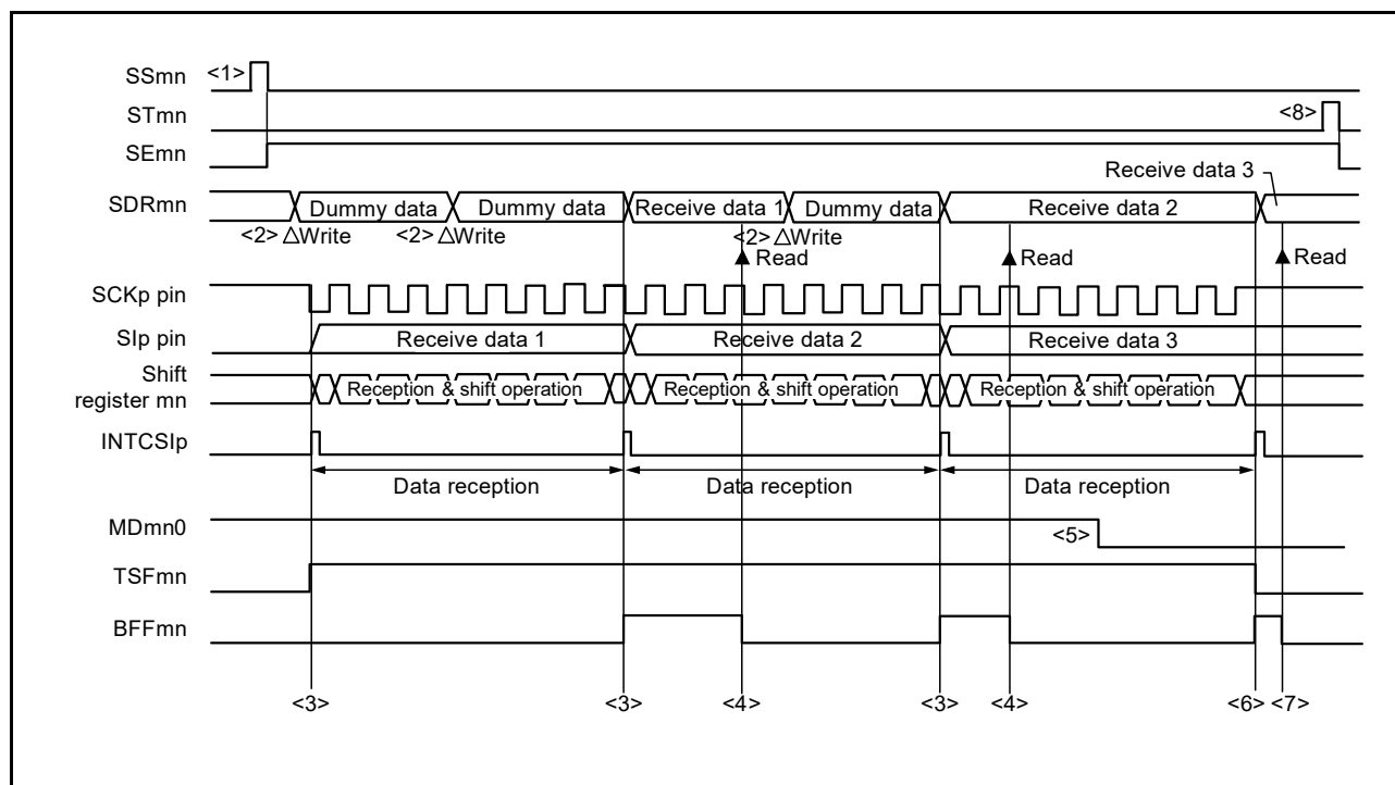
Figure 13 - 41 Timing Chart of Master Reception (in Continuous Reception Mode) (Type 1: DAPmn = 0, CKPmn = 0)
