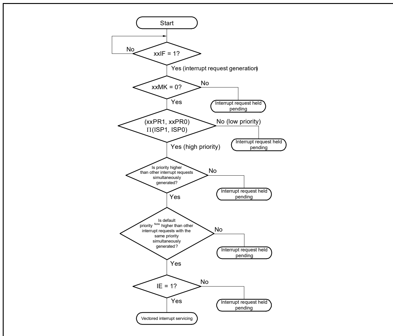
Figure 18 - 7 Interrupt Request Acknowledgment Processing Algorithm
