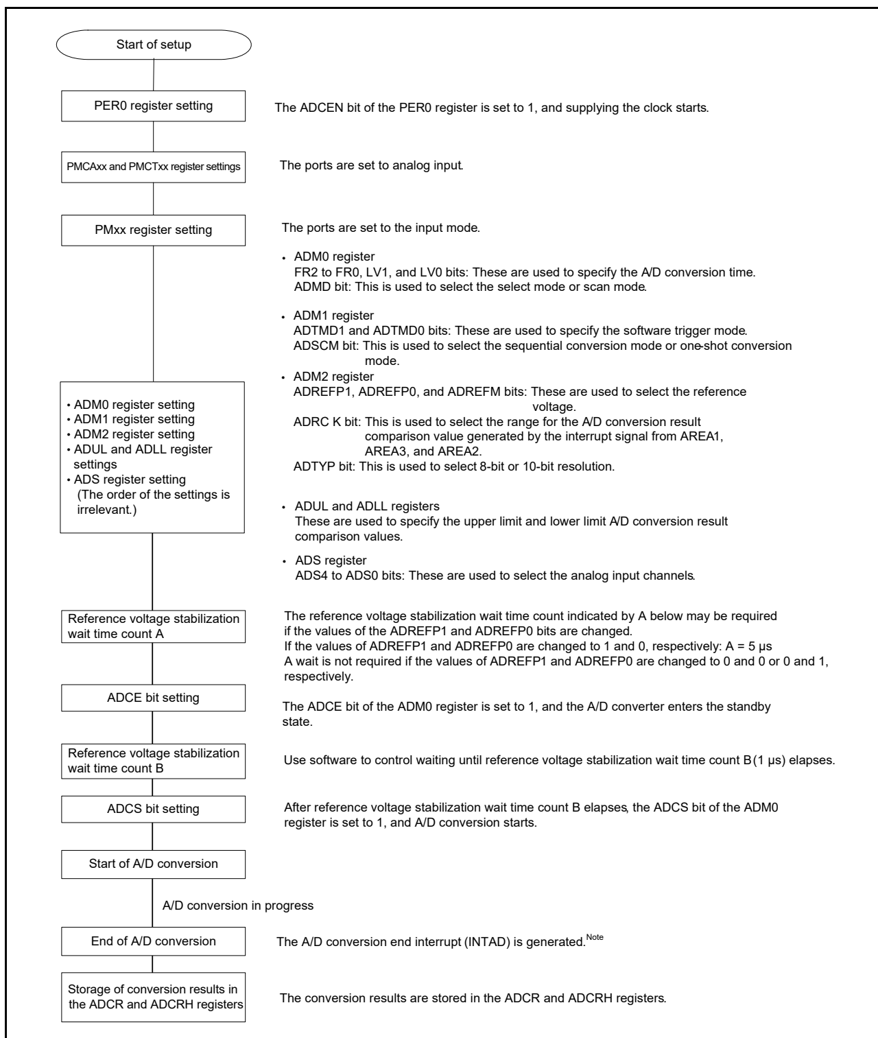
Figure 12 - 30 Setting up Software Trigger Mode
