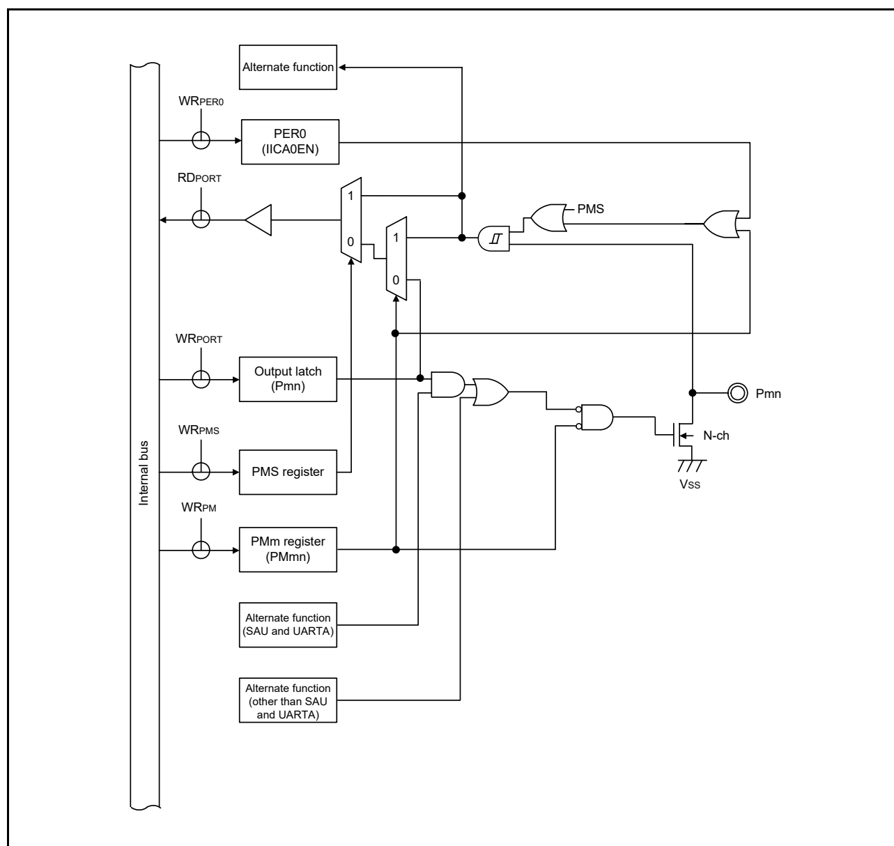
Figure 2 - 29 Pin Block Diagram for Pin Type 12-38-3
