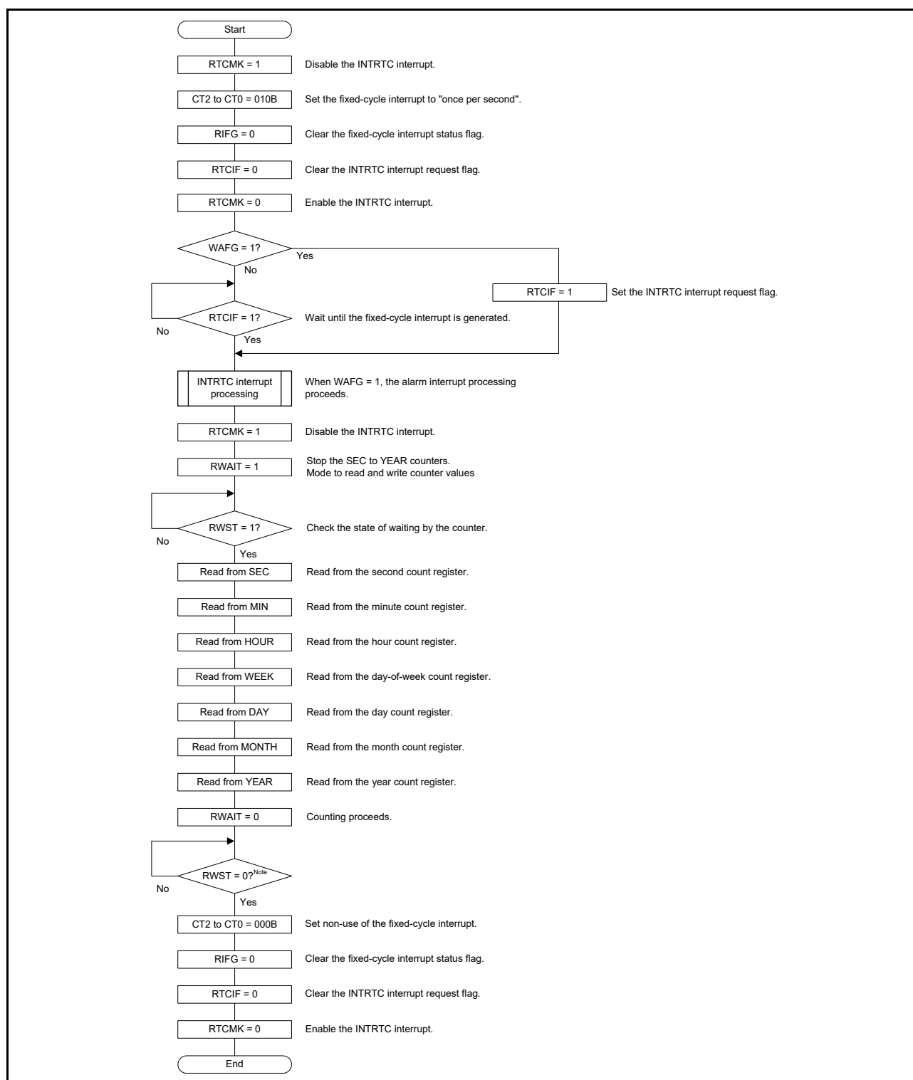
Figure 8 - 20 Procedure for Reading from the Realtime Clock (When the Alarm Interrupt is in Use)
