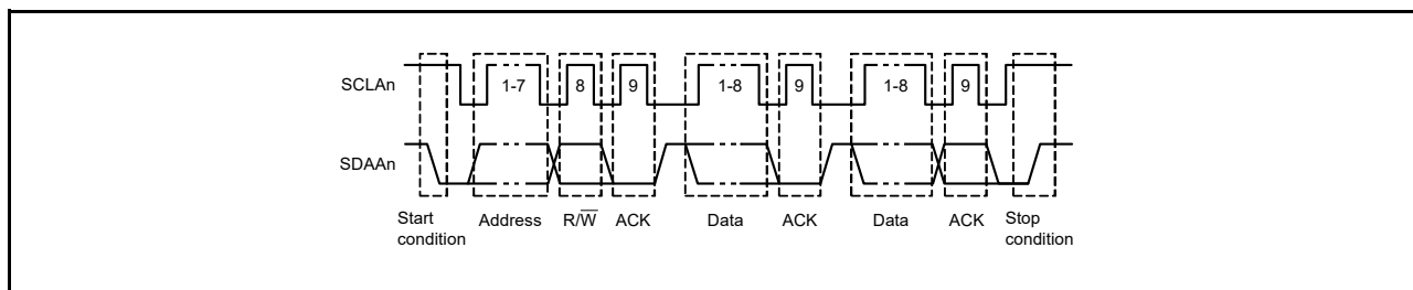
Figure 14 - 14 I 2 C Bus Serial Data Transfer Timing
