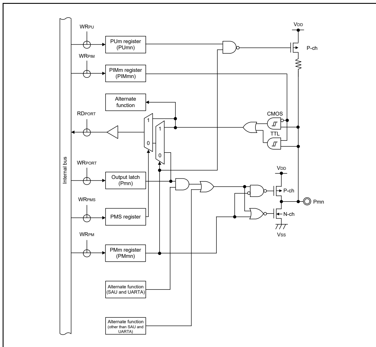
Figure 2 - 20 Pin Block Diagram for Pin Type 8-1-3
