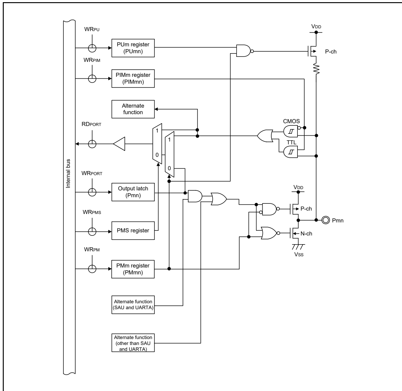
Figure 2 - 26 Pin Block Diagram for Pin Type 8-38-1
