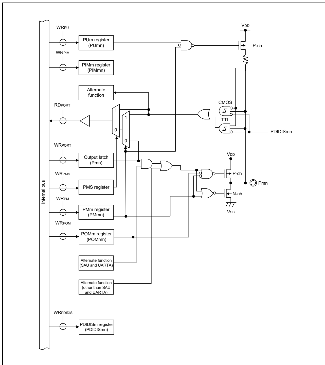
Figure 2 - 27 Pin Block Diagram for Pin Type 8-38-2
