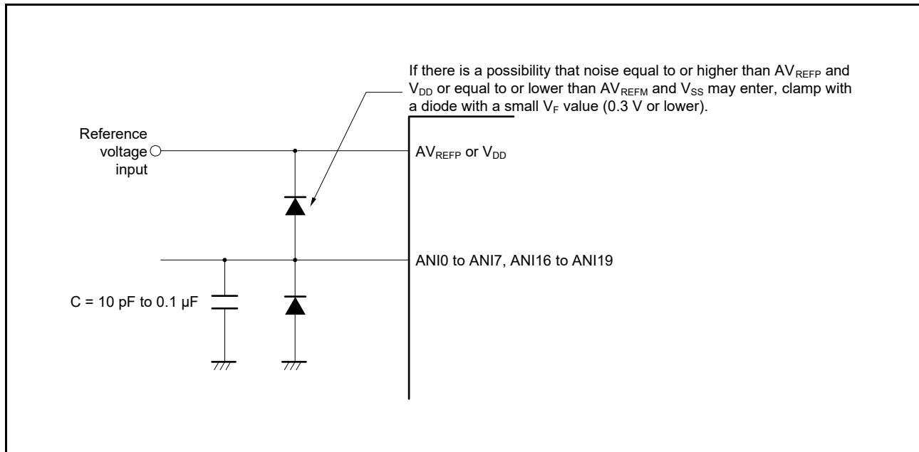
Figure 12 - 45 Analog Input Pin Connection
