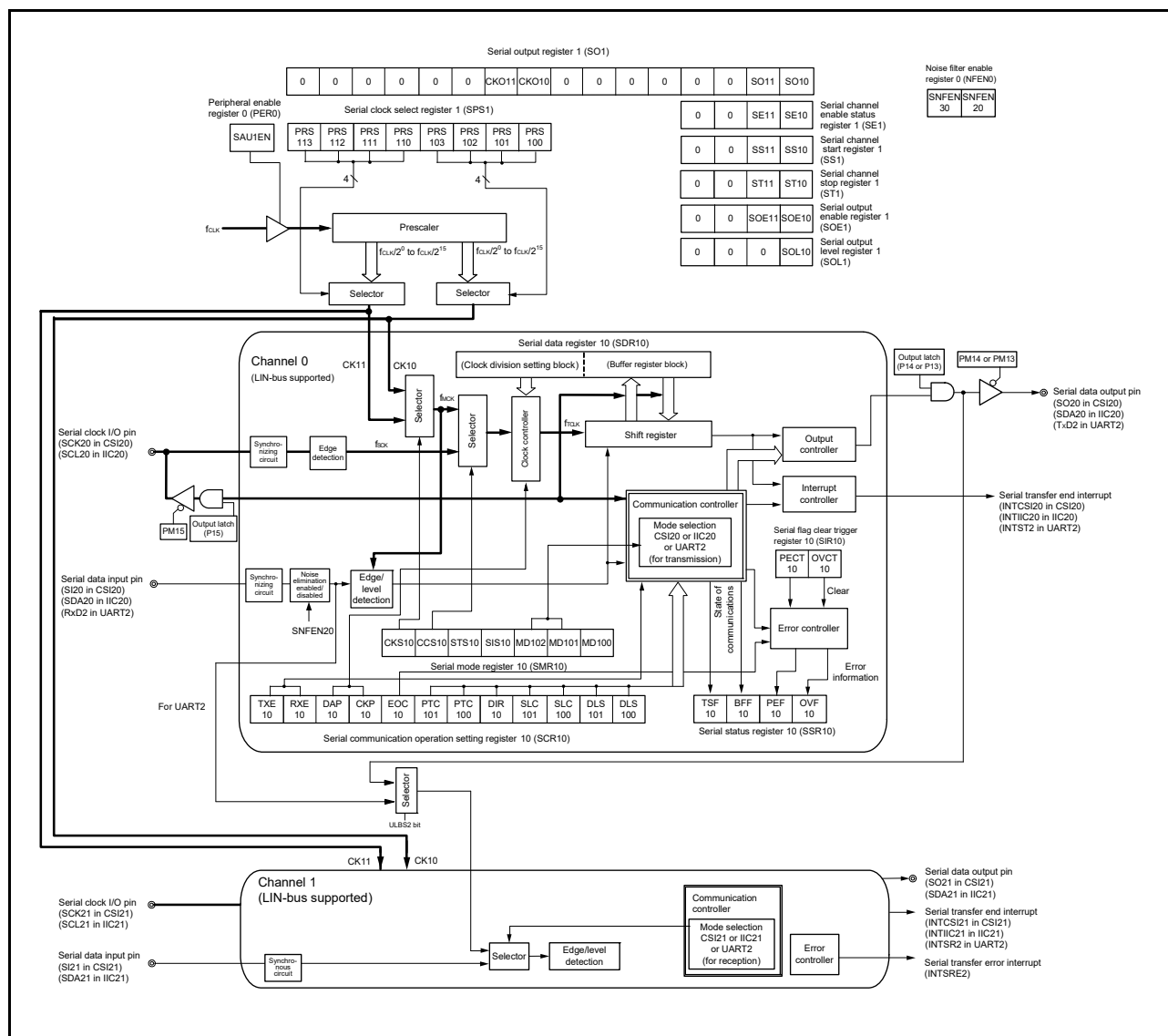
Figure 13 - 2 Block Diagram of Serial Array Unit 1
