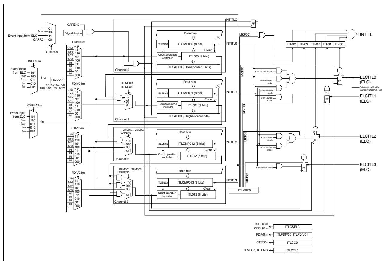
Figure 9 - 1 Block Diagram of 32-bit Interval Timer
