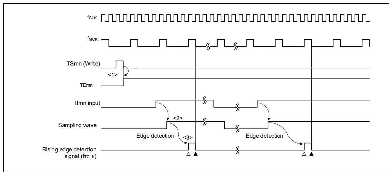
Figure 7 - 28 Timing of fCLK and Counter Clock (fCLK) (When CCSmn = 1, Noise Filter Not in Use)
