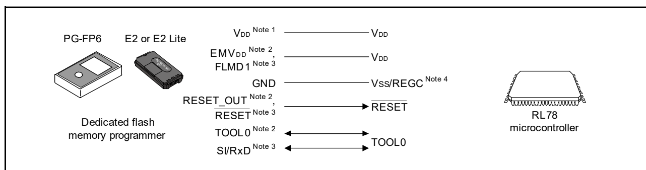
Figure 30 - 2 Communications with Dedicated Flash Memory Programmer
