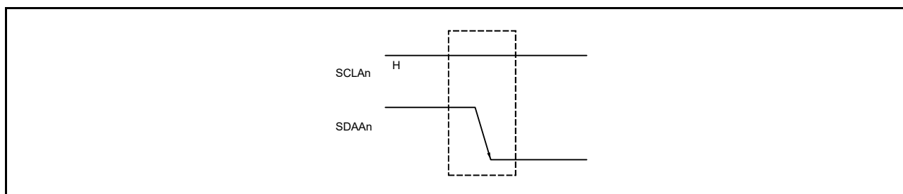
Figure 14 - 15 Start Conditions
