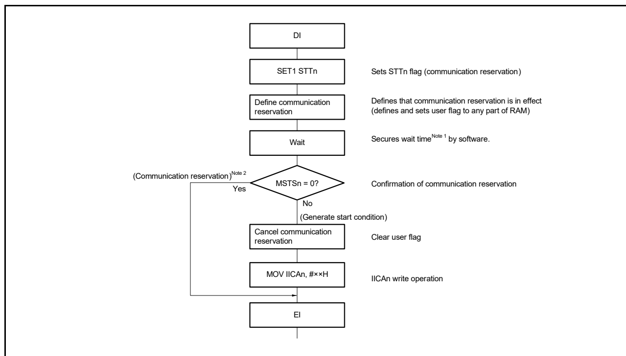
Figure 14 - 27 Communication Reservation Protocol
