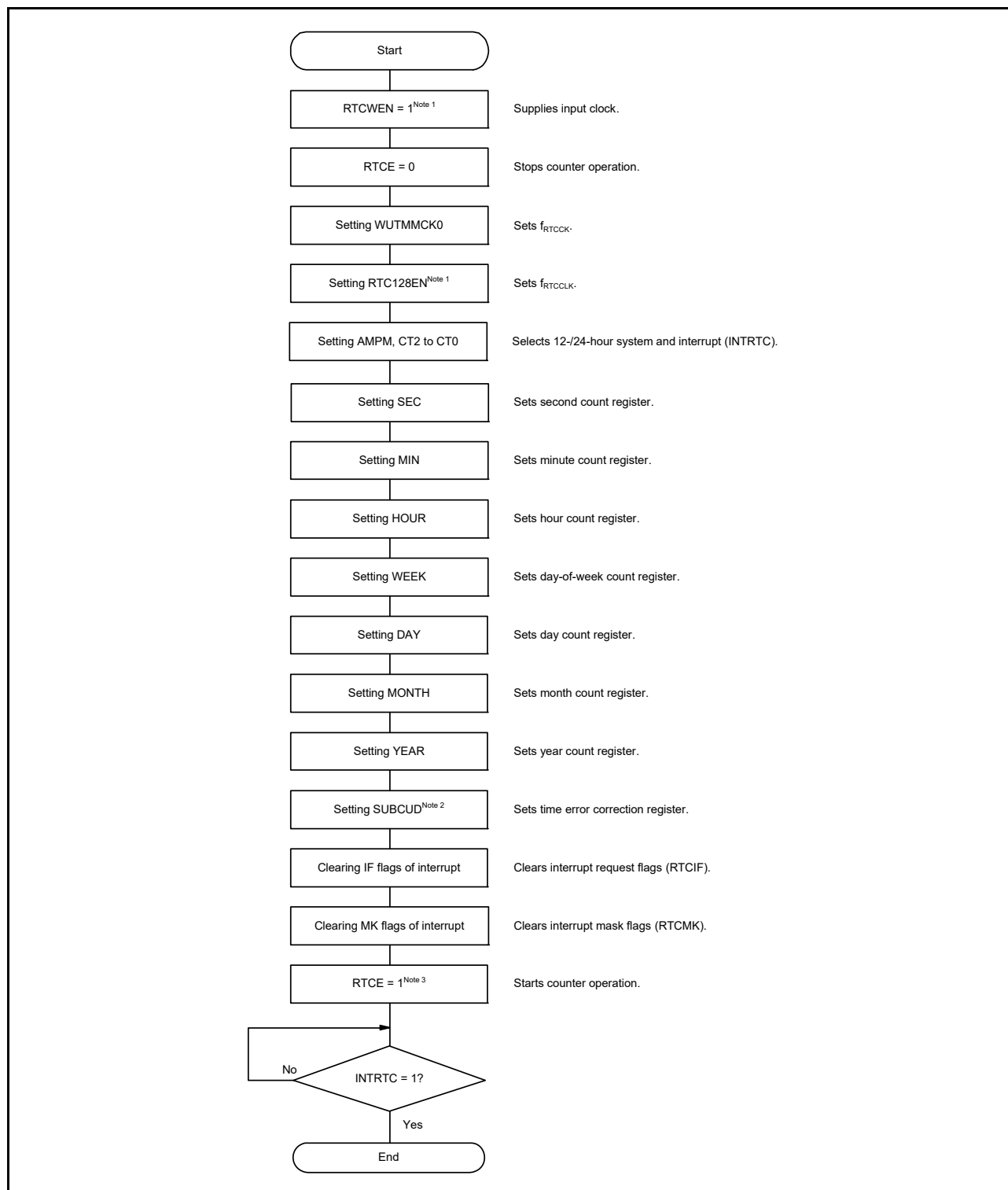
Figure 8 - 17 Procedure for Starting the Realtime Clock Operation
