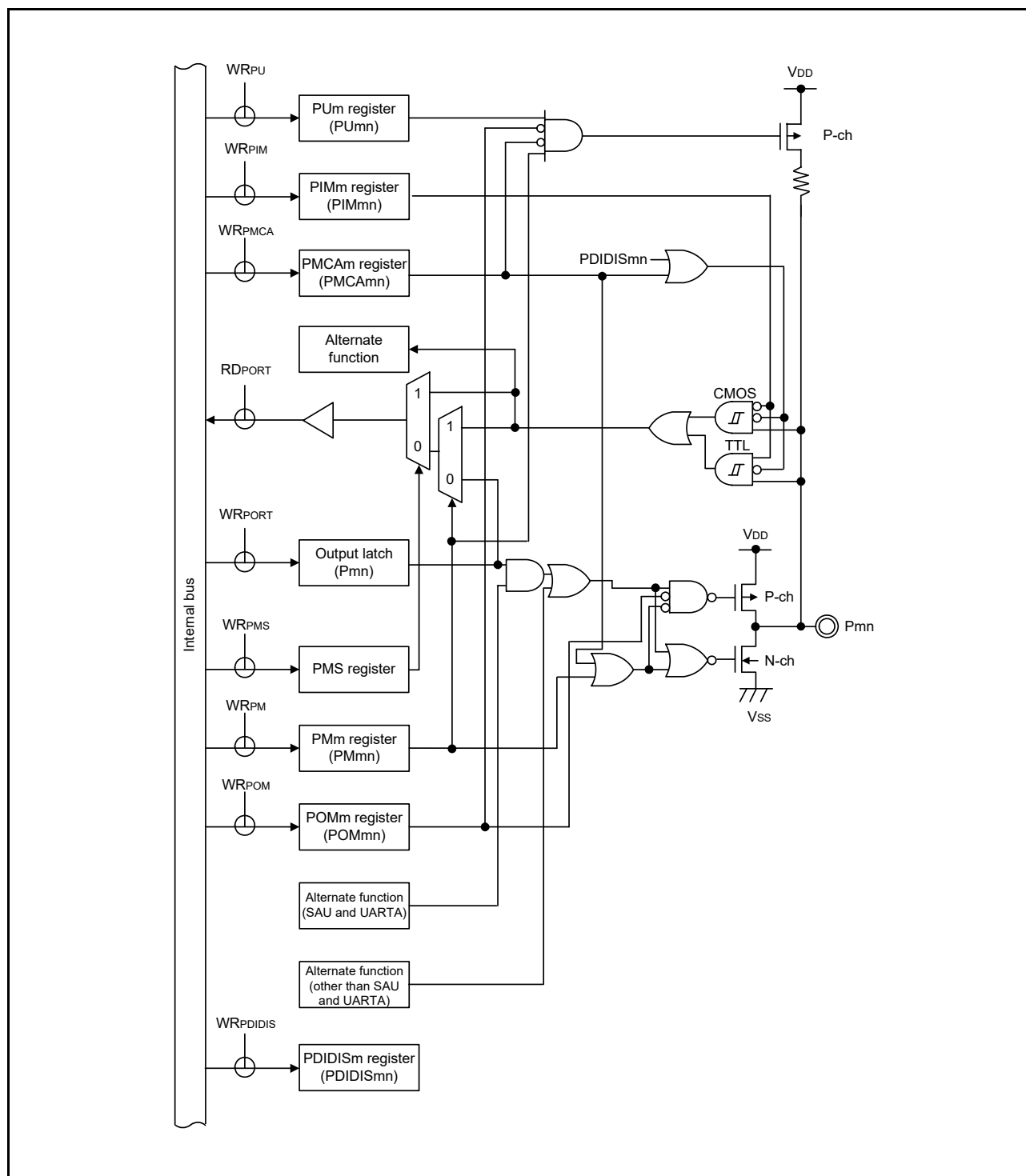
Figure 2 - 22 Pin Block Diagram for Pin Type 8-6-9
