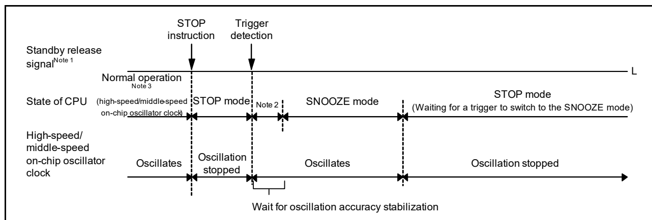
Figure 20 - 7 When the Interrupt Request Signal is Not Generated in the SNOOZE Mode
