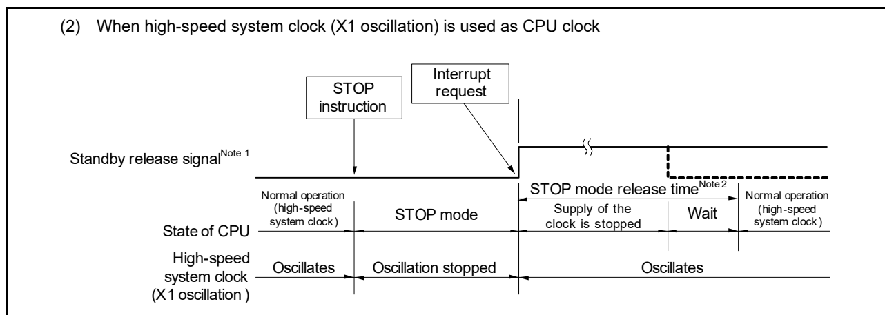
Figure 20 - 4 STOP Mode Release by Interrupt Request Generation (2/3)
