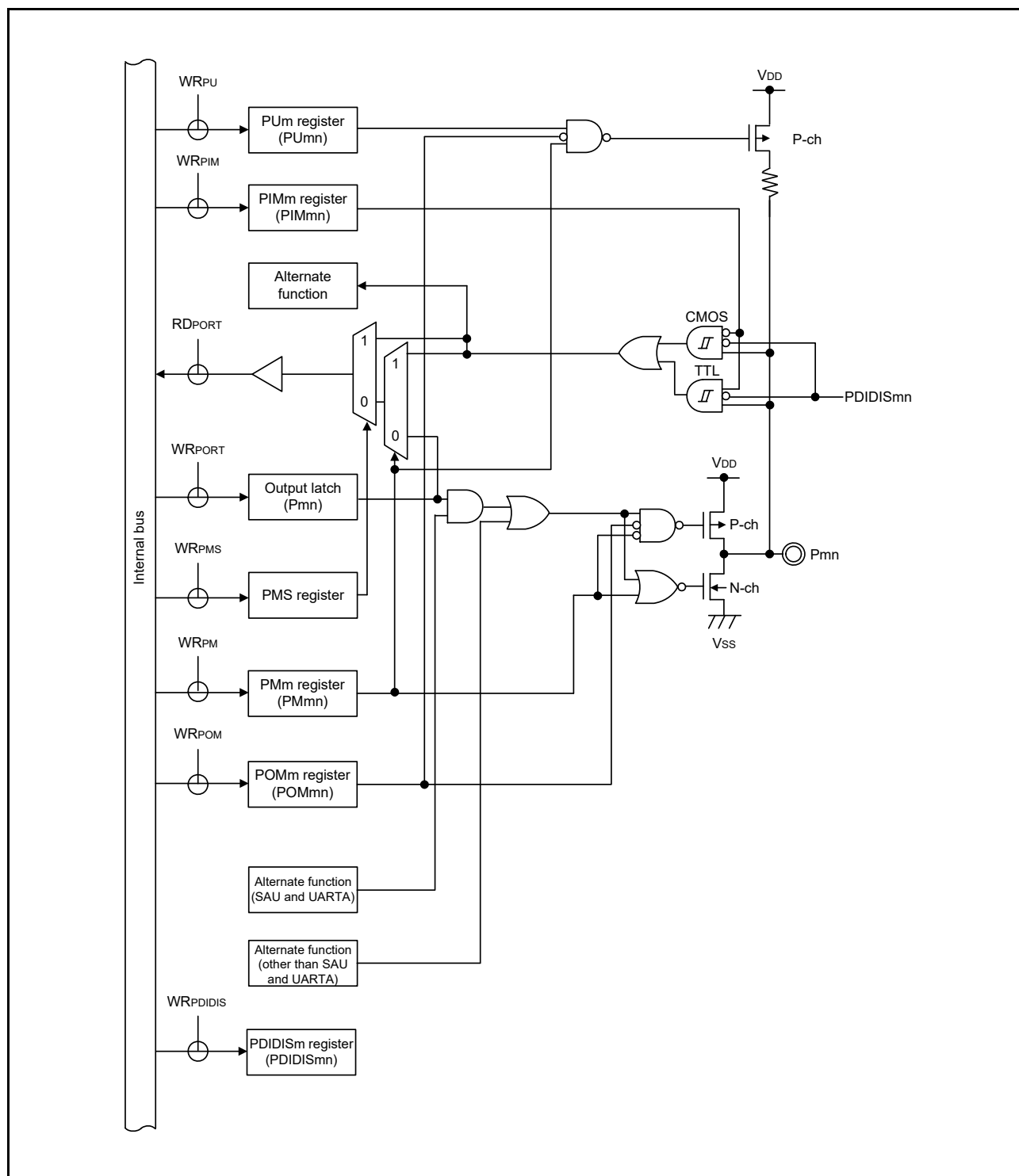
Figure 2 - 21 Pin Block Diagram for Pin Type 8-1-11
