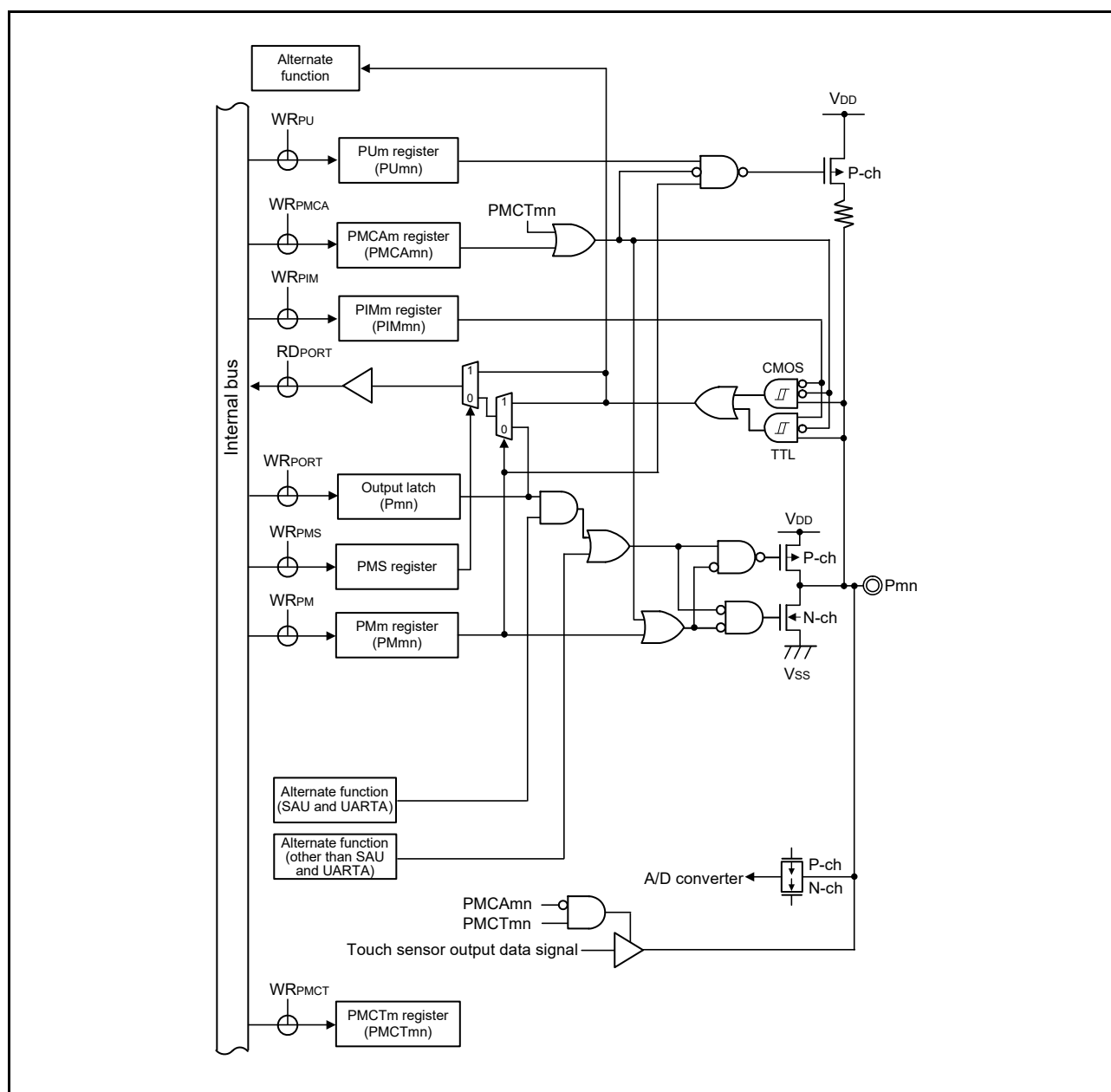
Figure 2 - 25 Pin Block Diagram for Pin Type 8-33-2
