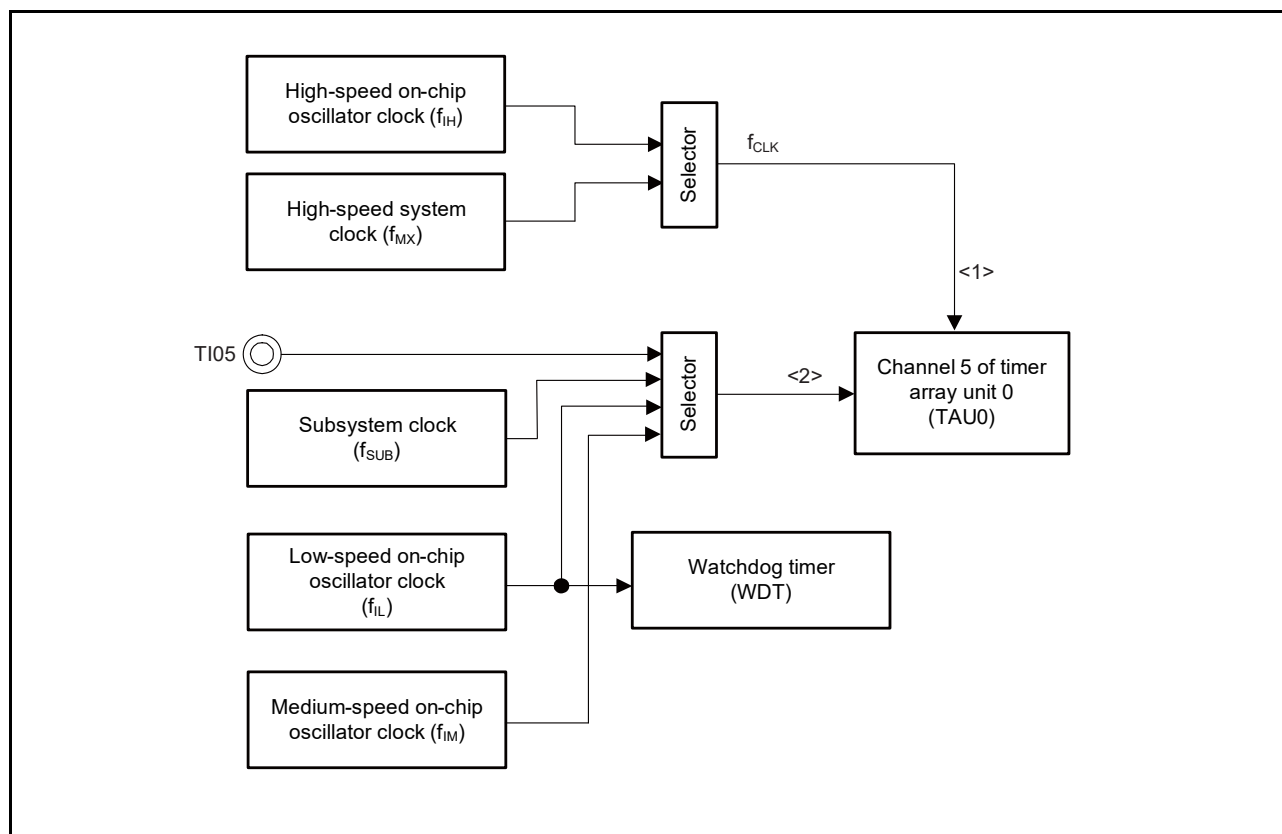
Figure 24 - 17 Configuration of Frequency Detection Function
