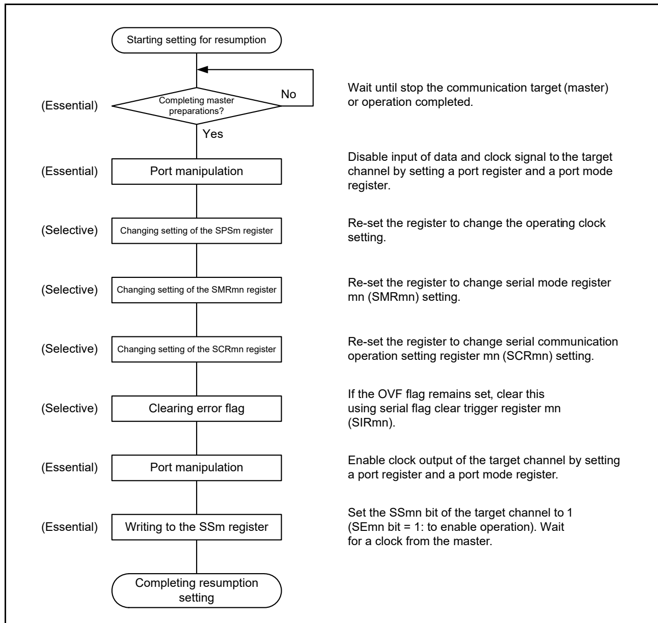
Figure 13 - 62 Procedure for Resuming Slave Reception
