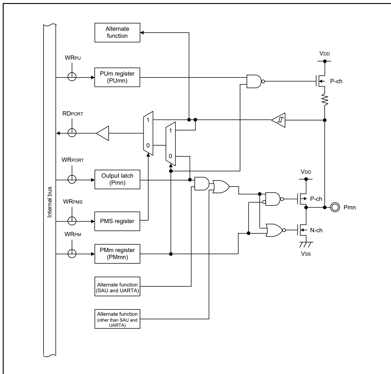
Figure 2 - 19 Pin Block Diagram for Pin Type 7-38-1
