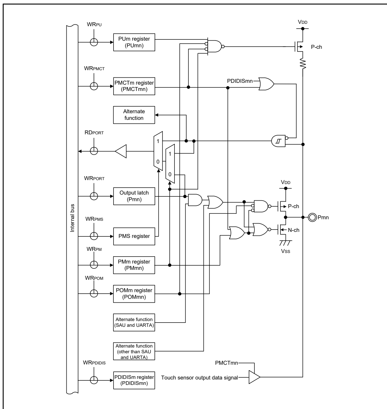
Figure 2 - 17 Pin Block Diagram for Pin Type 7-31-3
