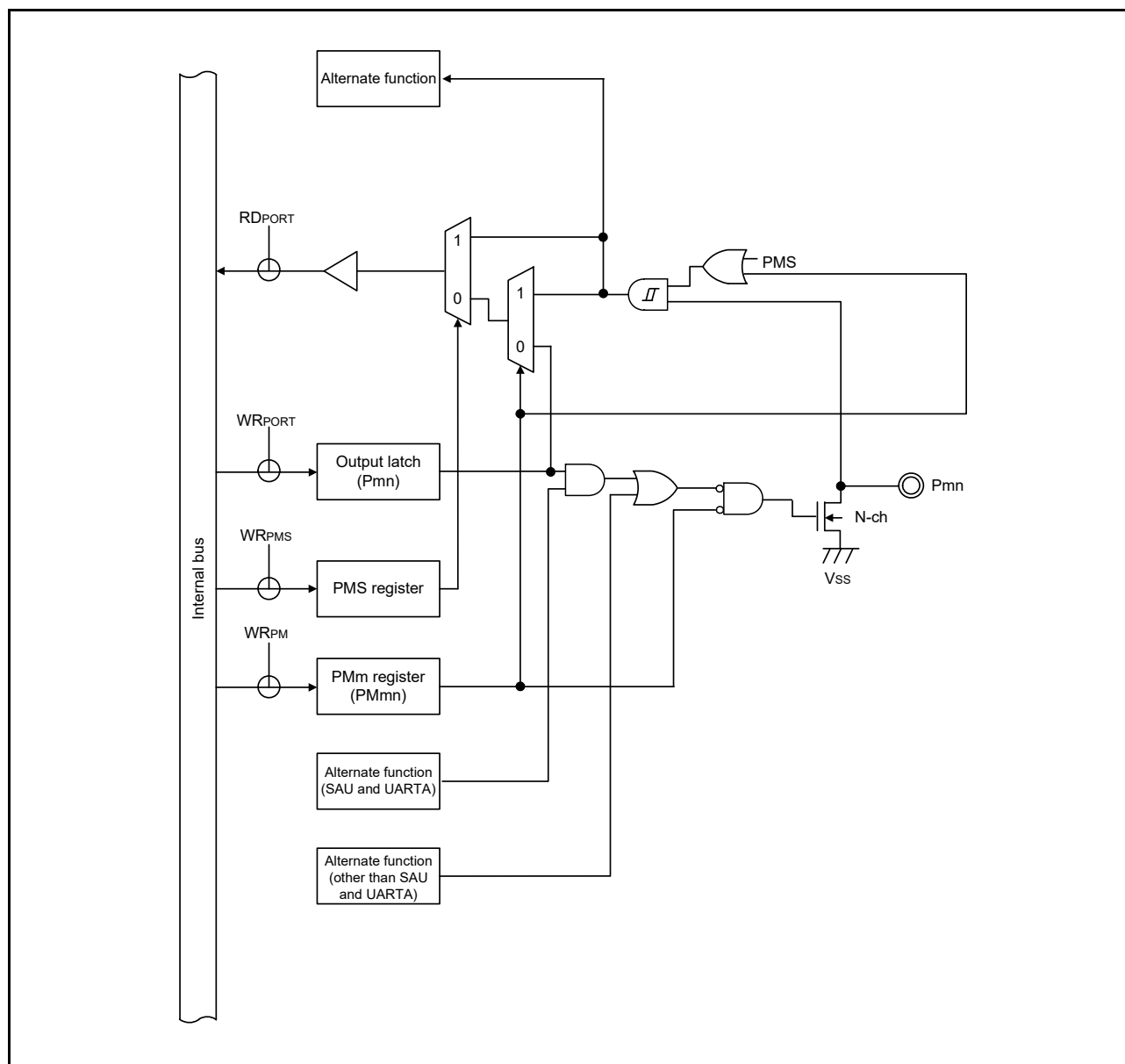
Figure 2 - 28 Pin Block Diagram for Pin Type 12-38-1
