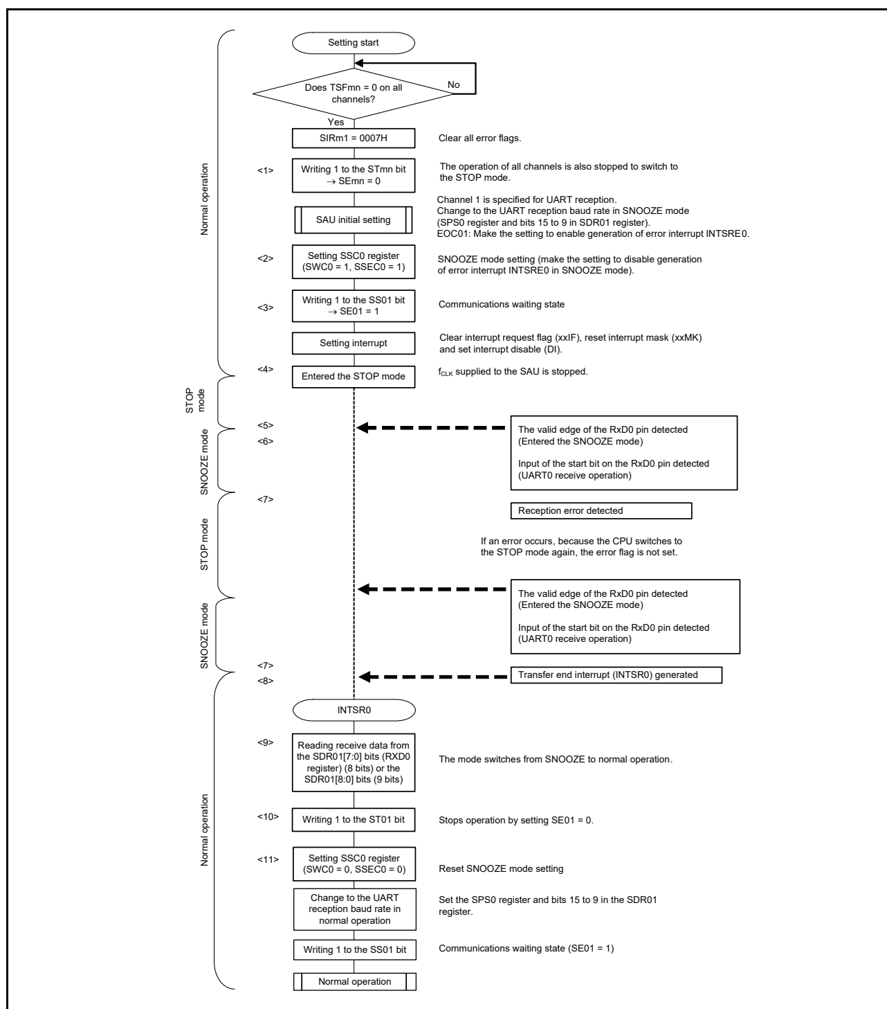
Figure 13 - 95 Flowchart of SNOOZE Mode Operation (EOC01 = 1, SSEC0 = 1)
