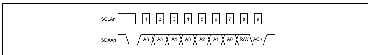
Figure 14 - 18 ACK
