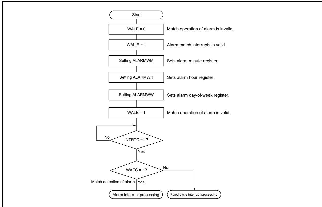
Figure 8 - 23 Alarm Processing Procedure
