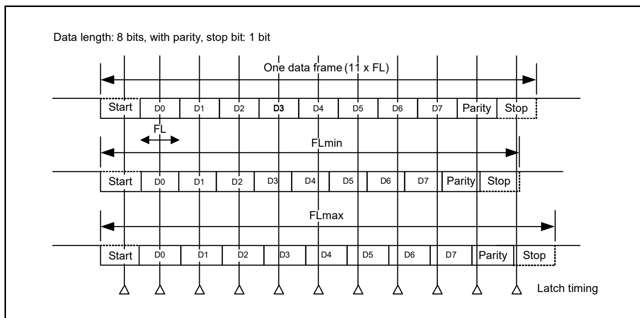
Figure 15 - 24 Permissible Baud Rate Range during Reception
