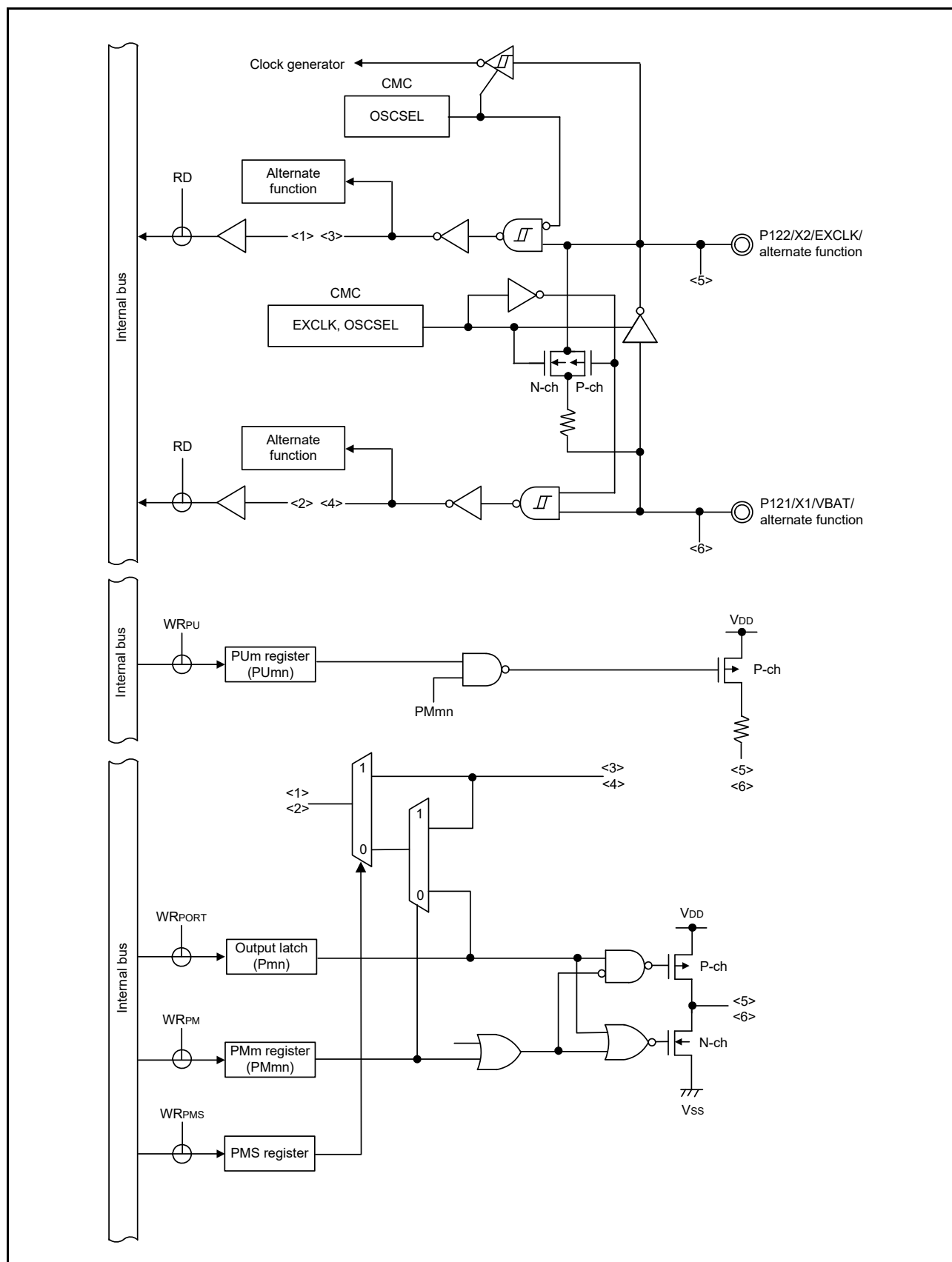
Figure 2 - 13 Pin Block Diagram for Pin Type 7-2-1
