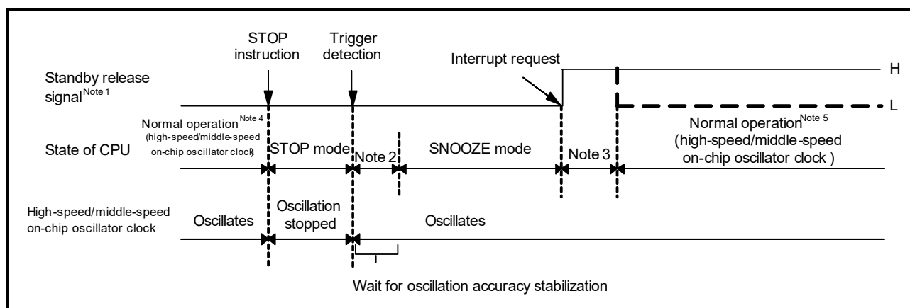
Figure 20 - 6 When the Interrupt Request Signal is Generated in the SNOOZE Mode
