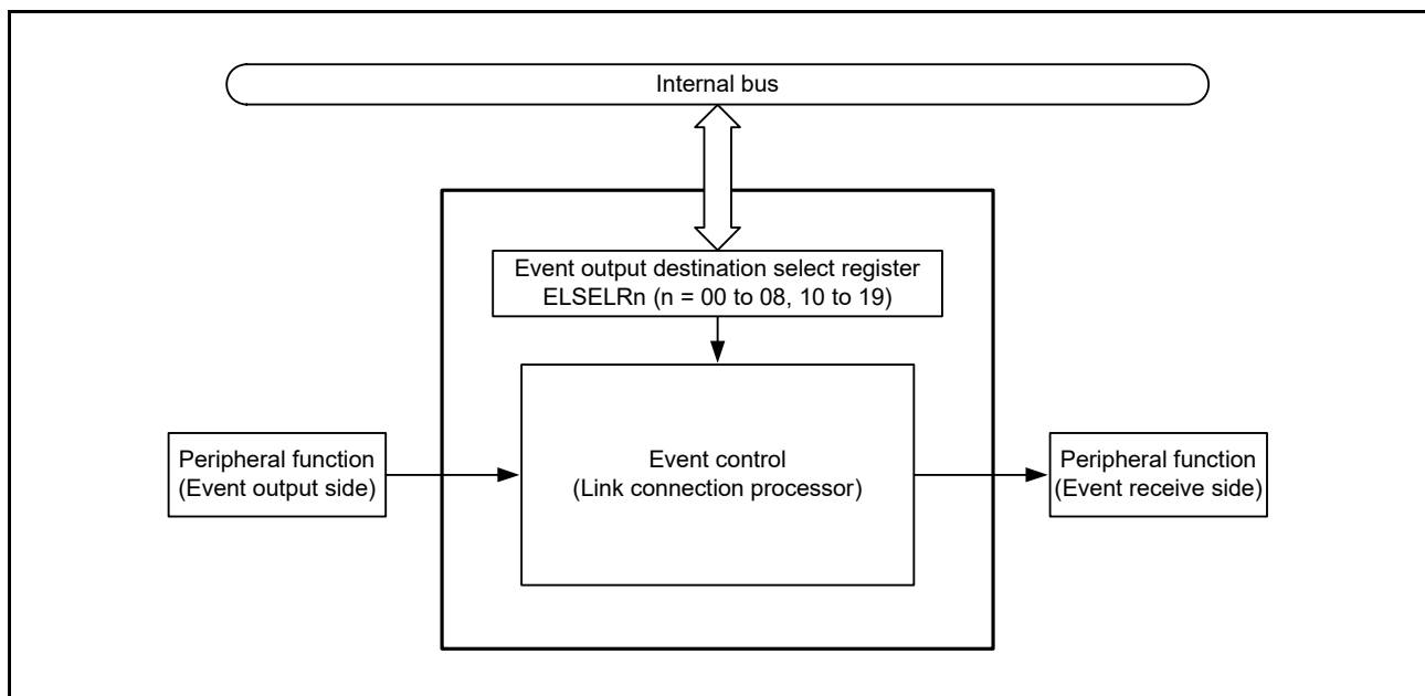
Figure 17 - 1 Block Diagram of the ELC
