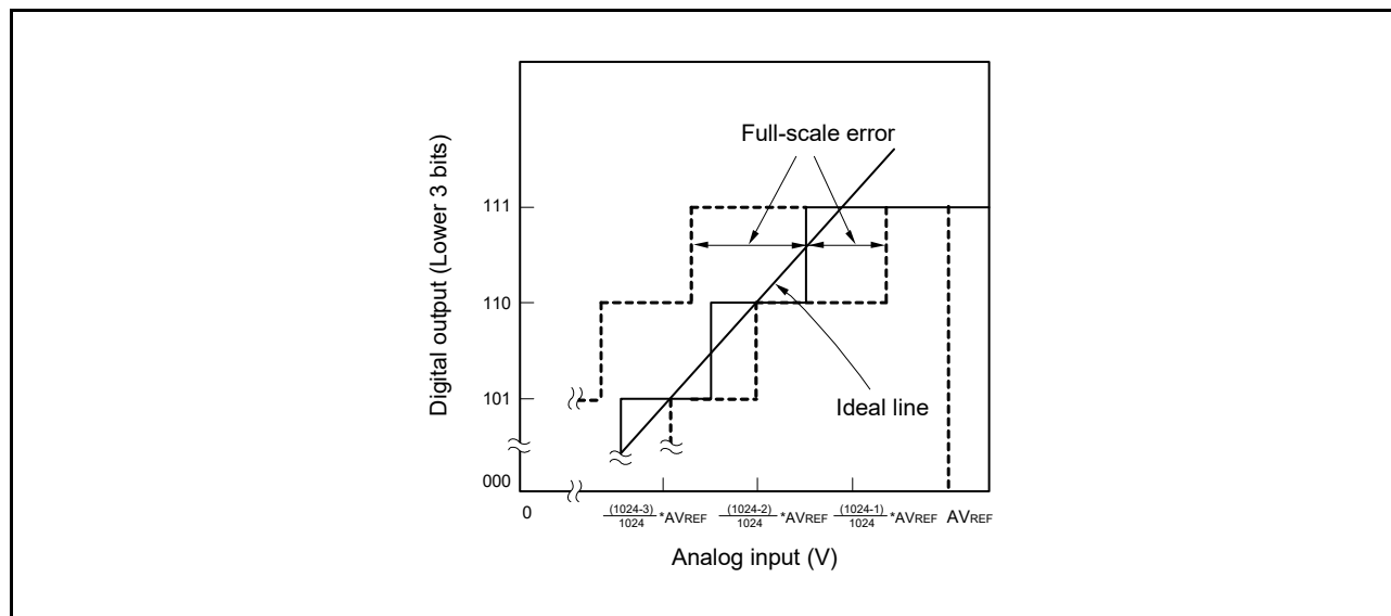
Figure 12 - 42 Full-Scale Error
