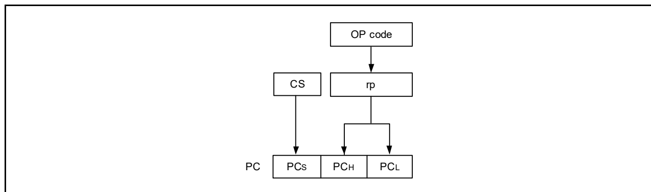
Figure 3 - 16 Outline of Register Indirect Addressing
