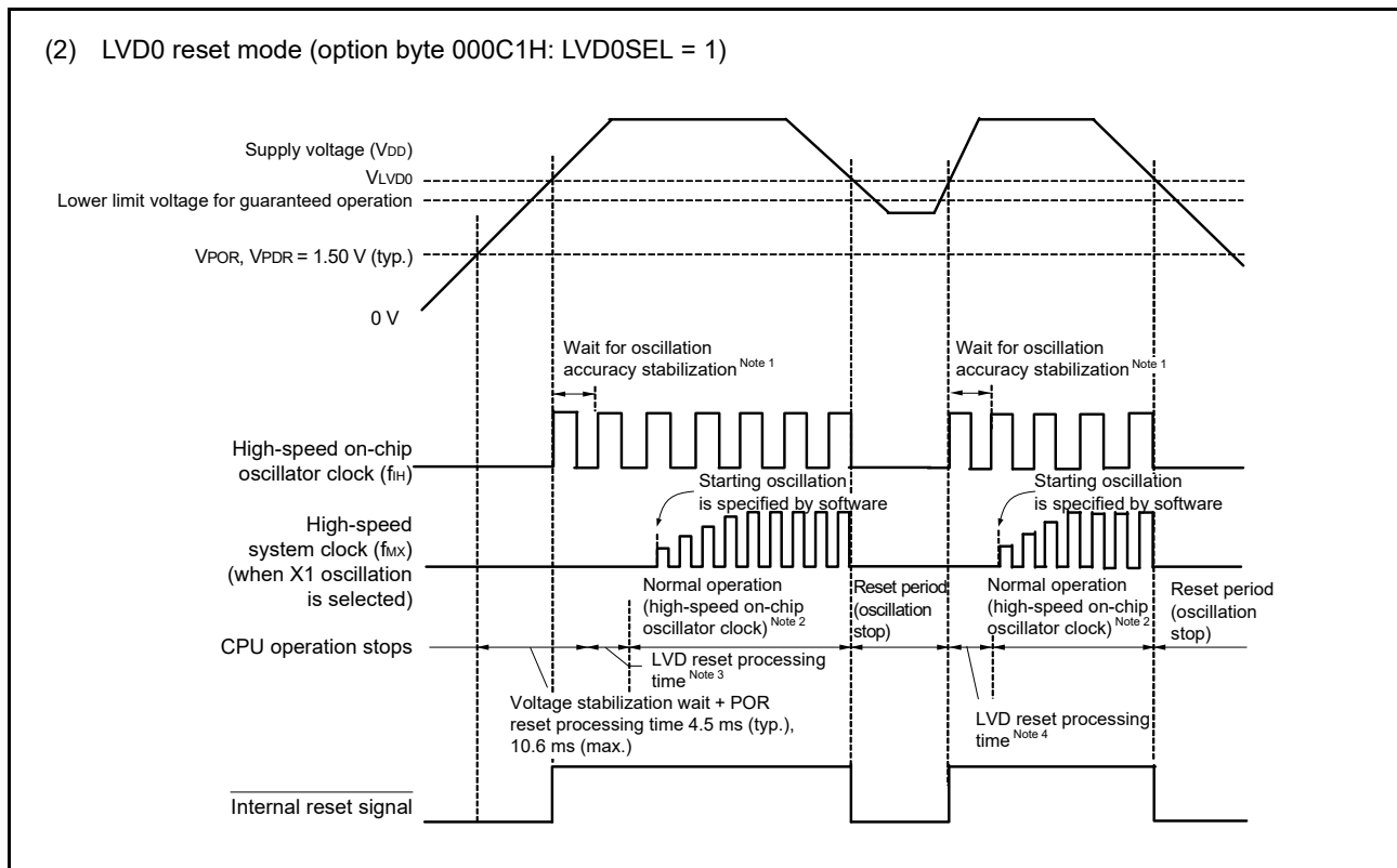
Figure 22 - 2 Timing of Generation of Internal Reset Signal by Power-on-reset Circuit and Voltage Detector (2/2)
