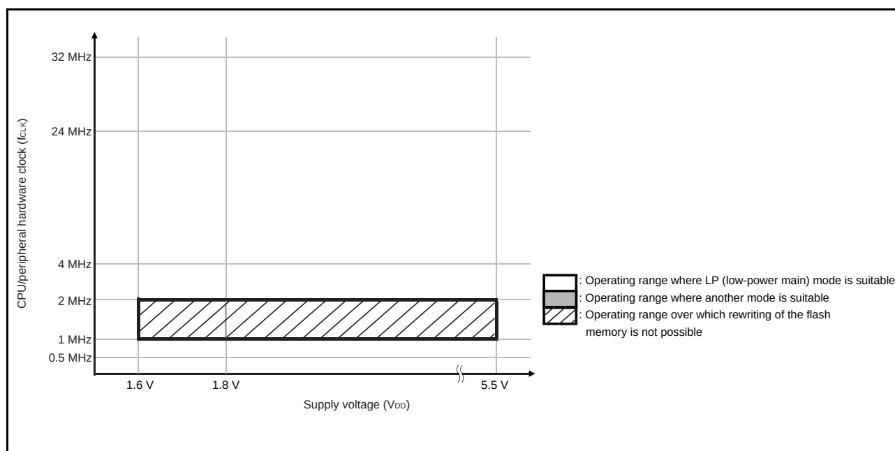
Figure 5 - 7 Operating Range in LP (Low-Power Main) Mode
