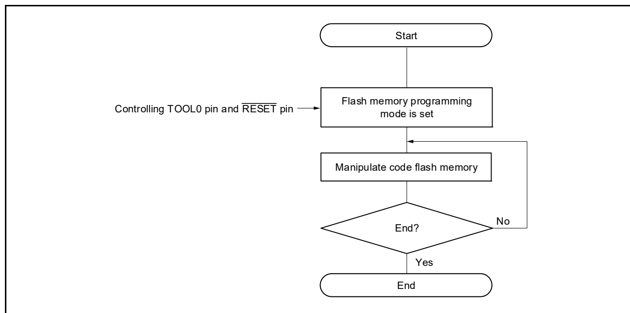
Figure 30 - 6 Code Flash Memory Manipulation Procedure
