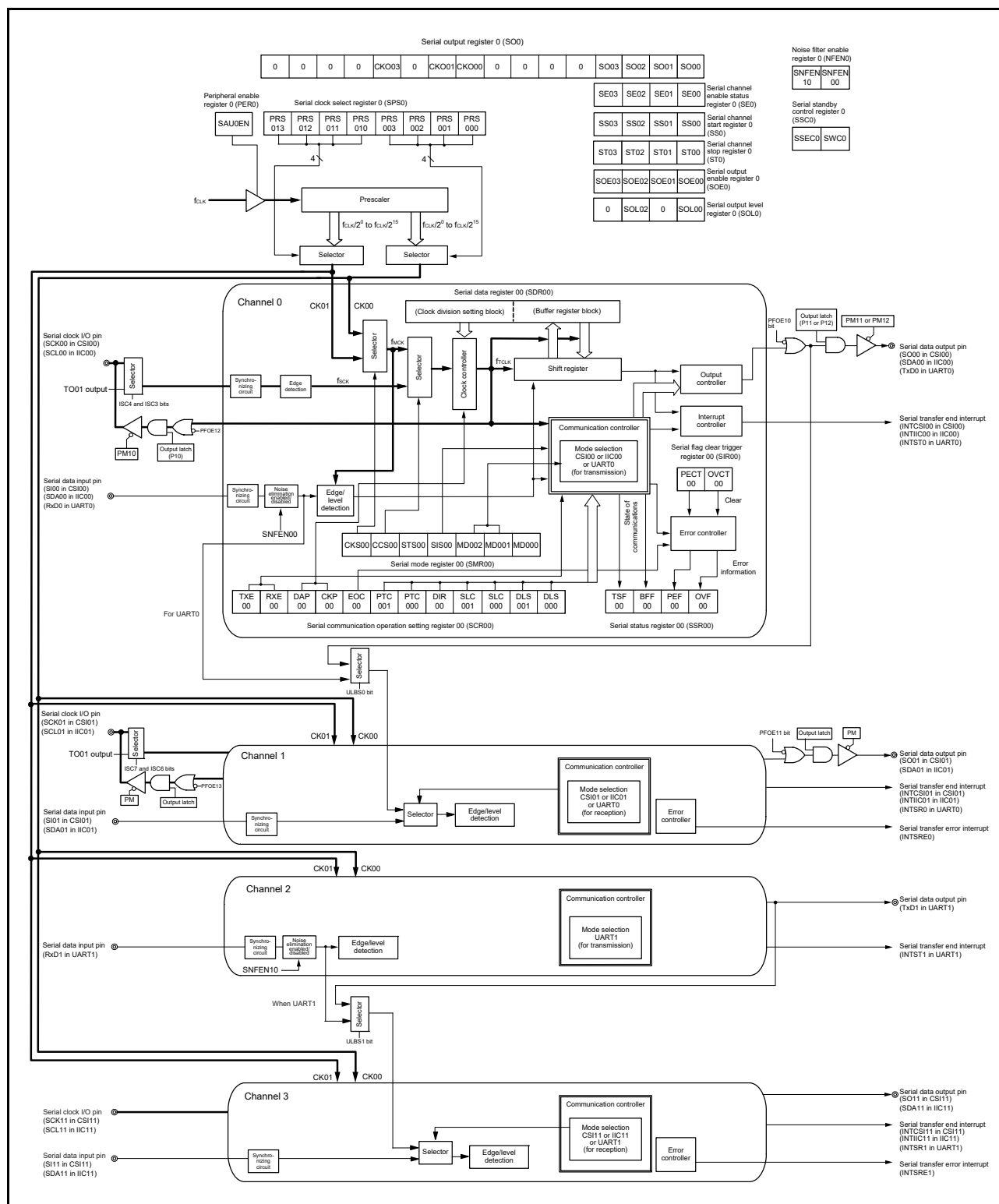
Figure 13 - 1 Block Diagram of Serial Array Unit 0
