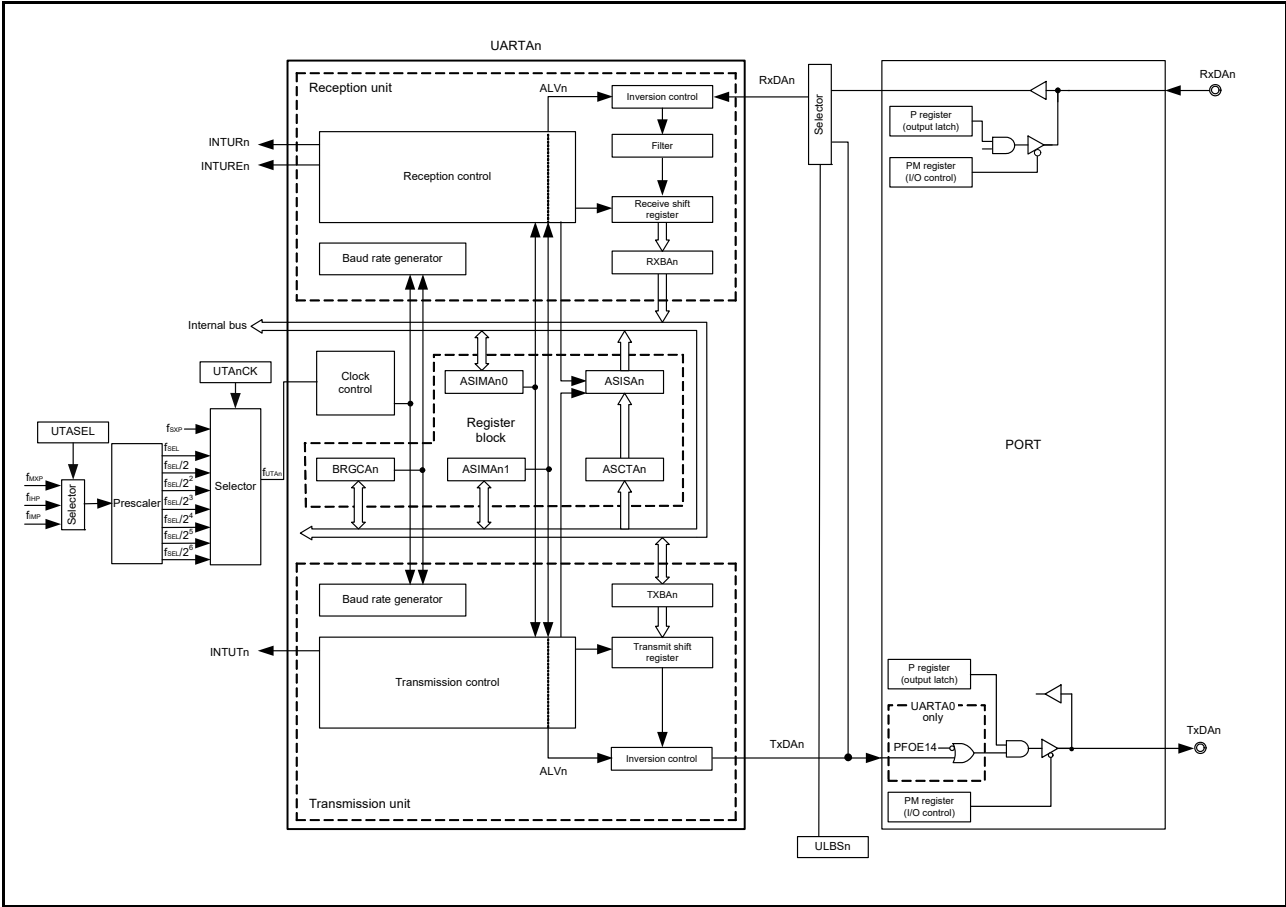
Figure 15 - 1 Block Diagram of UARTAn
