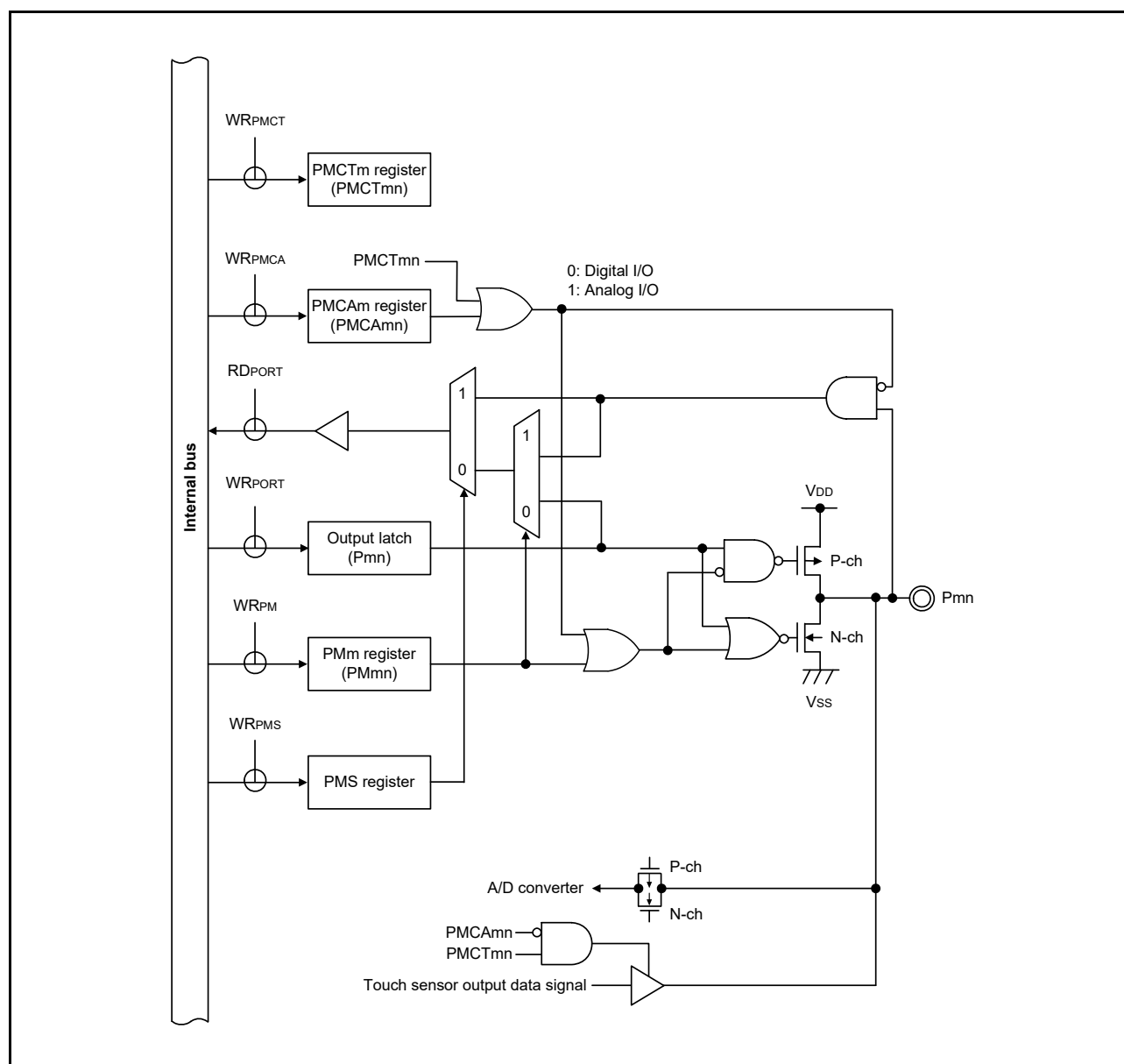
Figure 2 - 9 Pin Block Diagram for Pin Type 4-35-1
