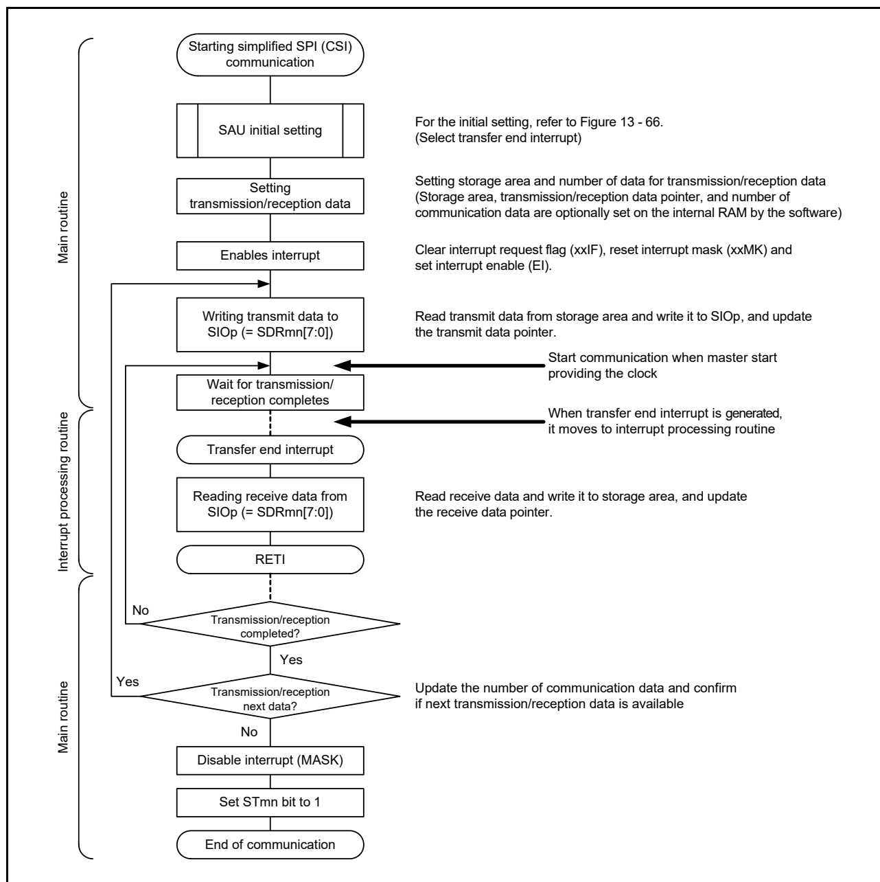
Figure 13 - 70 Flowchart of Slave Transmission/Reception (in Single-Transmission/Reception Mode)
