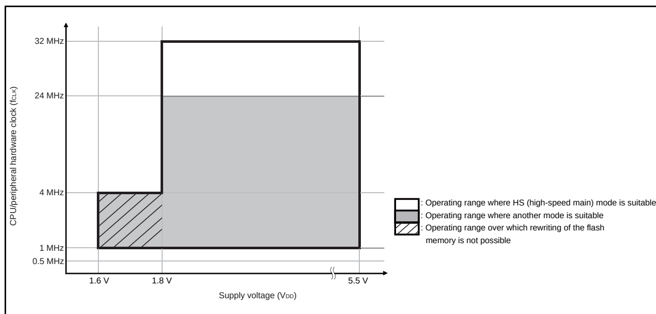
Figure 5 - 5 Operating Range in HS (High-Speed Main) Mode
