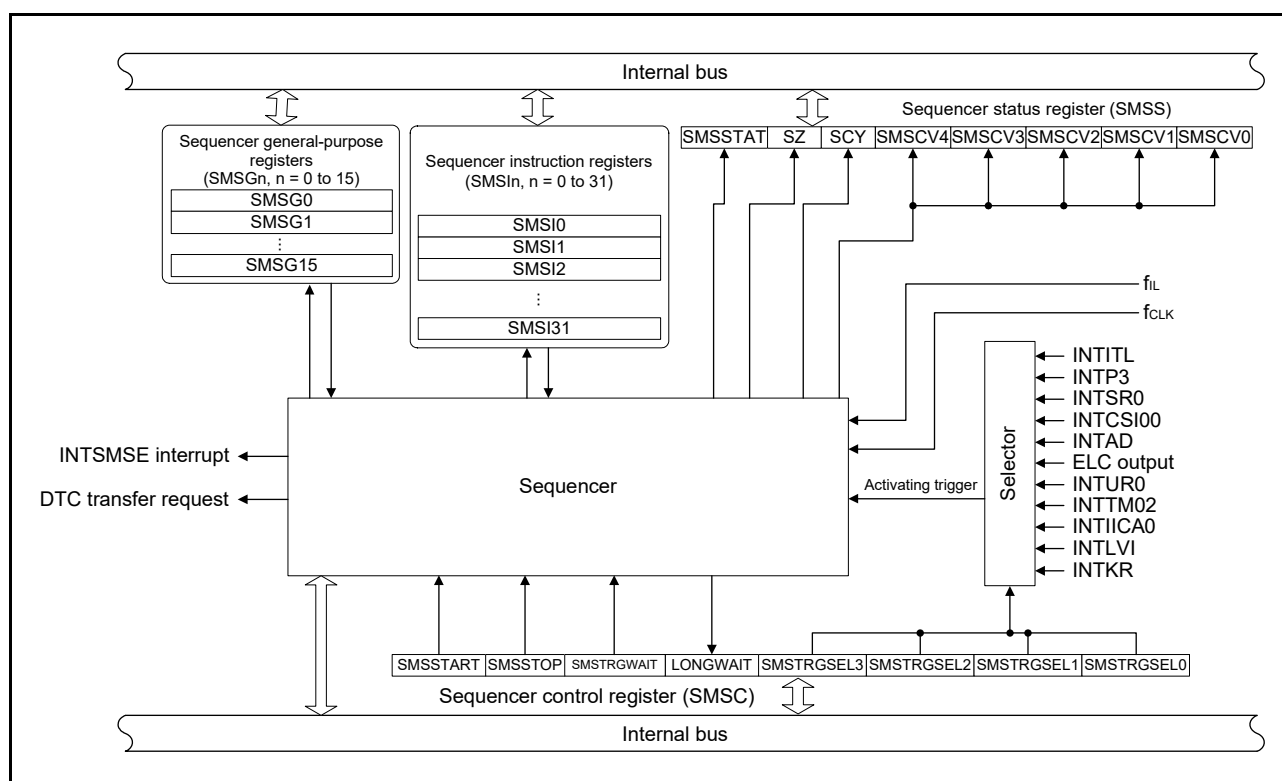
Figure 26 - 1 Block Diagram of the SNOOZE Mode Sequencer
