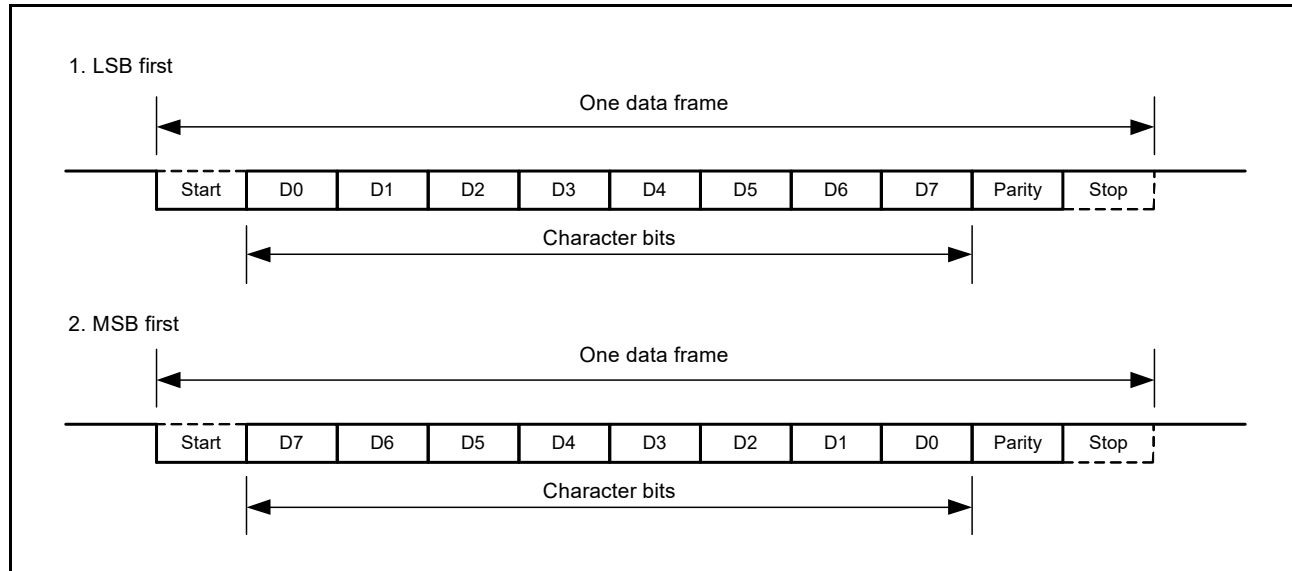
Figure 15 - 13 Transmit/Receive Data Format
