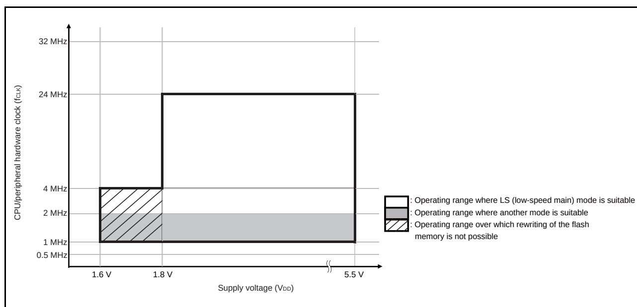
Figure 5 - 6 Operating Range in LS (Low-Speed Main) Mode
