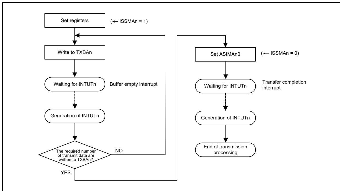
Figure 15 - 17 Flow Example of Continuous Transmission Using Interrupt
