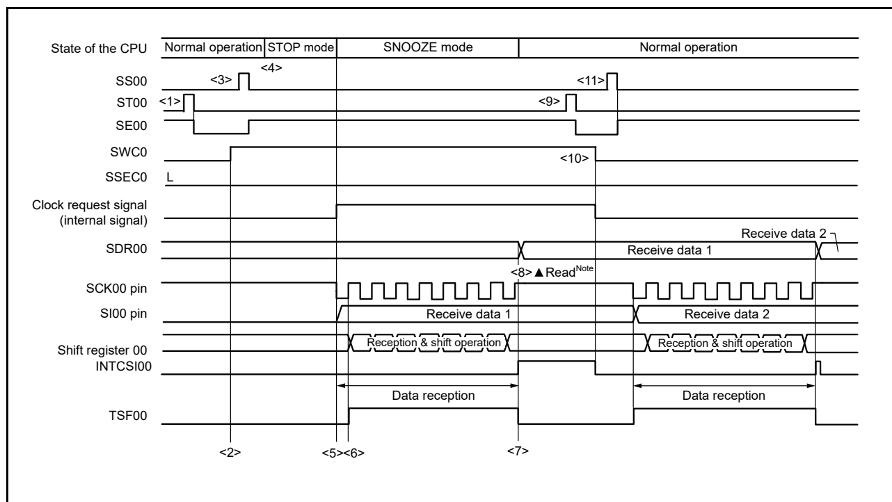
Figure 13 - 73 Timing Chart of SNOOZE Mode Operation (once startup) (Type 1: DAP00 = 0, CKP00 = 0)
