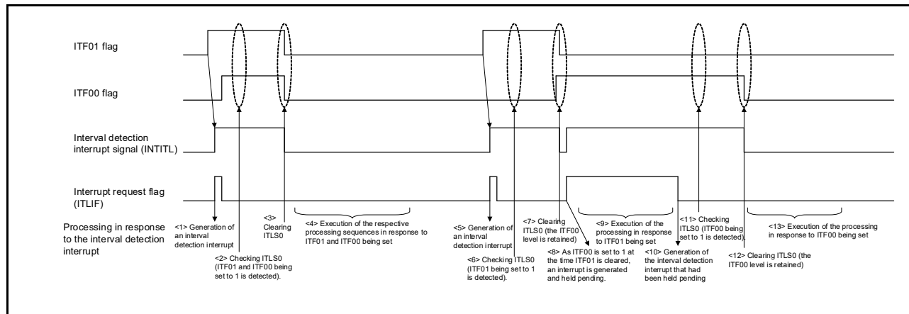
Figure 9 - 16 Example of Clearing the Detected Flags
