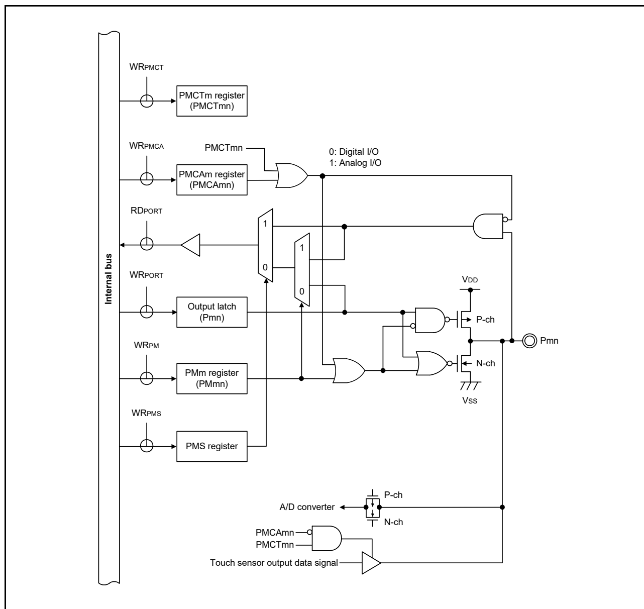
Figure 2 - 10 Pin Block Diagram for Pin Type 4-37-1
