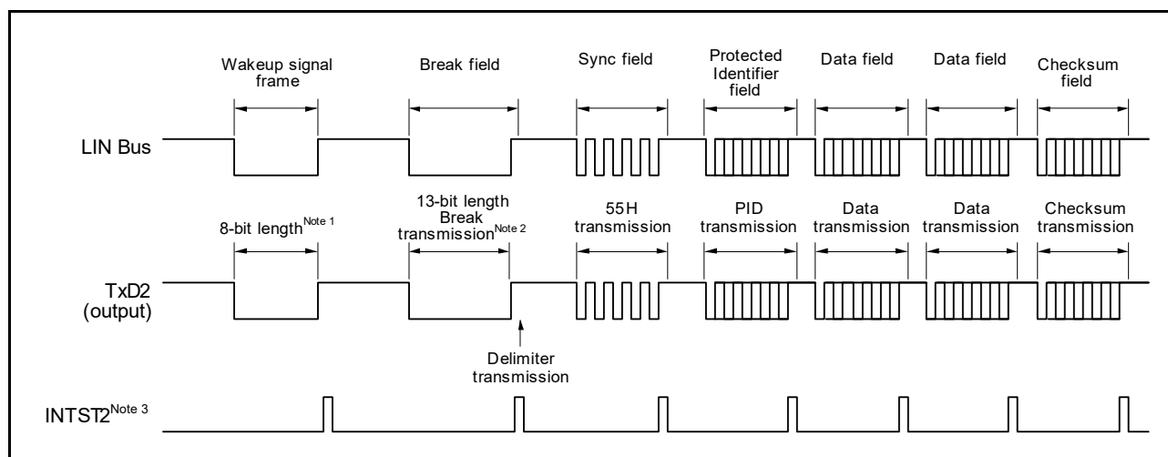
Figure 13 - 97 Transmission Operation of LIN
