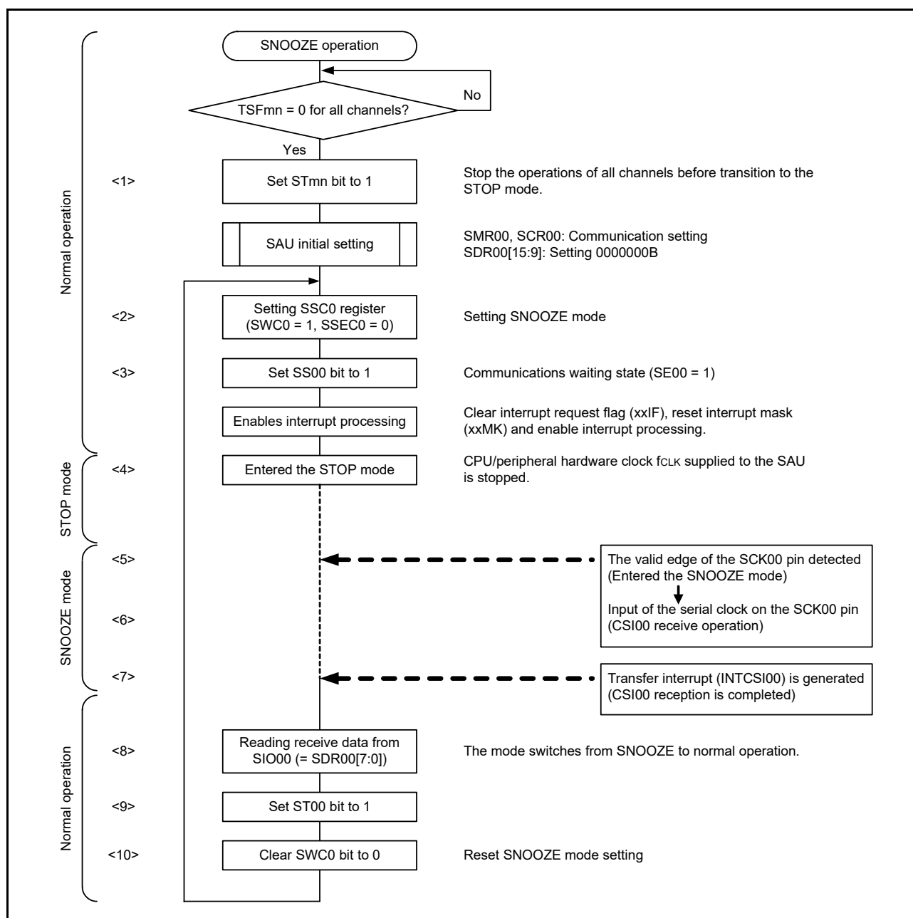
Figure 13 - 76 Flowchart of SNOOZE Mode Operation (continuous startup)
