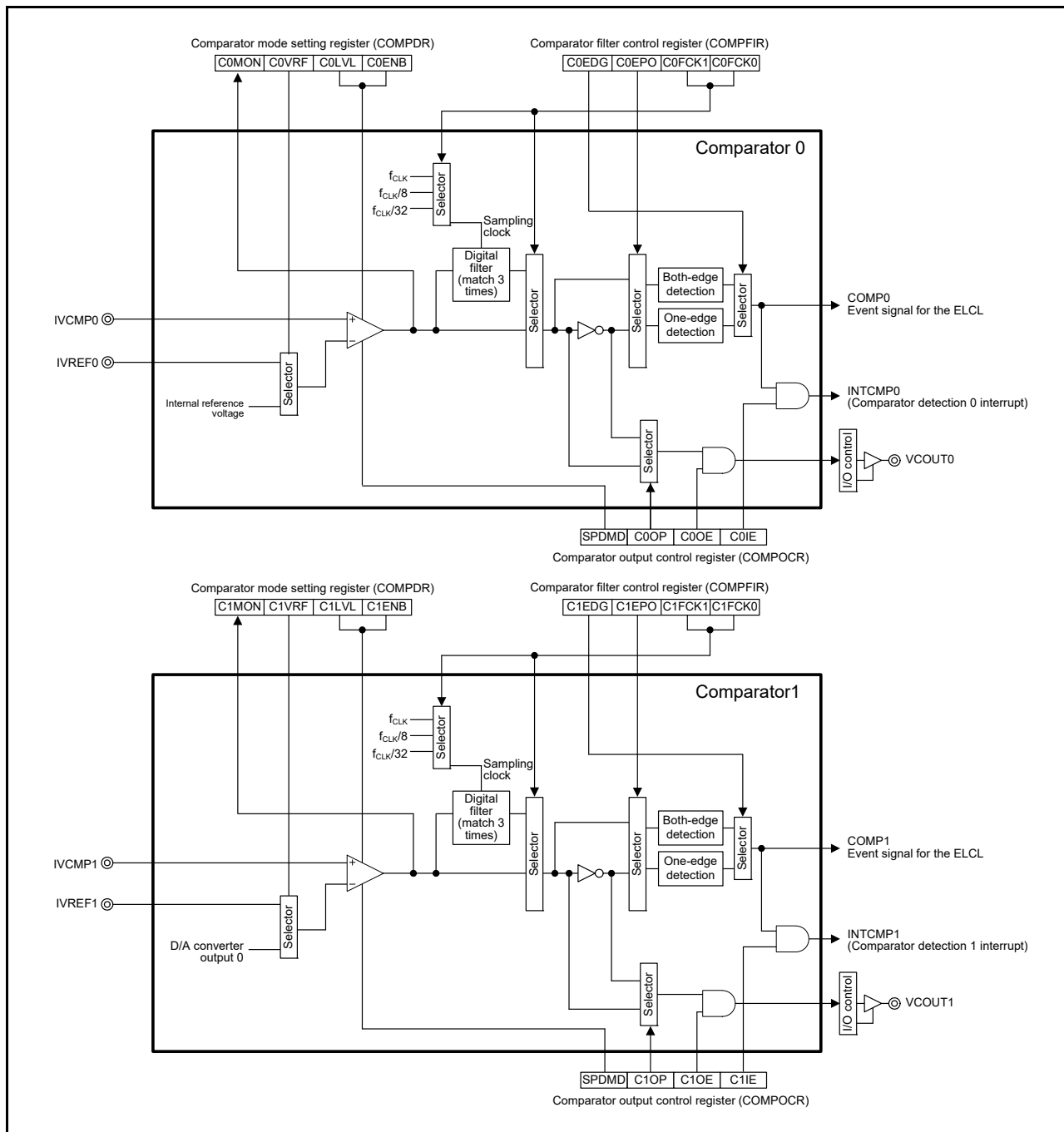
Figure 14 - 1 Comparator Block Diagram
