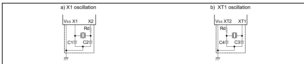
Figure 6 - 23 Examples of External Circuits
