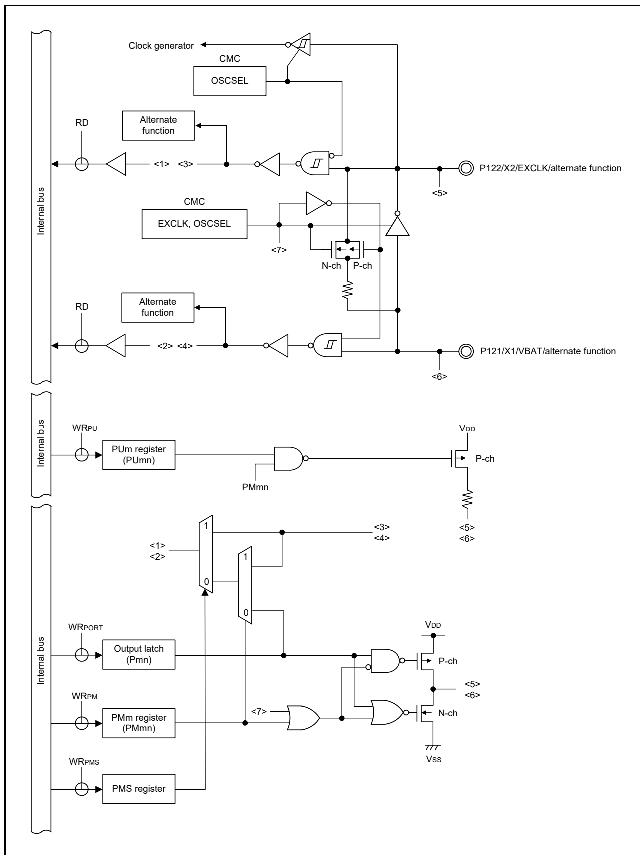
&lt;R&gt; Figure 2 - 14 Pin Block Diagram for Pin Type 7-2-1
