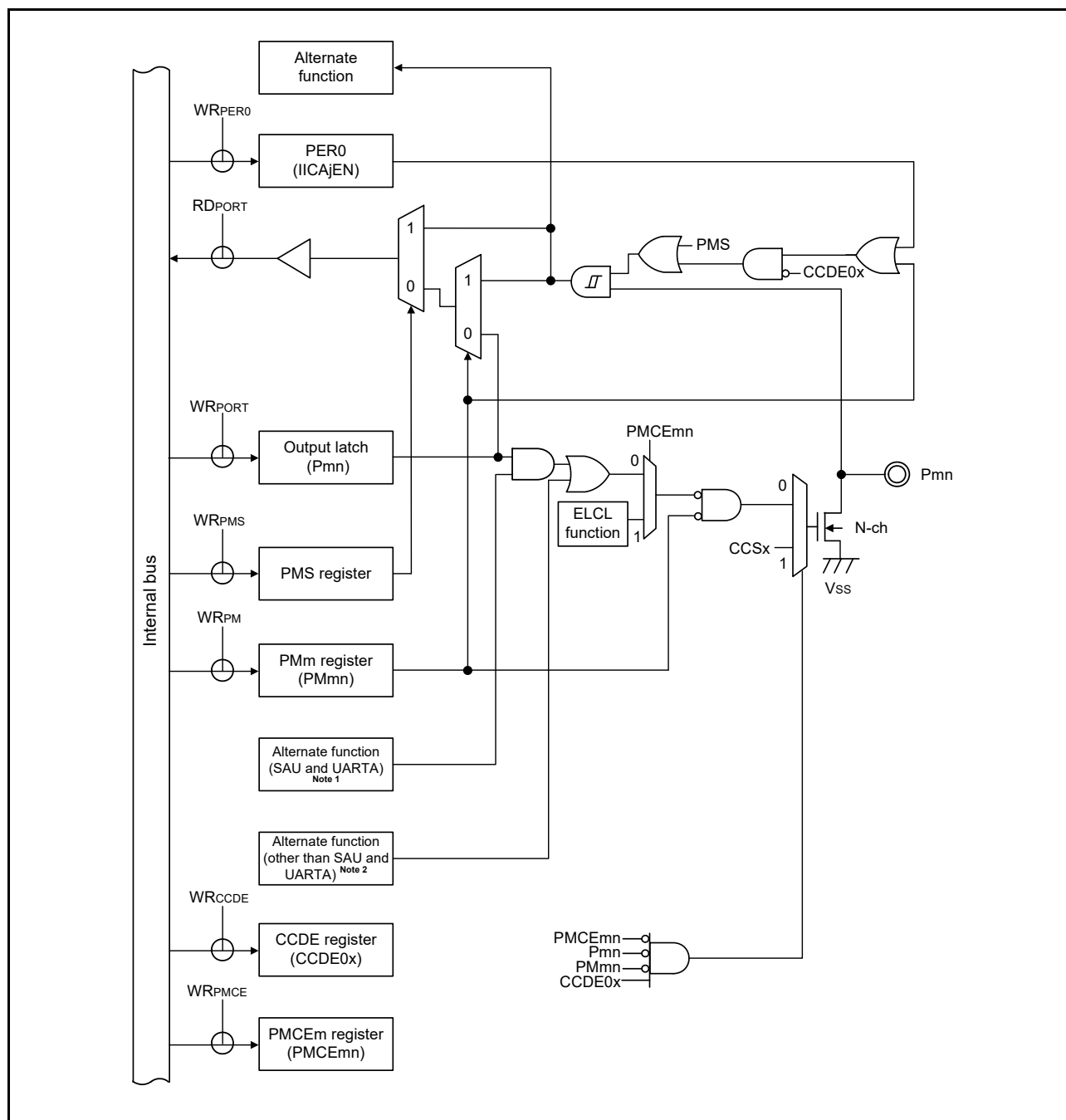
Figure 2 - 35 Pin Block Diagram for Pin Type 12-38-3
