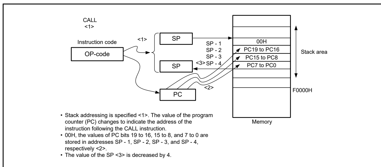
Figure 3 - 40 Example of CALL, CALLT
