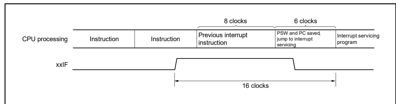
Figure 21 - 9 Interrupt Request Acknowledgment Timing (Maximum Time)
