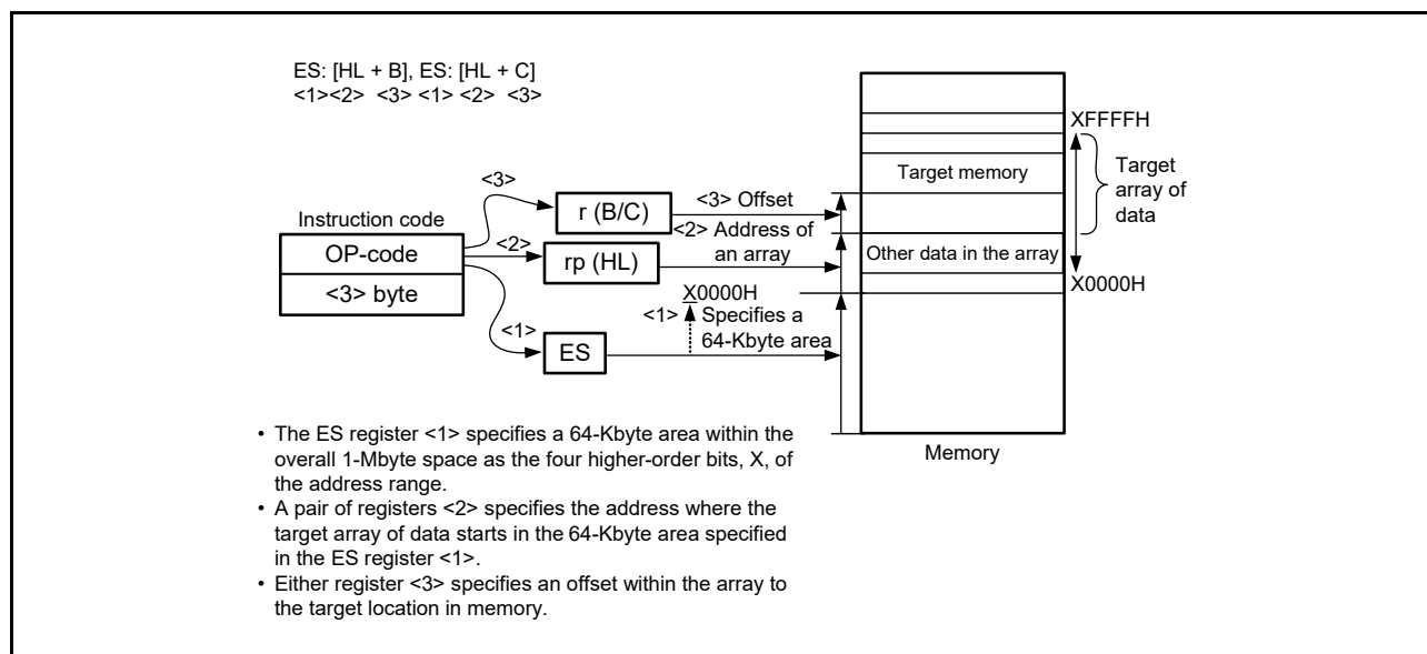
Figure 3 - 37 Example of ES:[HL + B], ES:[HL + C]
