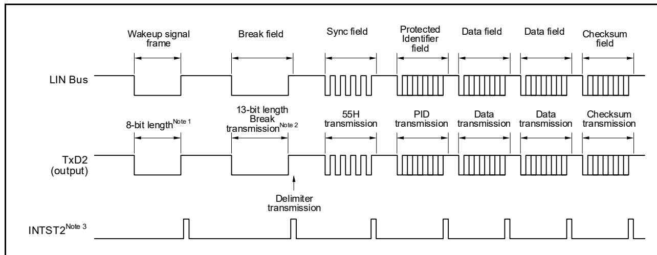
Figure 15 - 96 Transmission Operation of LIN
