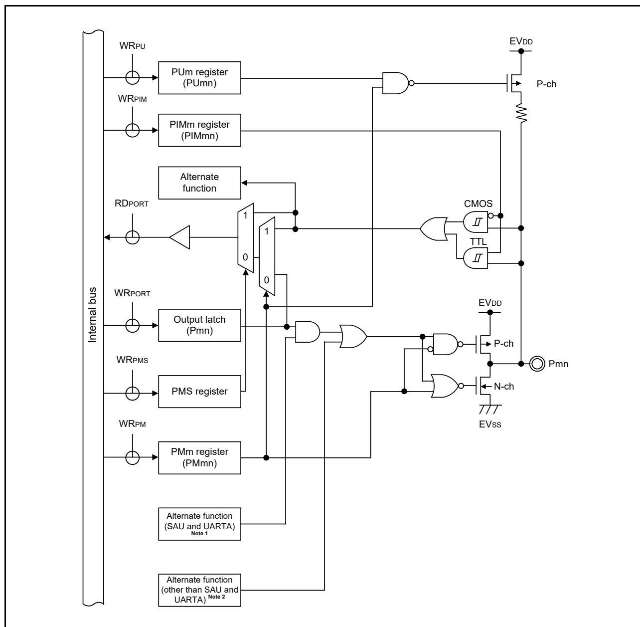
Figure 2 - 23 Pin Block Diagram for Pin Type 8-1-3
