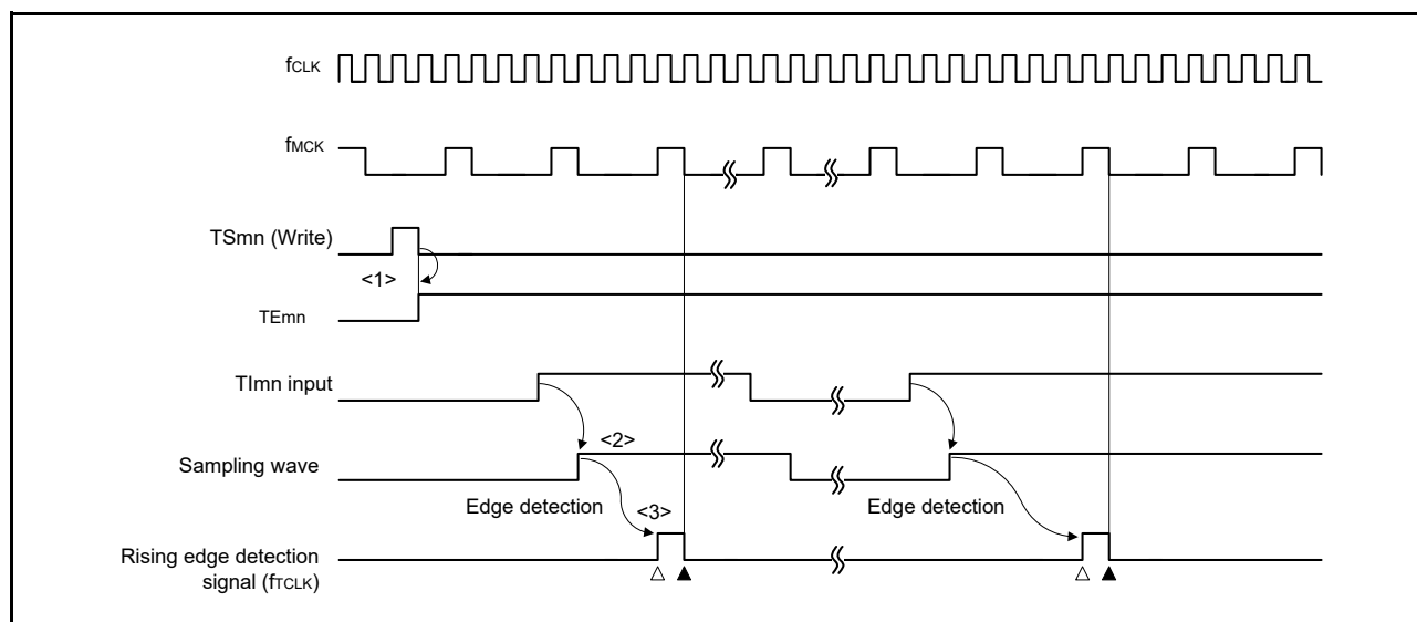
Figure 7 - 28 Timing of f CLK and Counter Clock (f TCLK ) (When CCSmn = 1, Noise Filter Unused)
