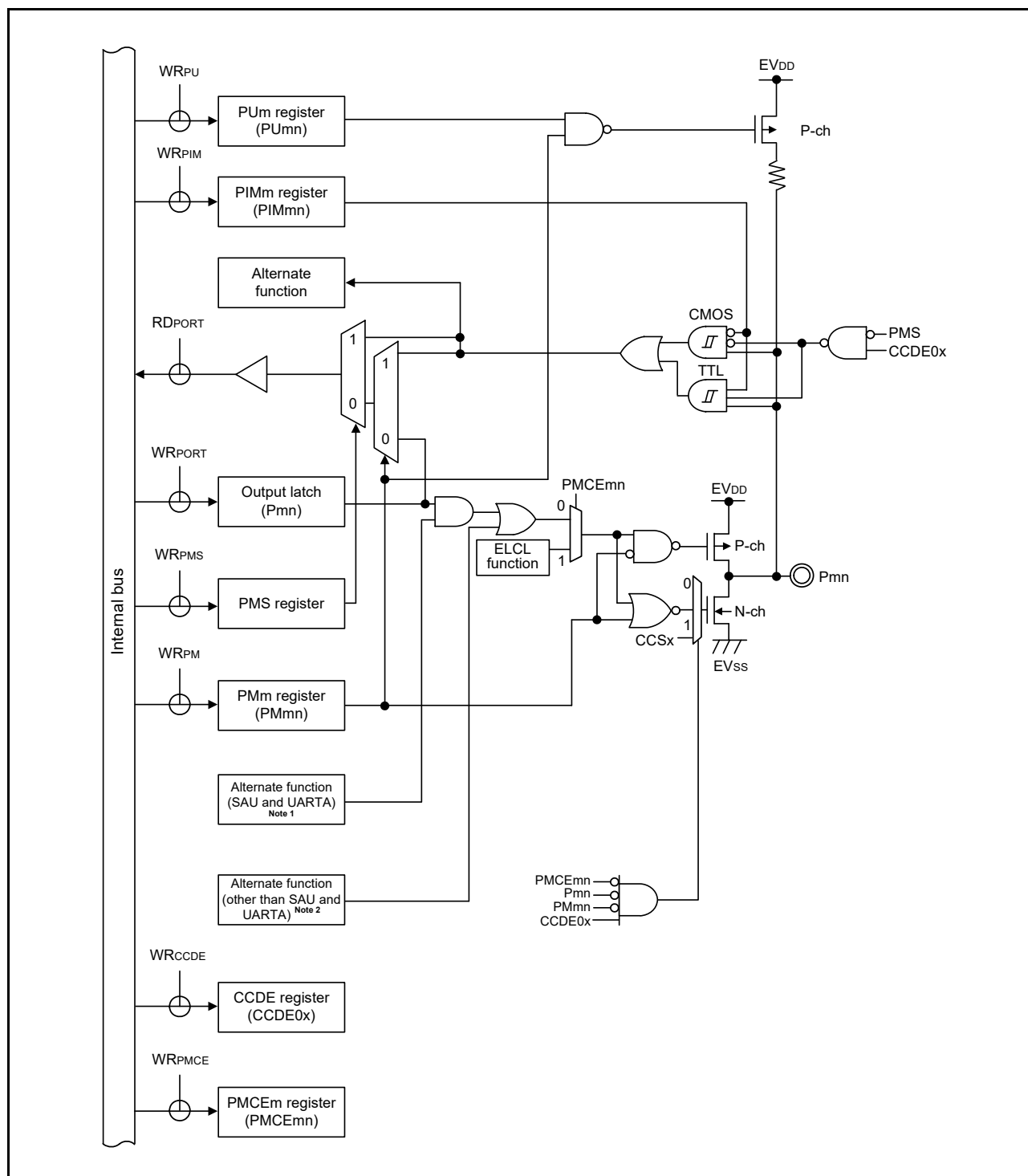
Figure 2 - 31 Pin Block Diagram for Pin Type 8-38-1
