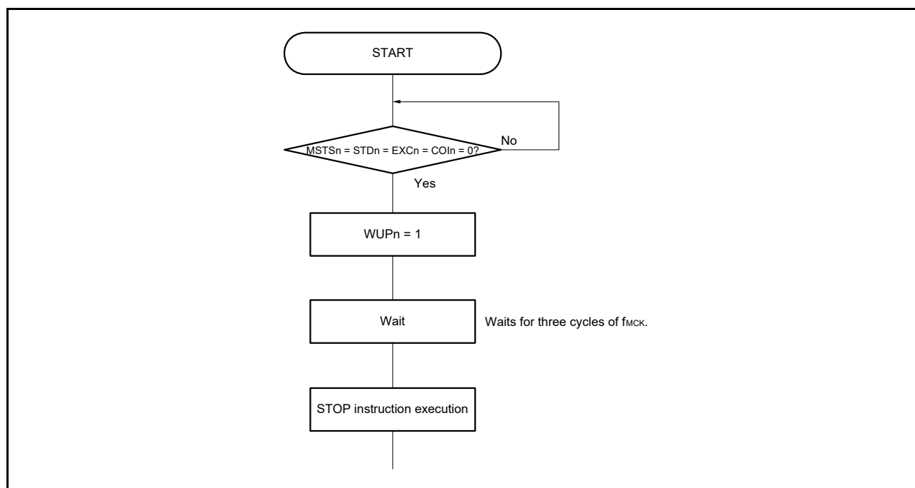
Figure 16 - 22 Flow When Setting WUPn = 1
