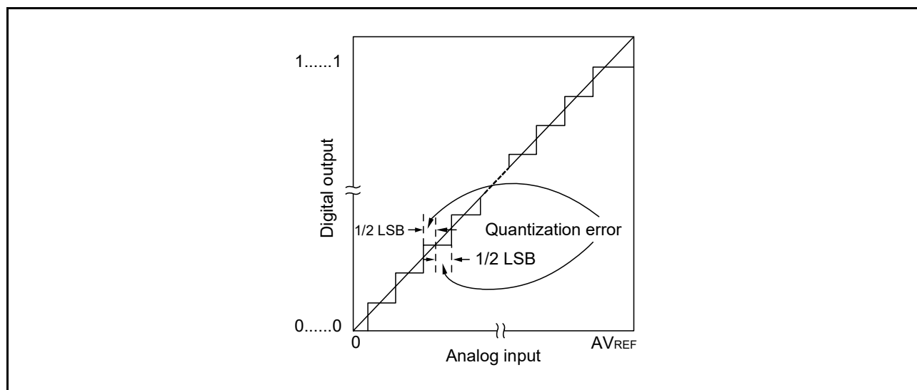
Figure 12 - 47 Quantization Error
