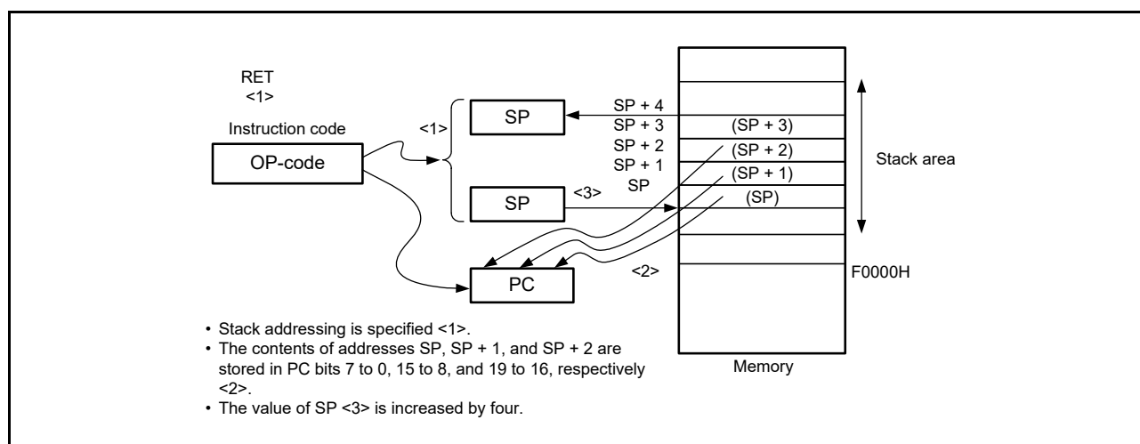
Figure 3 - 41 Example of RET
