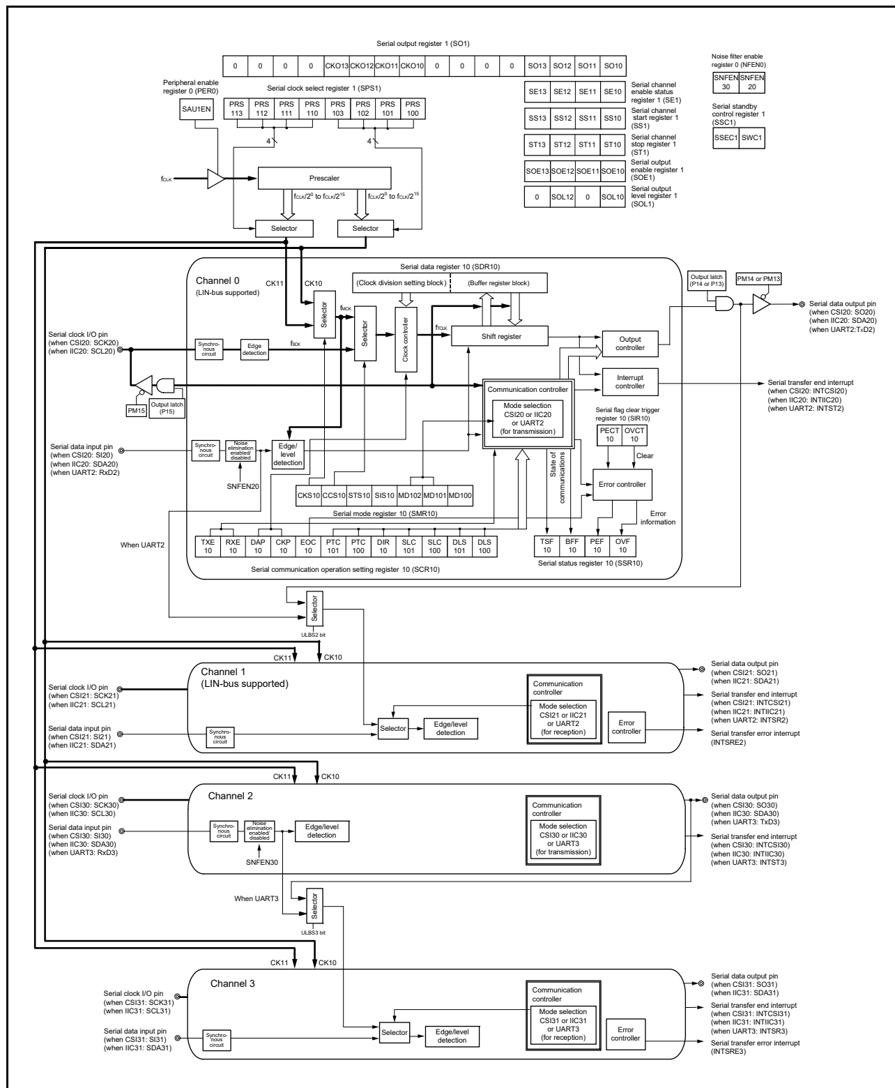
Figure 15 - 2 Block Diagram of Serial Array Unit 1
