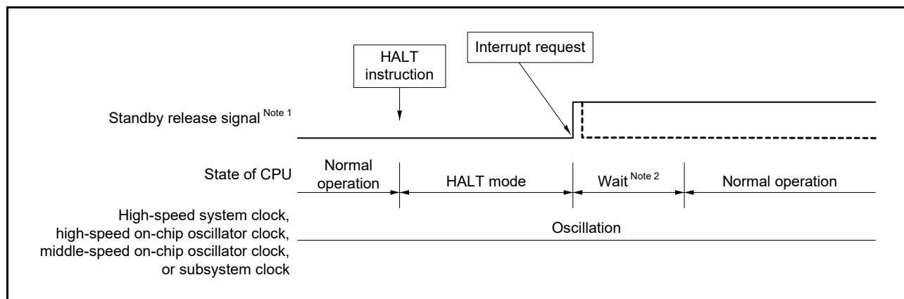
Figure 23 - 5 HALT Mode Release by Interrupt Request Generation
