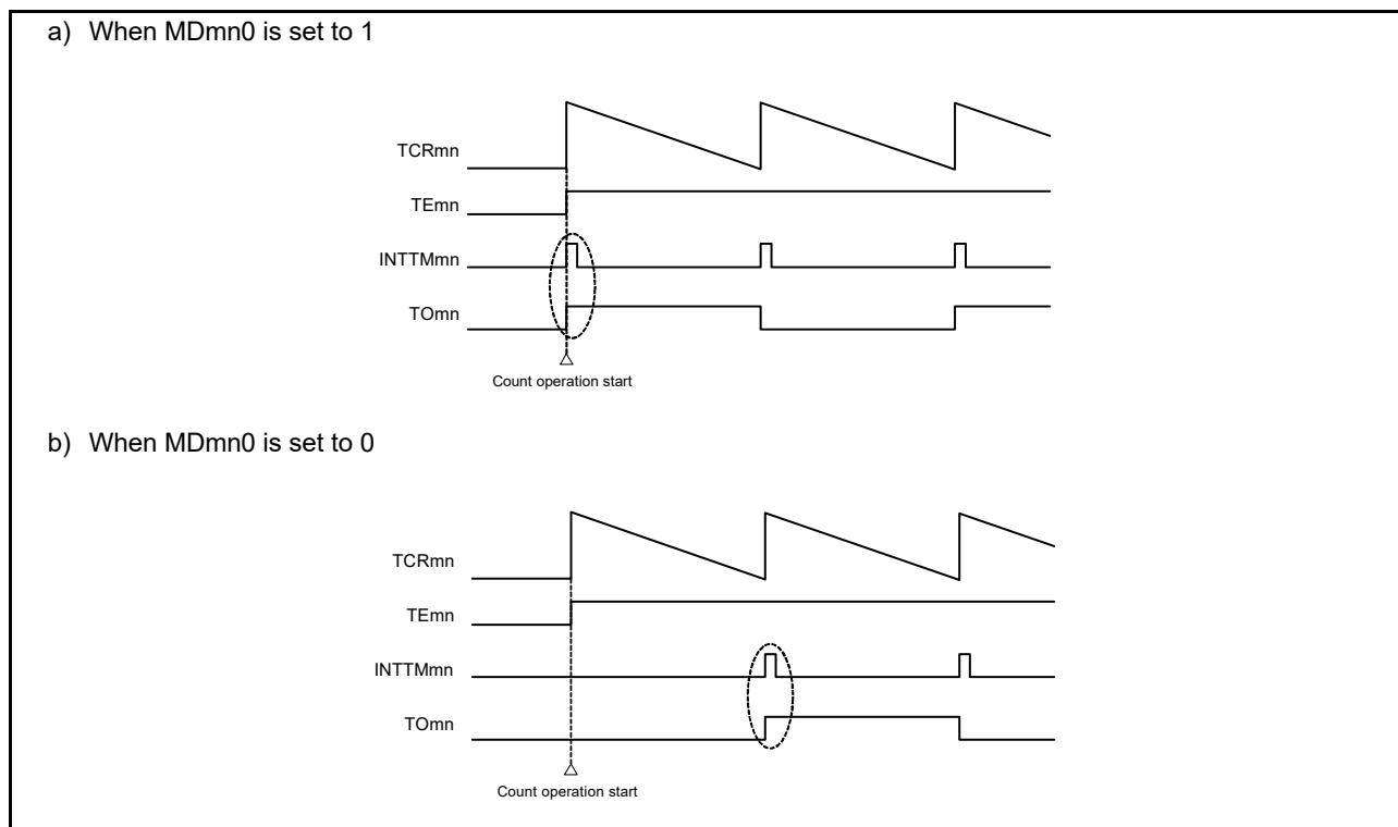
Figure 7 - 42 Examples of the Operation of Timer Interrupts and TOMn Outputs When Counting Is Started
