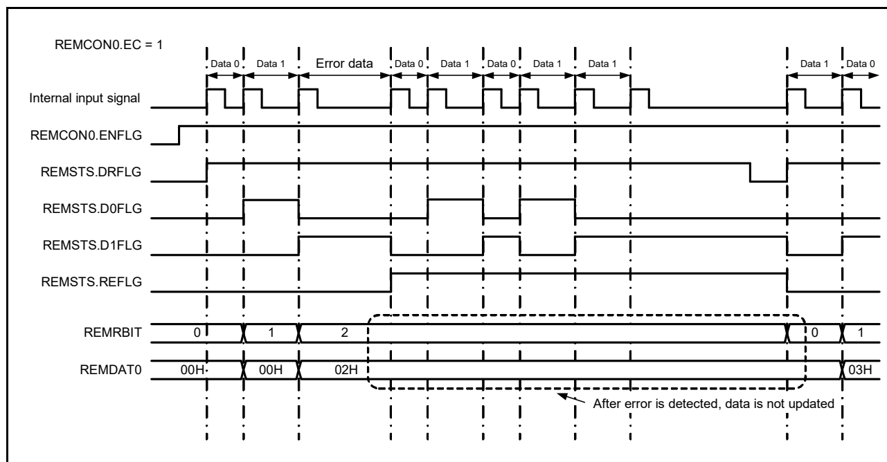
Figure 18 - 40 REMDAT0 and REMRBIT Registers Operation upon Error Detection (REMCN0.EC Bit = 1)
