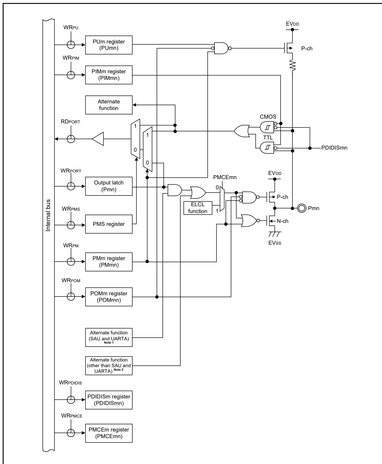
Figure 2 - 25 Pin Block Diagram for Pin Type 8-1-11
