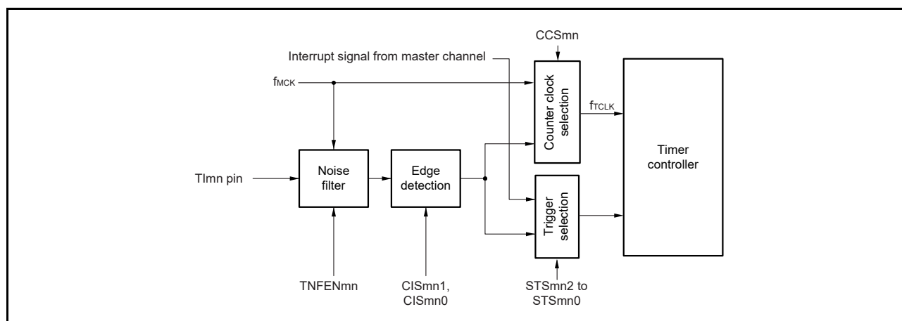
Figure 7 - 43 Input Circuit Configuration
