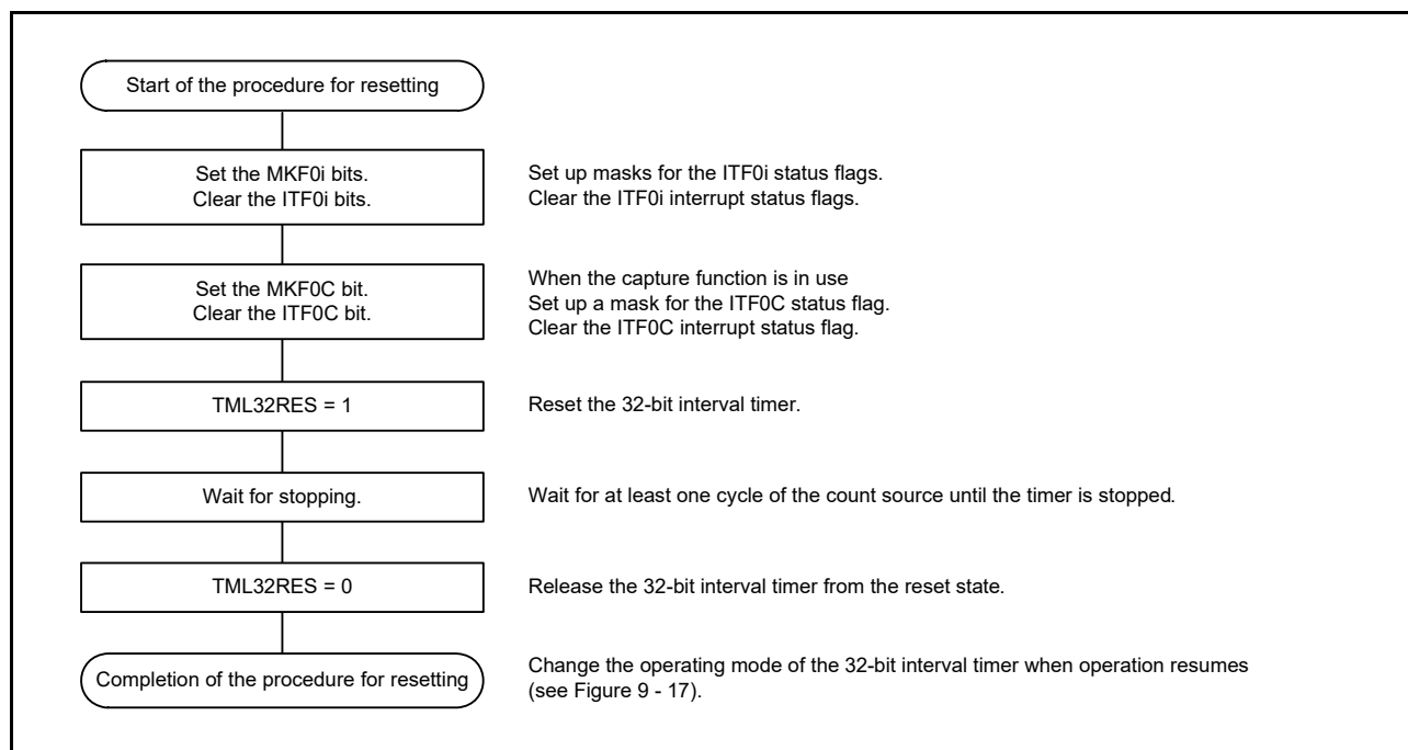
Figure 9 - 20 Procedure for Resetting the 32-Bit Interval Timer
