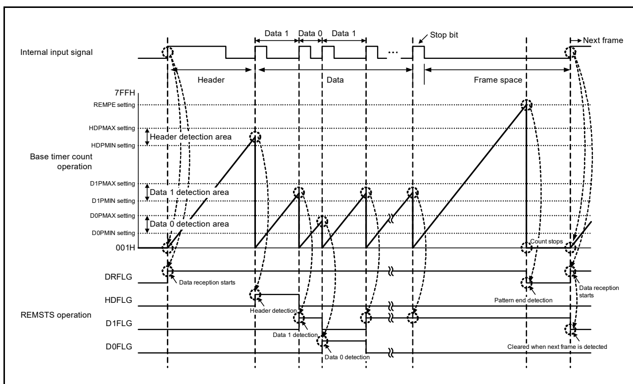
Figure 18 - 30 Waveform of REMC Operation
