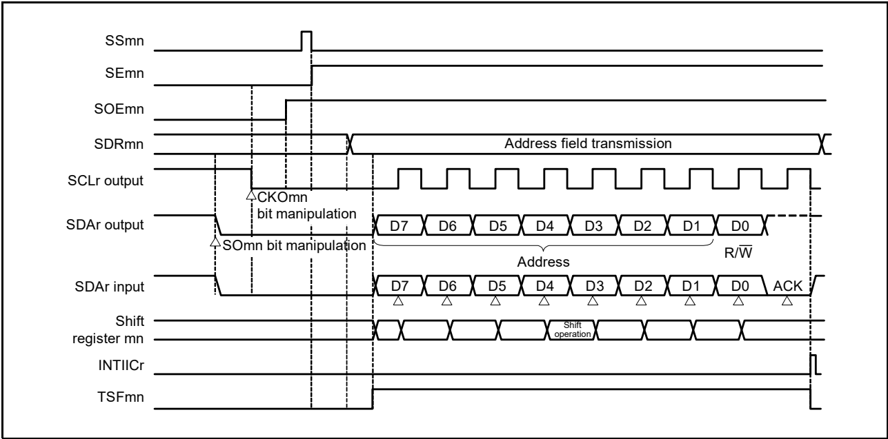
Figure 15 - 104 Timing Chart of Address Field Transmission
