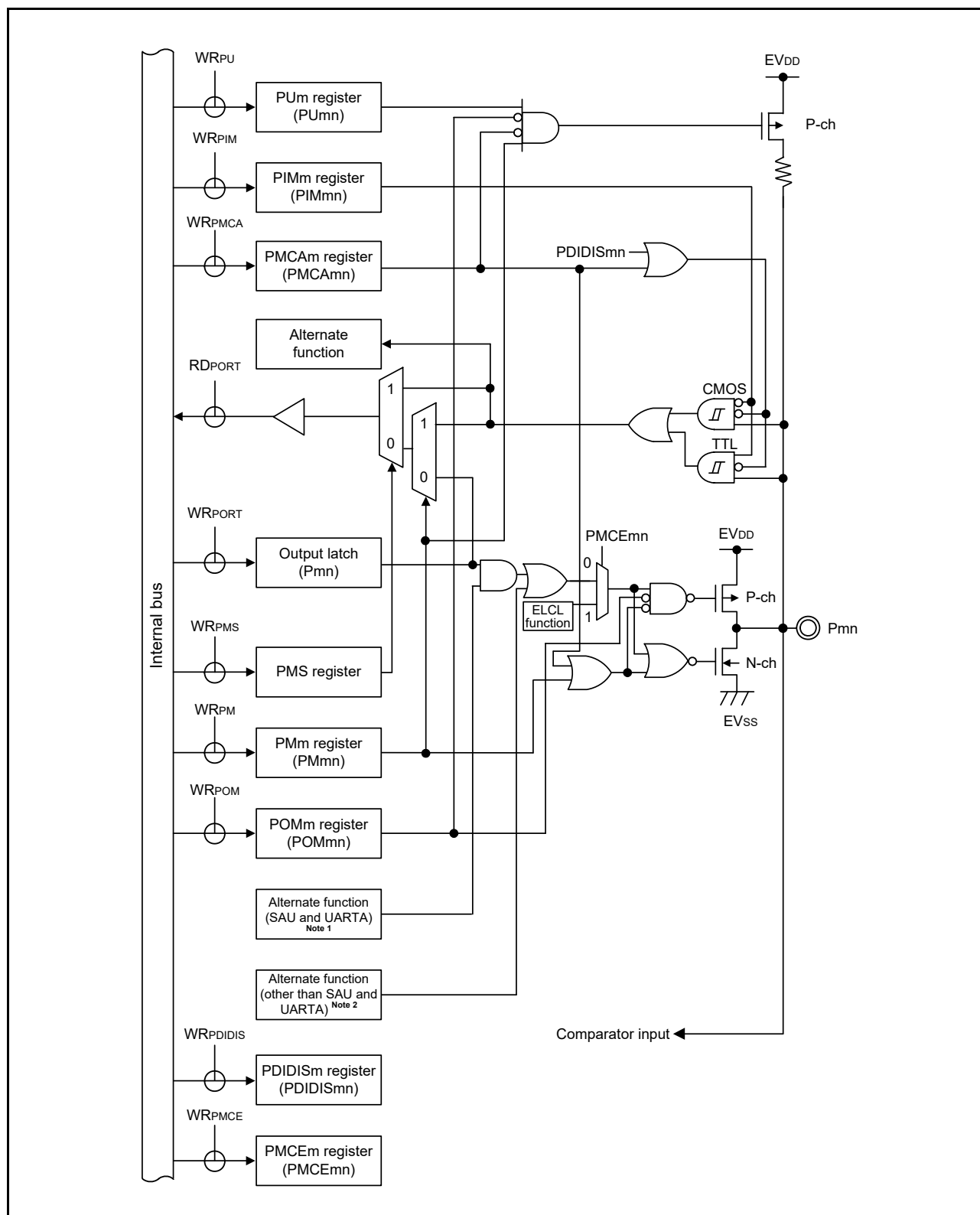
Figure 2 - 26 Pin Block Diagram for Pin Type 8-6-9
