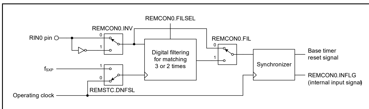
Figure 18 - 28 RIN0 Internal Input Signal Generation Configuration
