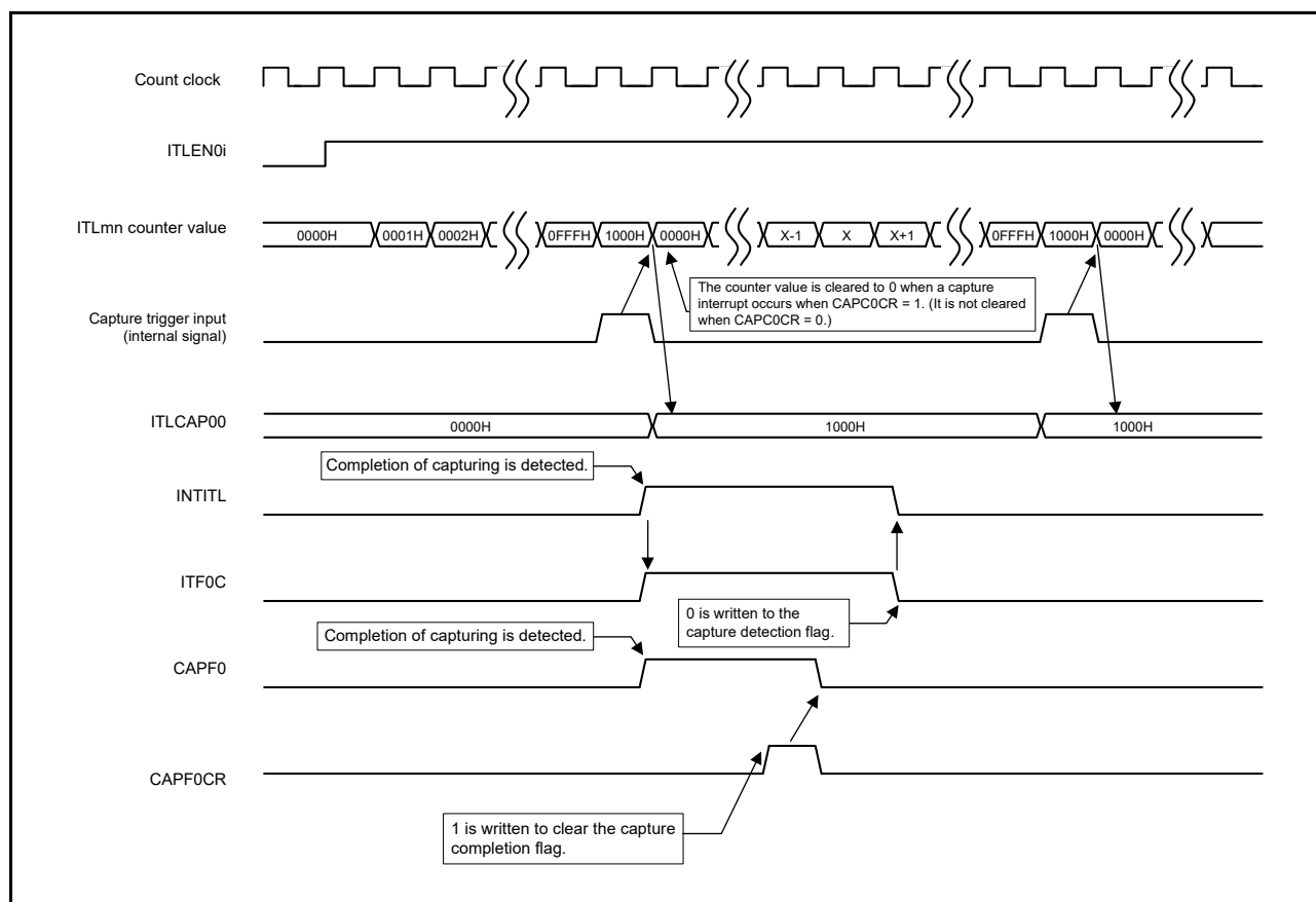
Figure 9 - 15 Example of Capture Operation
