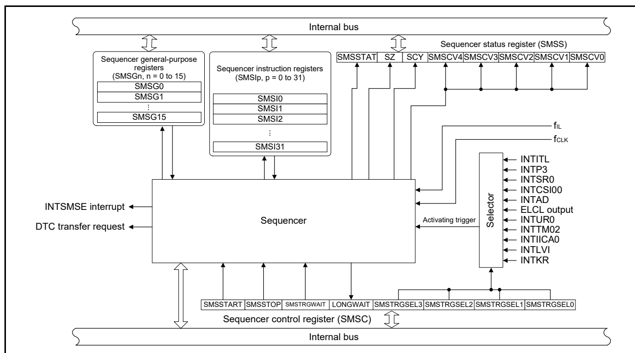
Figure 29 - 1 Block Diagram of the SNOOZE Mode Sequencer
