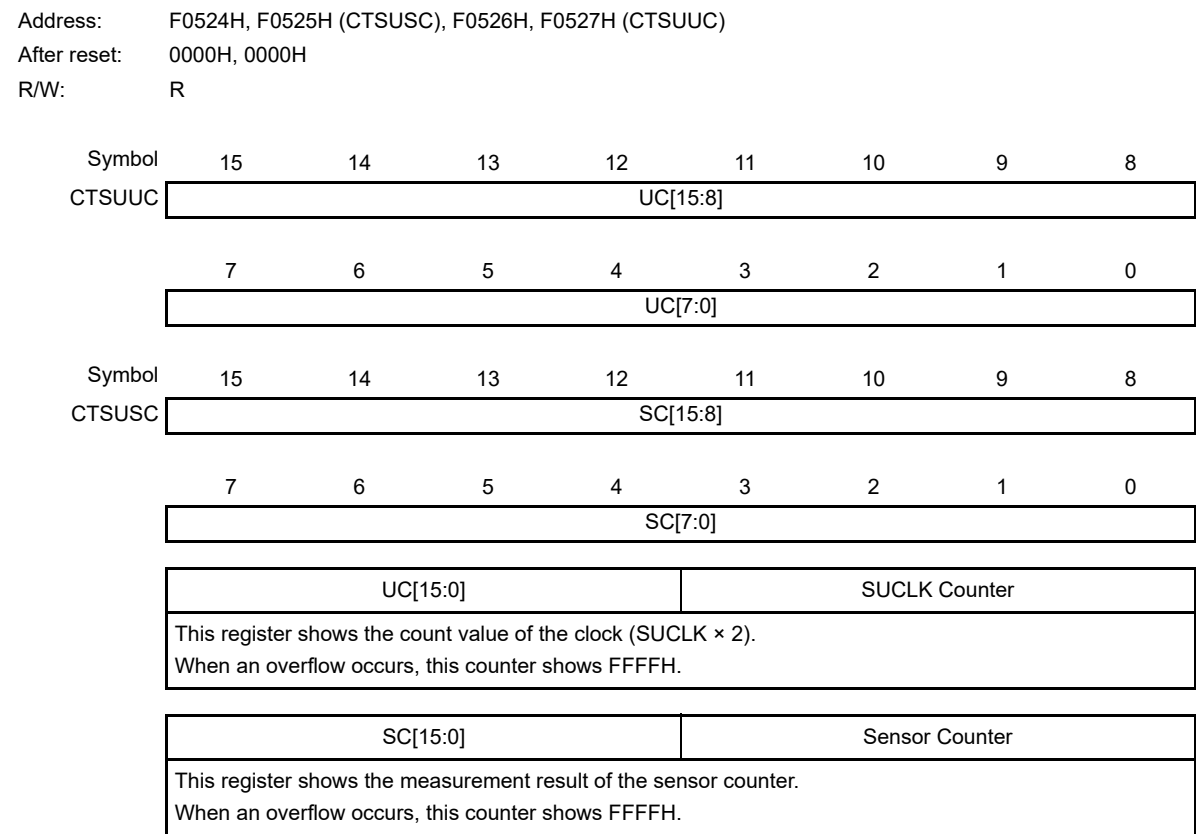
Figure 30 - 14 Format of CTSU Sensor Counter Registers L and H (CTSUSC, CTSUUC)
