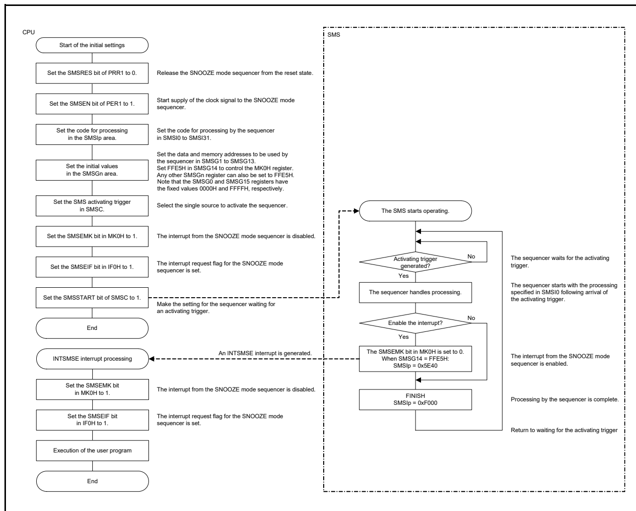
<R> Figure 29 - 11 Flow of Activating and Running the SNOOZE Mode Sequencer
