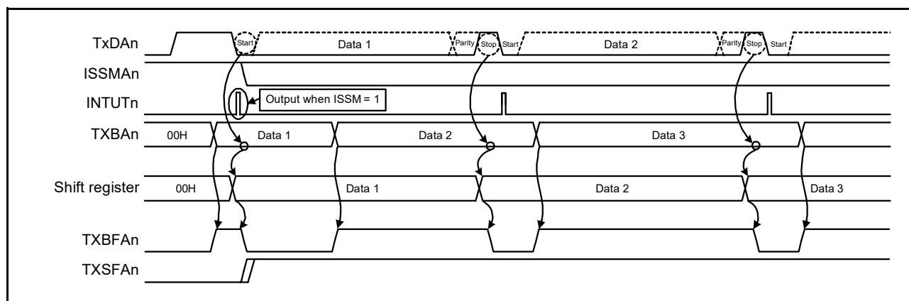
Figure 17 - 19 Timing Chart When Continuous Transmission Is Started
