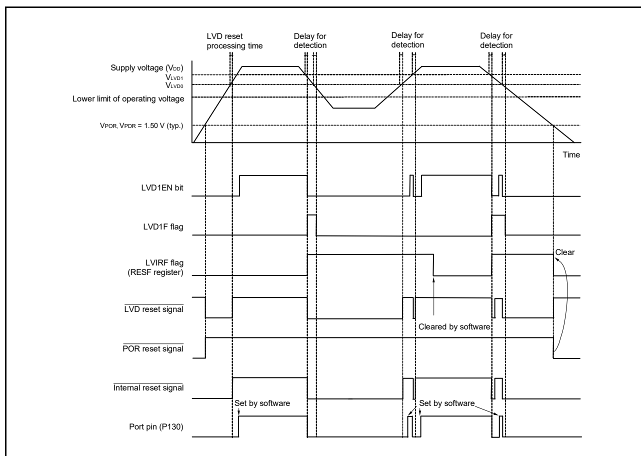
Figure 26 - 7 Timing of LVD1 Internal Reset Signal Generation
