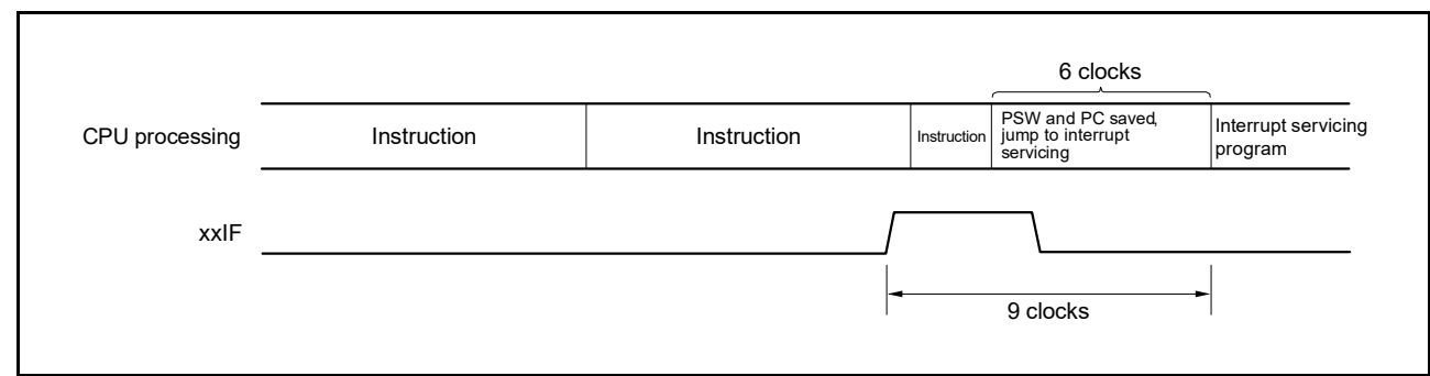
Figure 21 - 8 Interrupt Request Acknowledgment Timing (Minimum Time)
