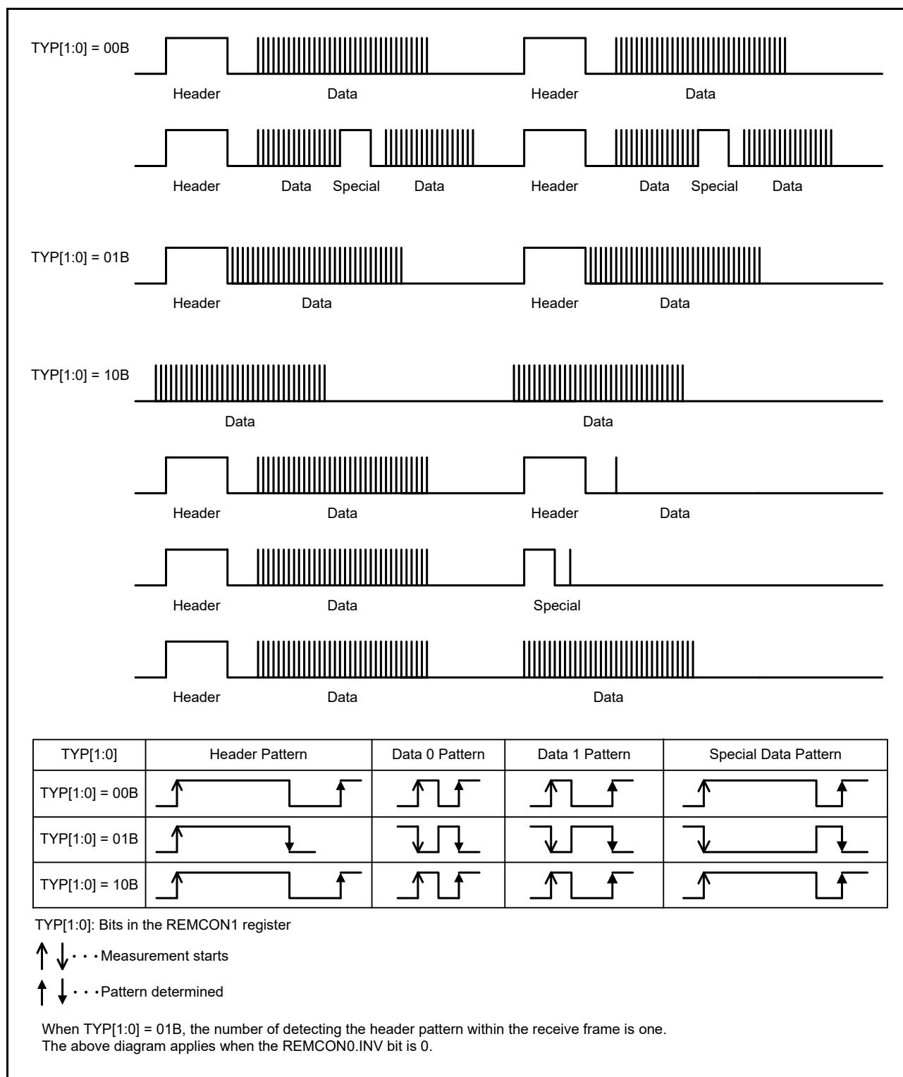
Figure 18 - 26 Example of Remote Control Signal Reception Waveform Captured by Setting REMCON1.TYP[1:0] Bits (REMCN0.INV = 0)
