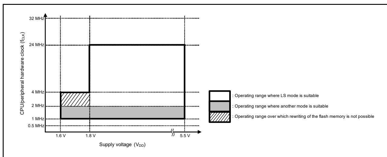
Figure 5 - 6 Operating Range in LS Mode
