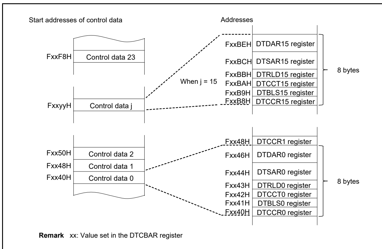
Figure 19 - 3 Control Data Allocation
