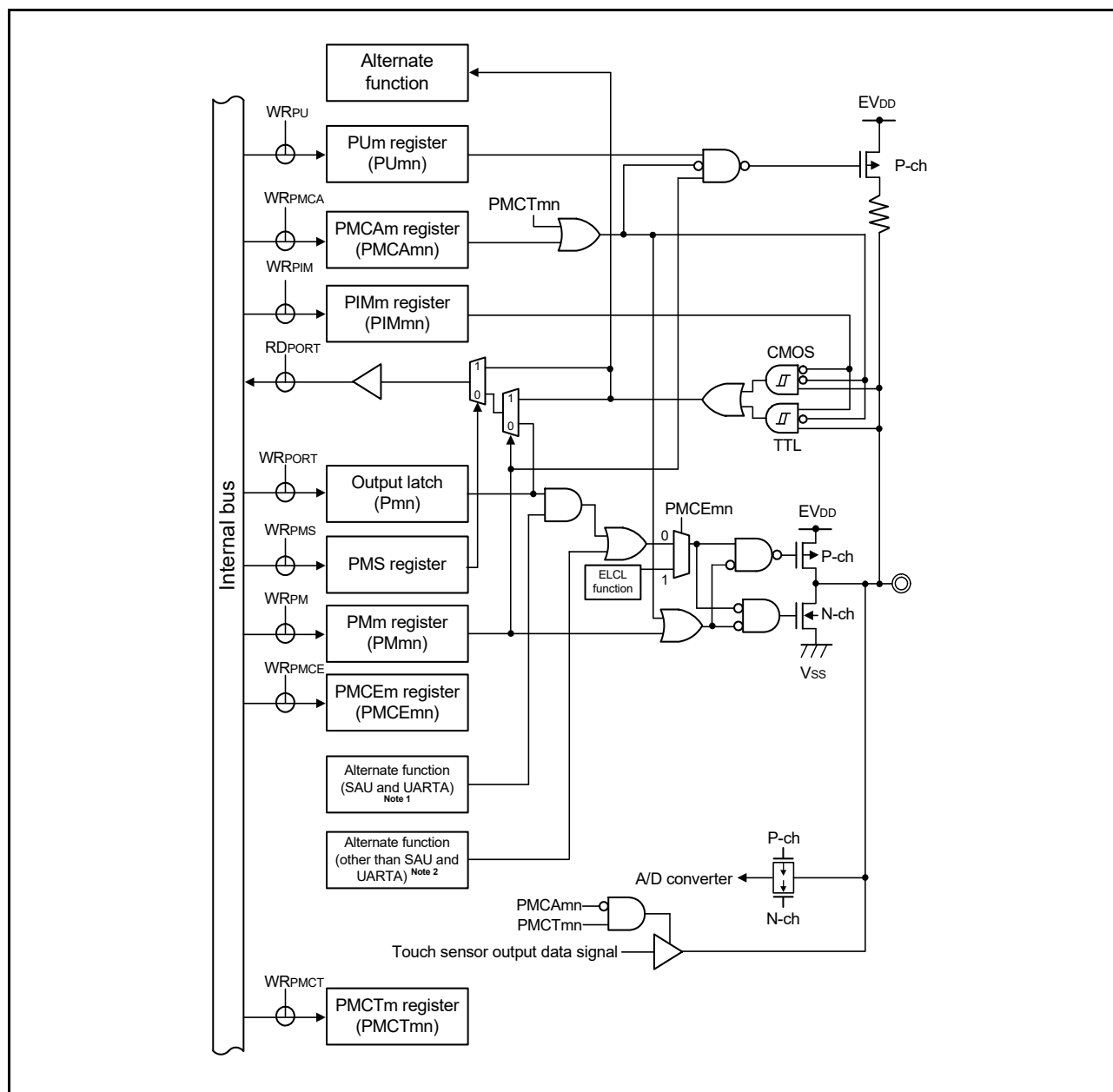
Figure 2 - 29 Pin Block Diagram for Pin Type 8-33-2
