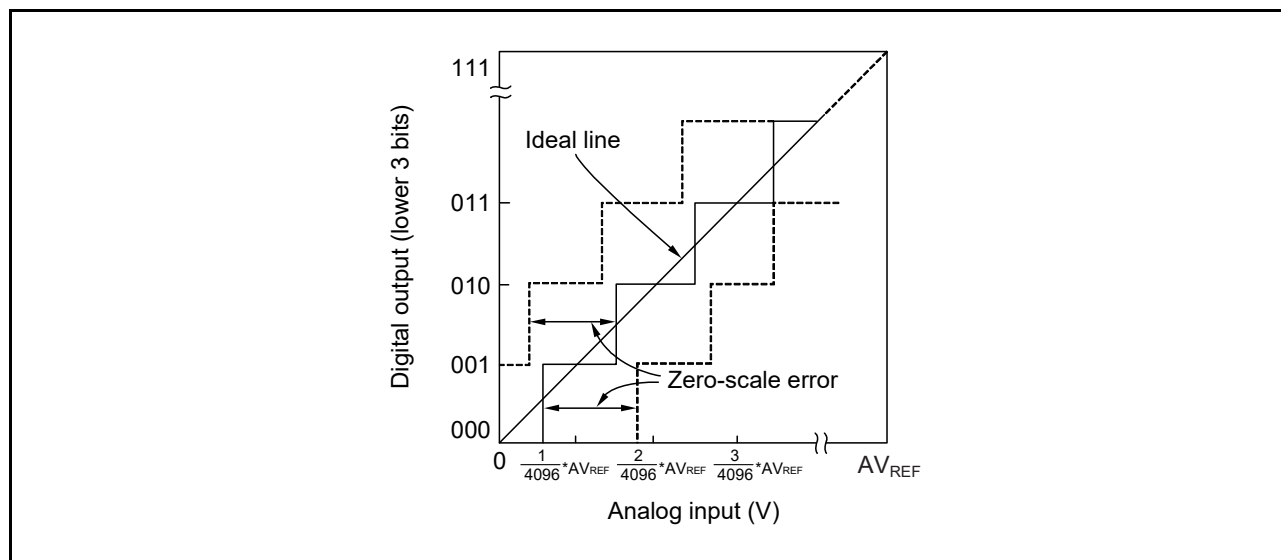
Figure 12 - 48 Zero-scale Error
