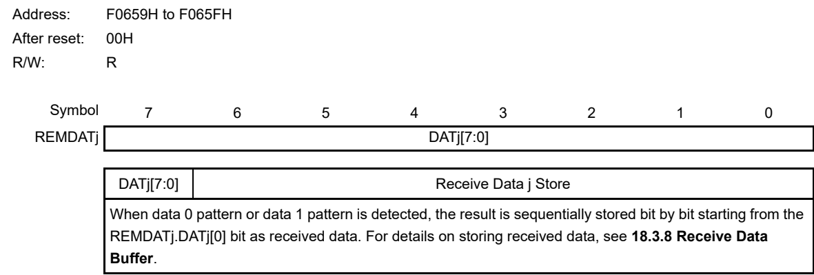
Figure 18 - 22 Format of Receive Data j Register (REMDATj)
