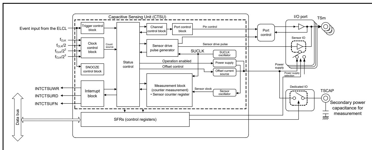
Figure 30 - 3 CTSU Block Diagram
