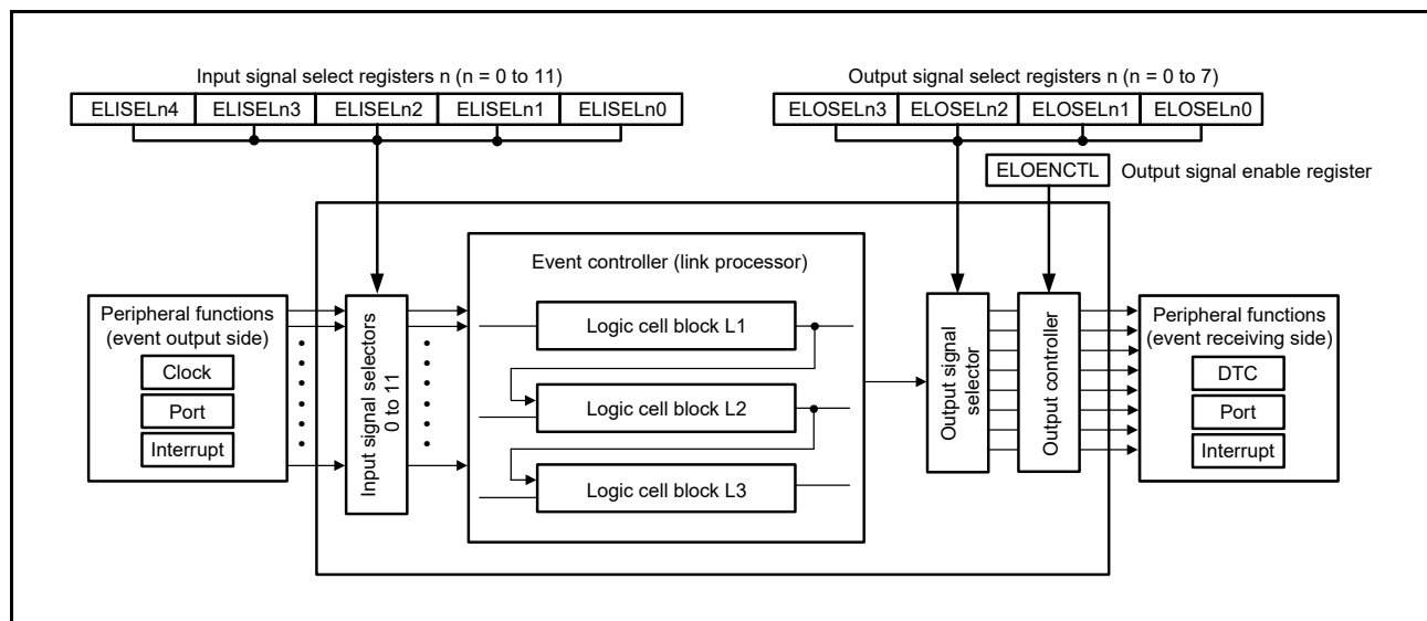
Figure 20 - 1 Block Diagram of ELCL
