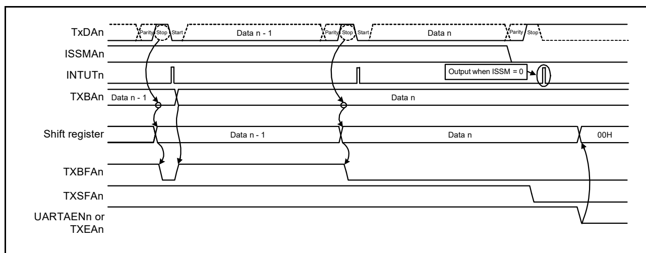
Figure 17 - 20 Timing Chart When Continuous Transmission Is Completed
