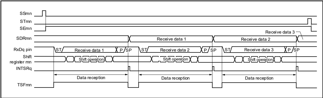
Figure 15 - 88 Timing Chart of UART Reception
