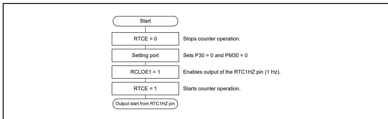
Figure 8 - 22 1 Hz Output Setting Procedure
