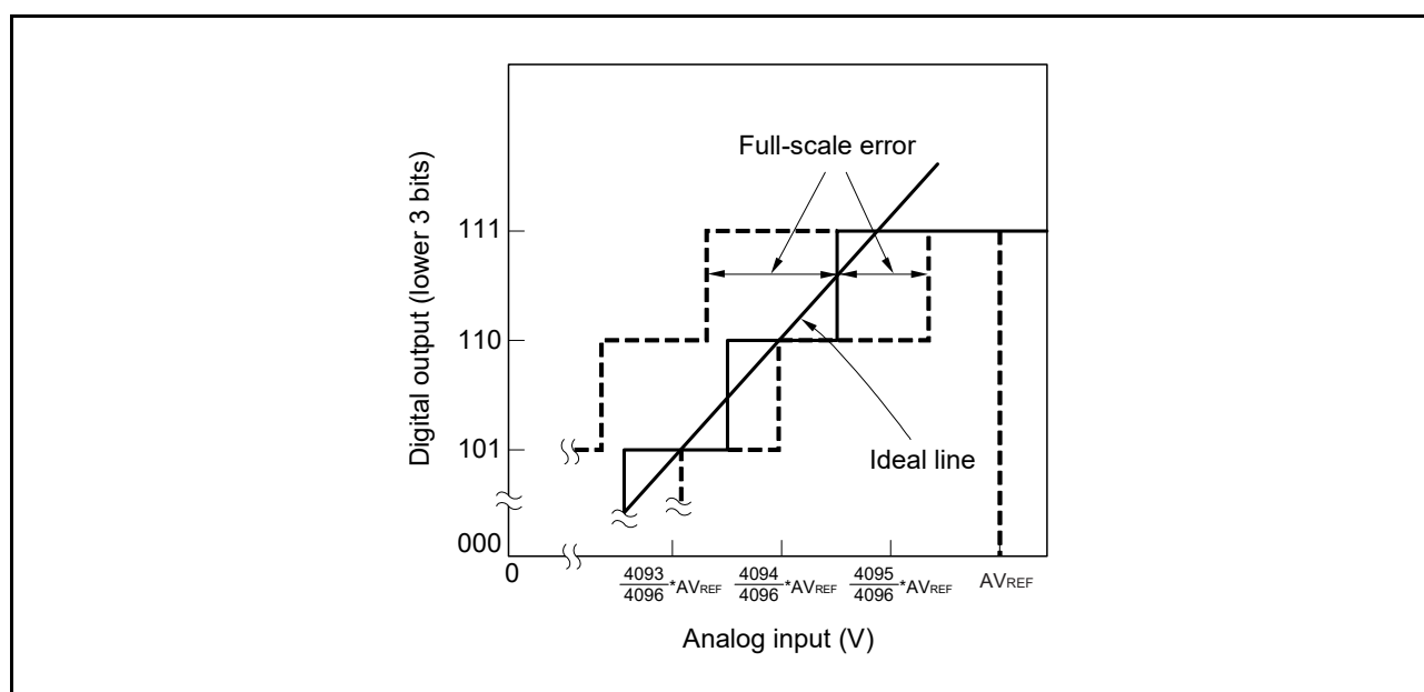
Figure 12 - 49 Full-scale Error
