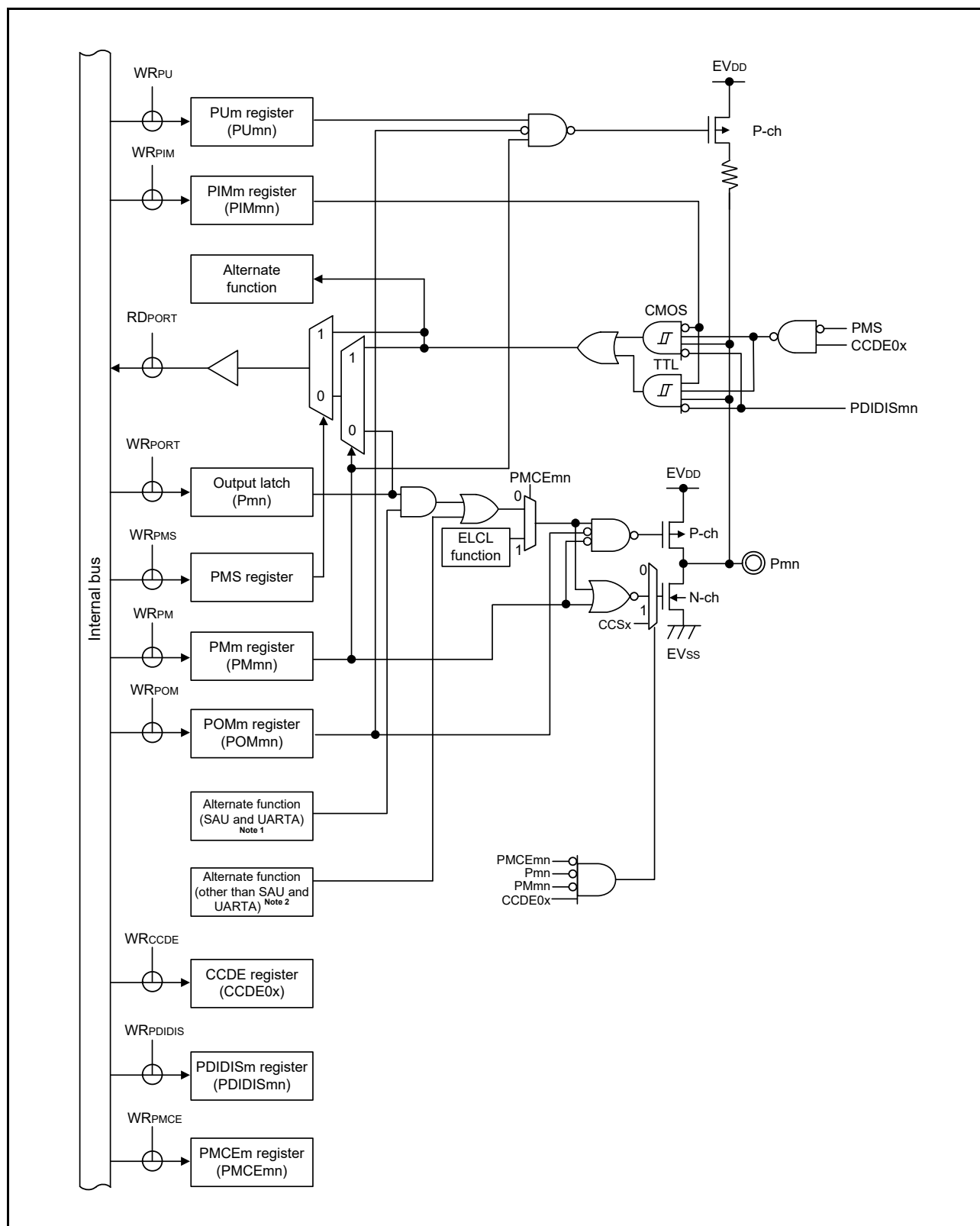
Figure 2 - 32 Pin Block Diagram for Pin Type 8-38-2
