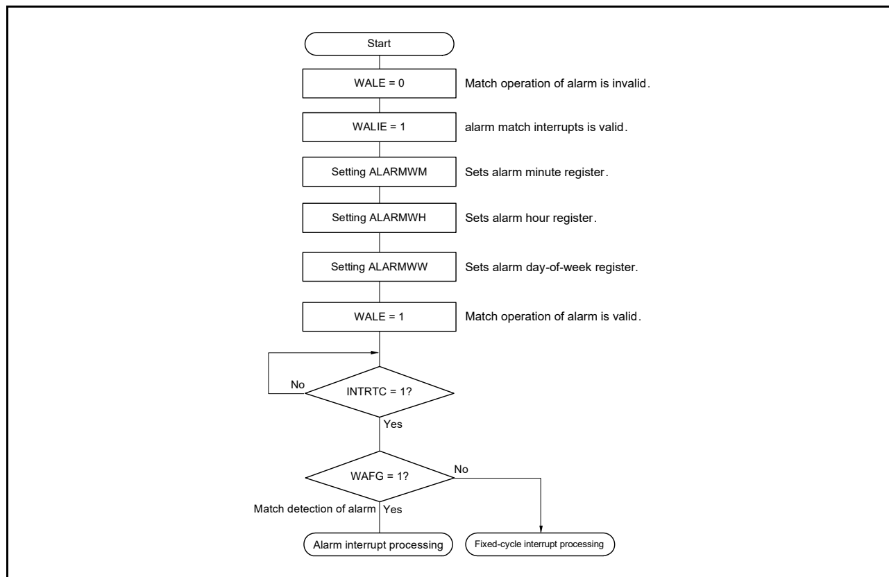
Figure 8 - 21 Alarm Processing Procedure
