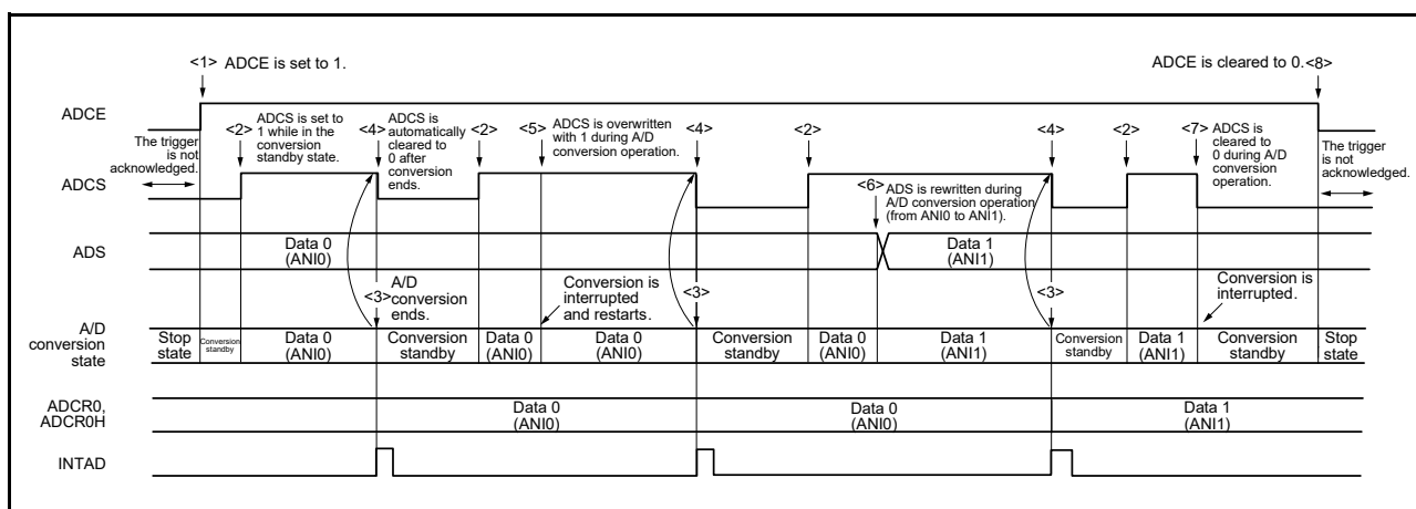
Figure 12 - 19 Example of Software Select No-wait Mode (Select Mode, One-shot Conversion Mode) Operation Timing
