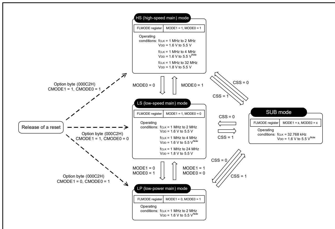
Figure 5 - 4 State Transitions between Flash Operation Modes
