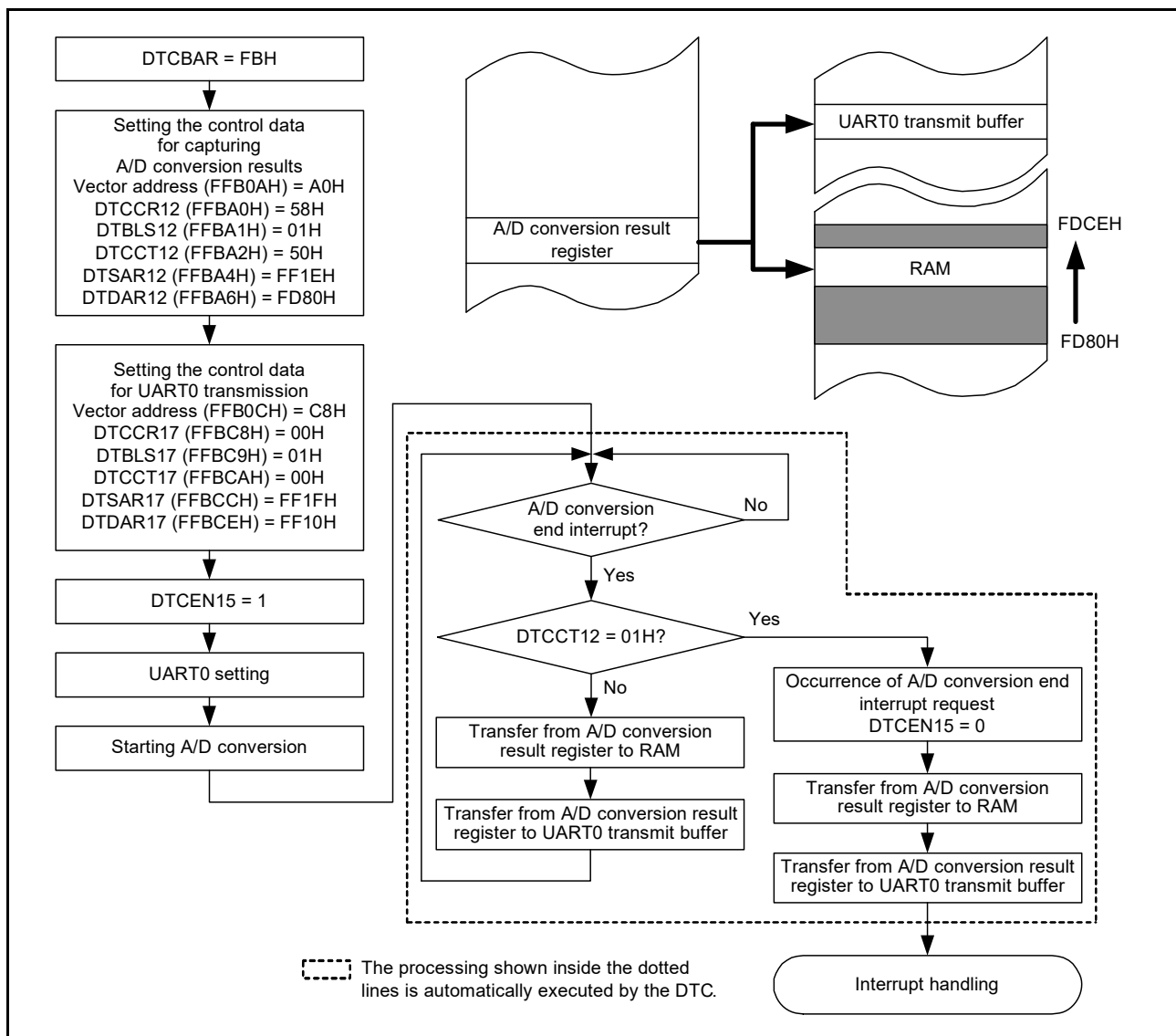
Figure 19 - 22 Example of Using Chain Transfers: Consecutively Capturing A/D Conversion Results and UART0 Transmission
