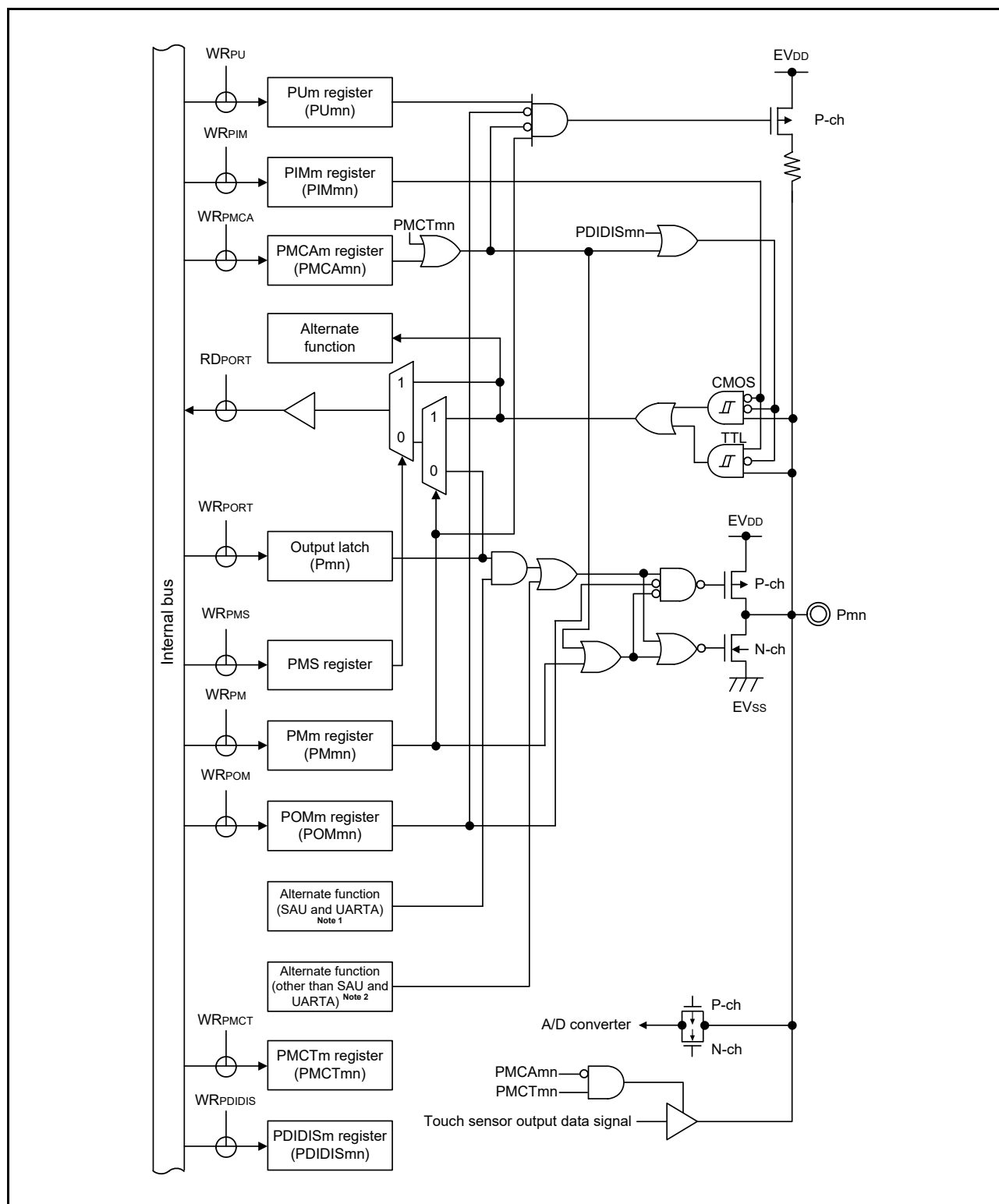
Figure 2 - 30 Pin Block Diagram for Pin Type 8-33-3
