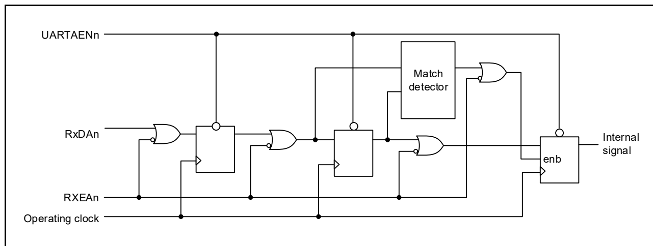
Figure 17 - 23 Noise Filter
