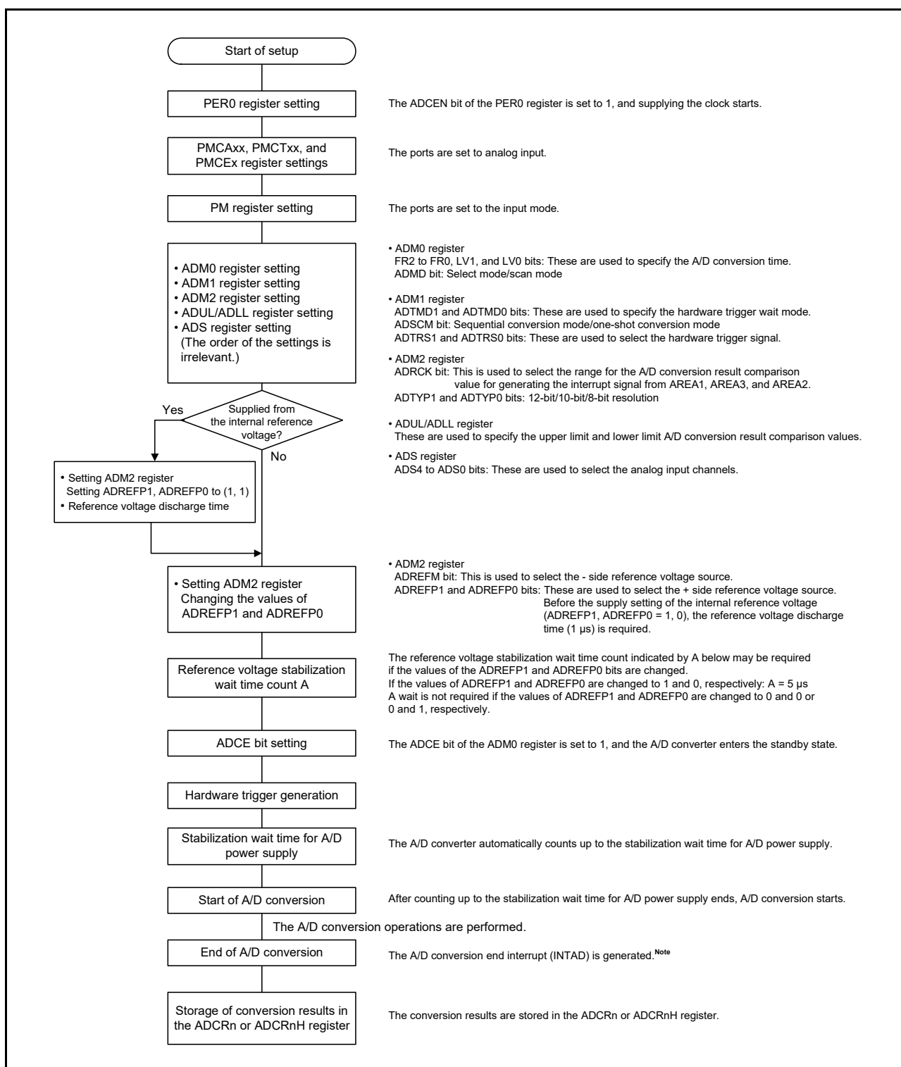
Figure 12 - 37 Setting up Hardware Trigger Wait Mode
