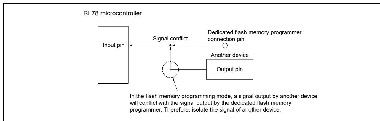
Figure 33 - 5 Signal Conflict ( \overline{\text{RESET}} Pin)
