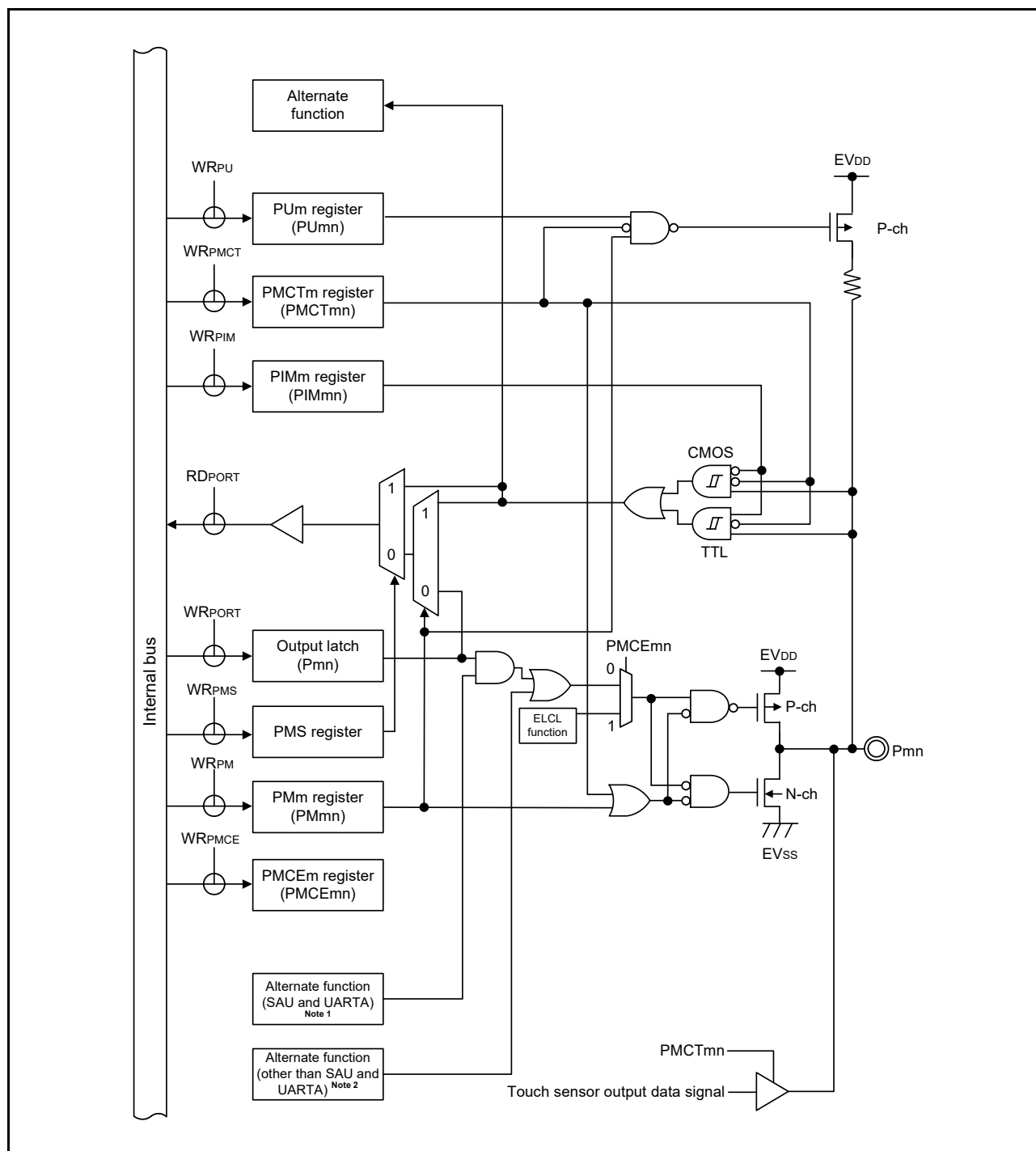
Figure 2 - 27 Pin Block Diagram for Pin Type 8-31-1
