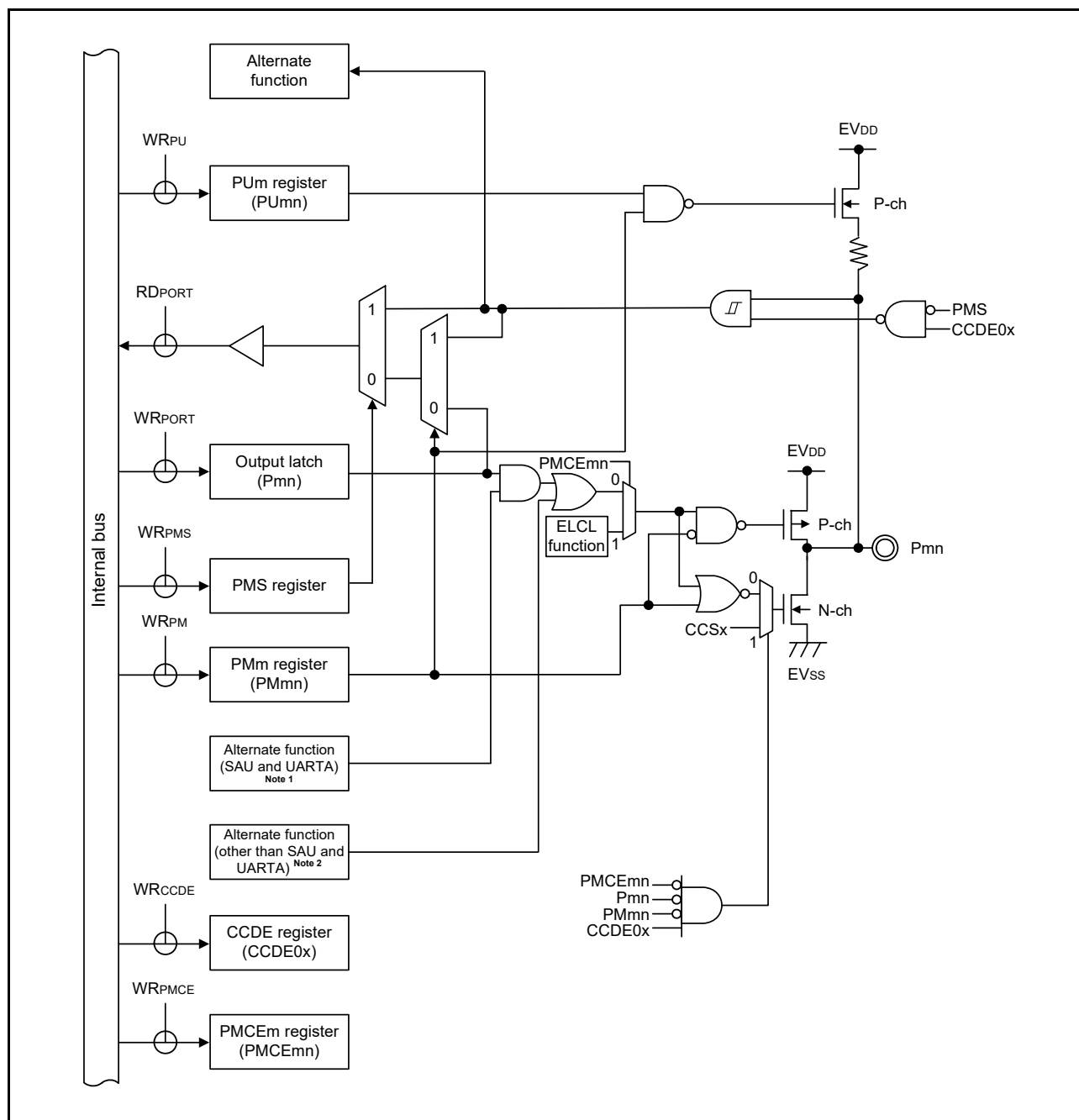
Figure 2 - 21 Pin Block Diagram for Pin Type 7-38-1
