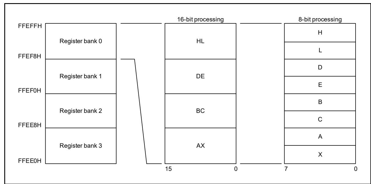
Figure 3 - 13 Configuration of General-Purpose Registers
