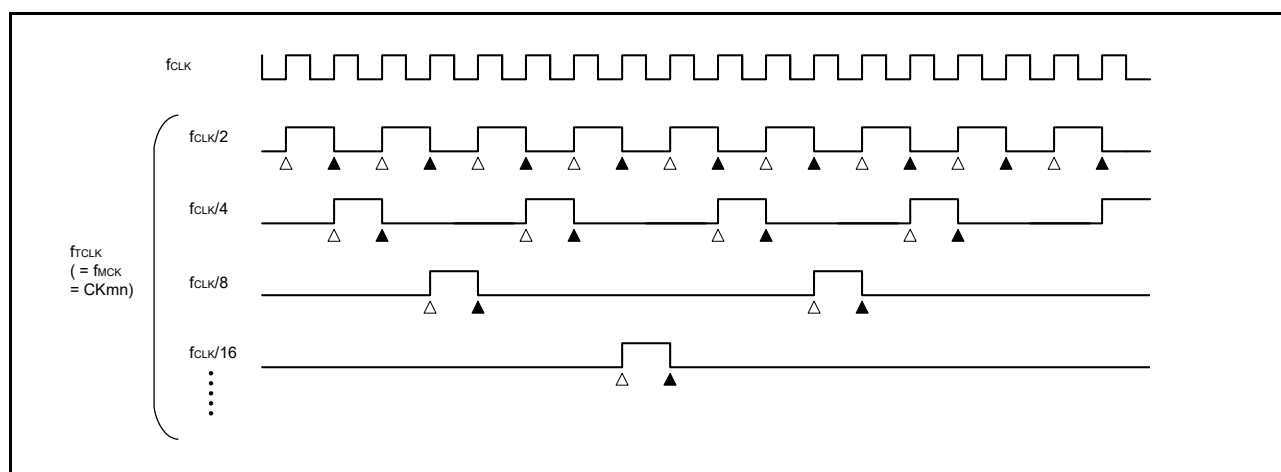
Figure 7 - 27 Timing of f CLK and Counter Clock (f CLK ) (When CCS mn = 0)
