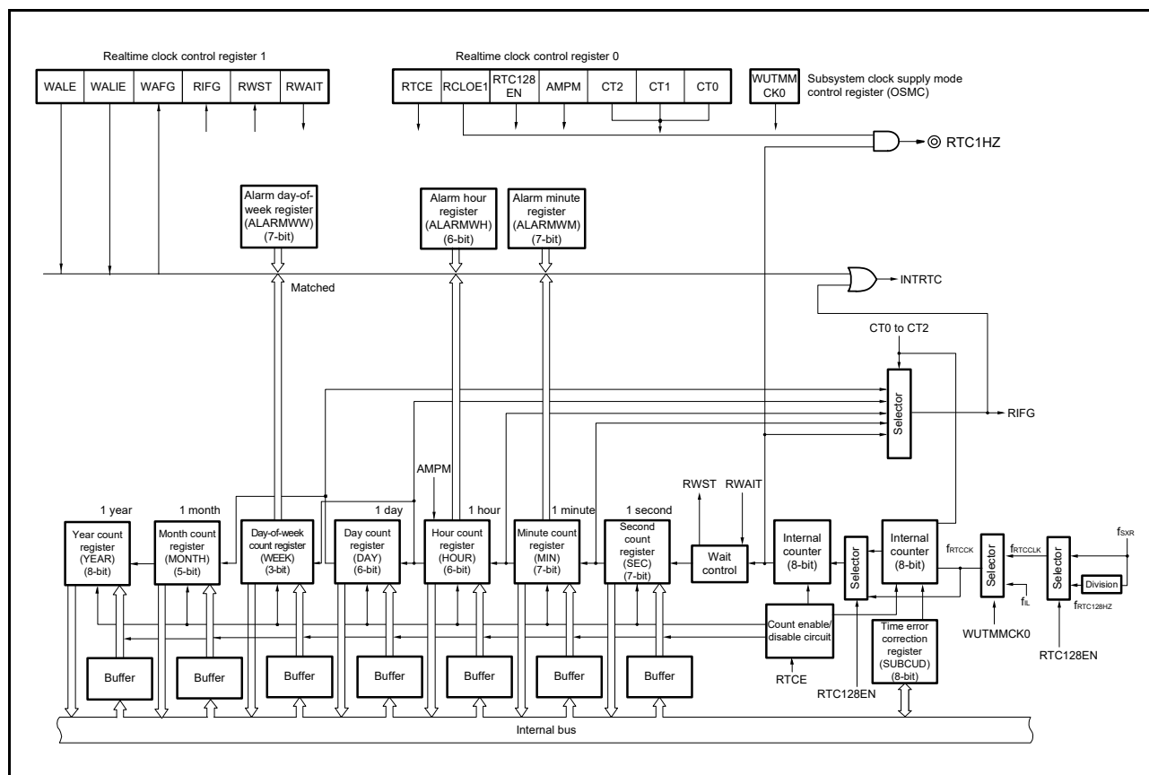
Figure 8 - 1 Block Diagram of the Realtime Clock
