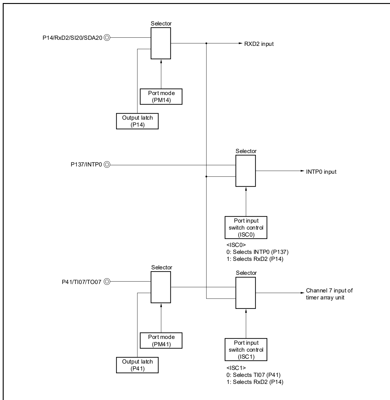
Figure 15 - 101 Port Configuration for Reception of LIN (44-, 48-, 52-, and 64-pin)
