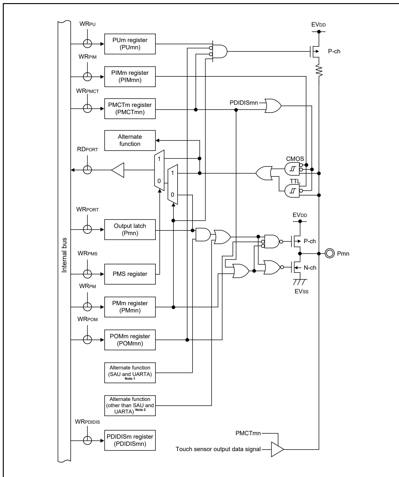
Figure 2 - 28 Pin Block Diagram for Pin Type 8-31-2
