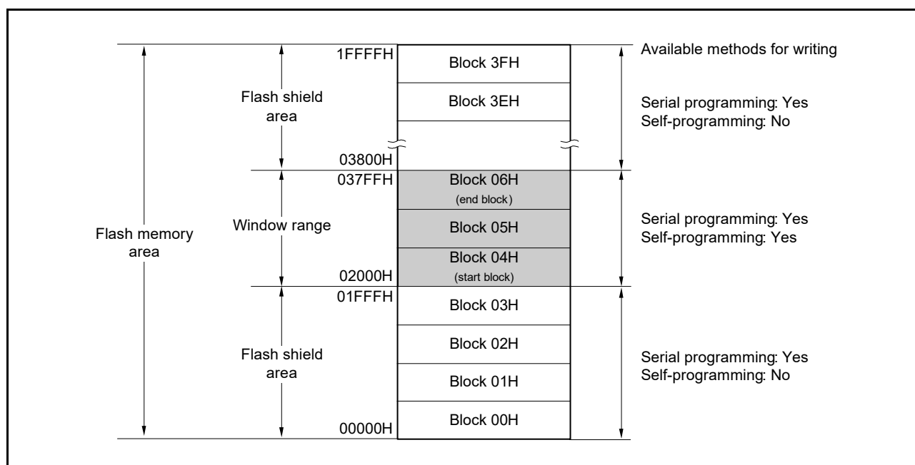
Figure 33 - 32 Flash Shield Window Setting Example (Target Devices: R7F100GLG, Start Block Number: 04H, End Block Number: 06H, FSWC: 1)
