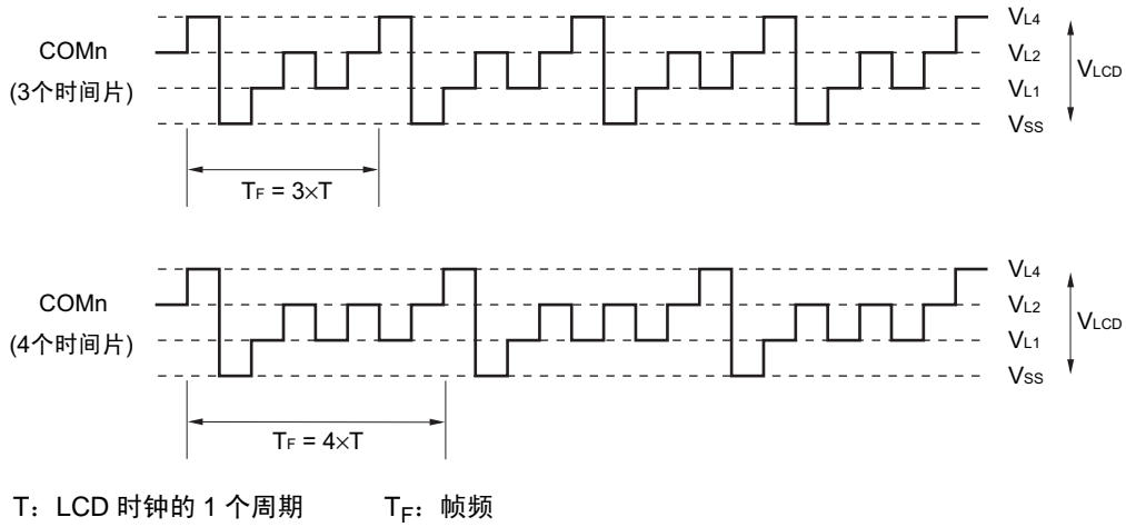
(c) 1/3 偏压法
